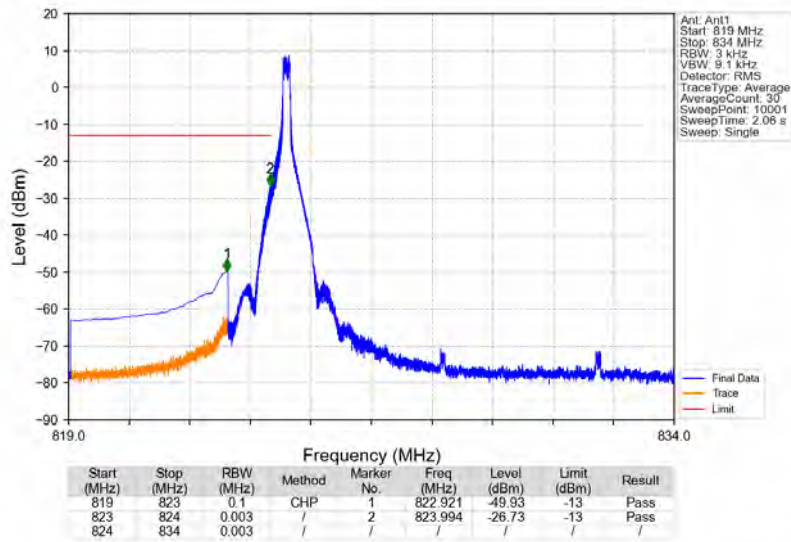
n5_15kHz_SISO_NTNV_10MHz_DFT-s-OFDM PI/2 BPSK_829MHz_Edge_1RB_Left
