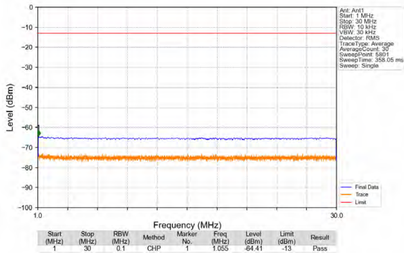
n5_15kHz_SISO_NTNV_10MHz_CP-OFDM QPSK_829MHz_Edge_1RB_Left
