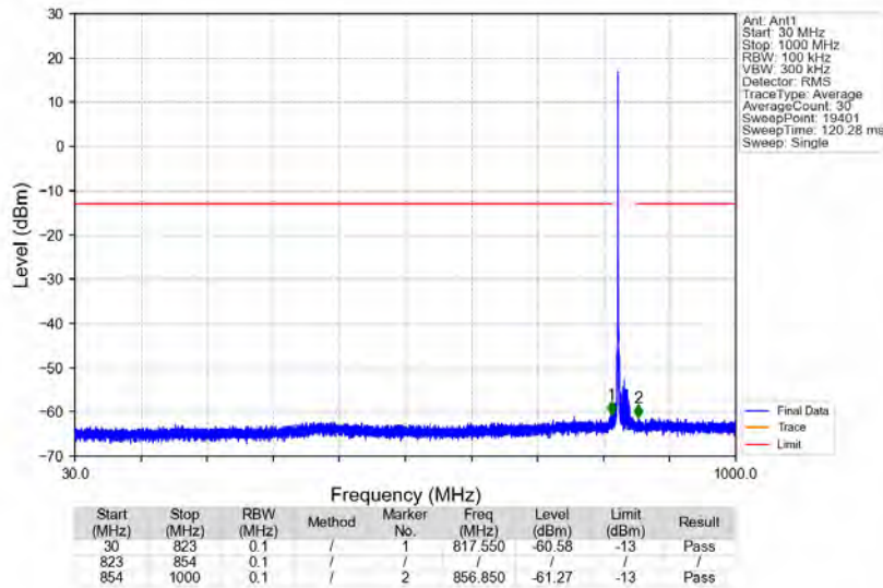
n5_15kHz_SISO_NTNV_20MHz_CP-OFDM QPSK_836.5MHz_Edge_1RB_Left
