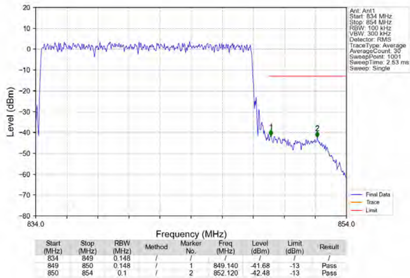
n5_15kHz_SISO_NTNV_15MHz_DFT-s-OFDM QPSK_841.5MHz_Outer_Full
