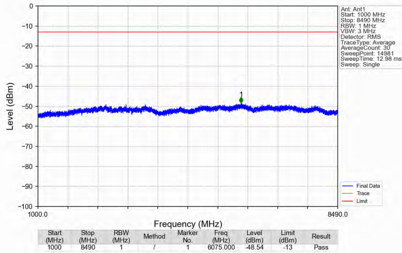
n5_15kHz_SISO_NTNV_5MHz_CP-OFDM QPSK_846.5MHz_Edge_1RB_Right
