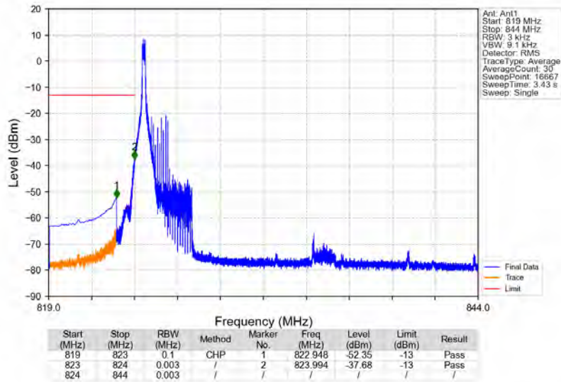
n5_15kHz_SISO_NTNV_20MHz_DFT-s-OFDM QPSK_834MHz_Edge_1RB_Left
