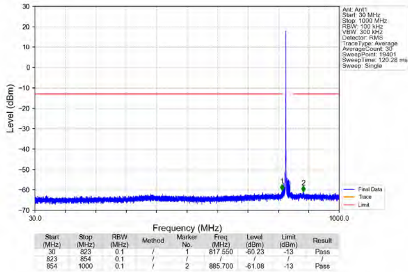
n5_15kHz_SISO_NTNV_15MHz_CP-OFDM QPSK_836.5MHz_Edge_1RB_Left
