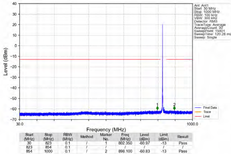
n5_15kHz_SISO_NTNV_10MHz_DFT-s-OFDM PI/2 BPSK_836.5MHz_Edge_1RB_Left
