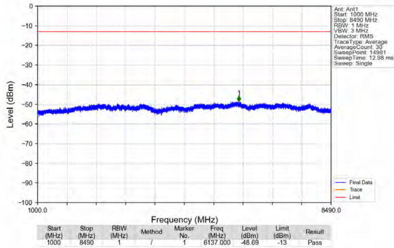
n5_15kHz_SISO_NTNV_10MHz_DFT-s-OFDM PI/2 BPSK_844MHz_Edge_1RB_Right
