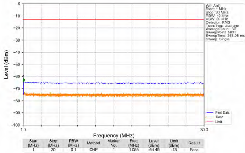
n5_15kHz_SISO_NTNV_15MHz_DFT-s-OFDM QPSK_831.5MHz_Edge_1RB_Left
