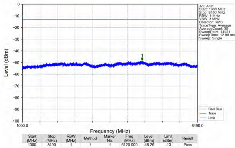
n5_15kHz_SISO_NTNV_20MHz_CP-OFDM QPSK_834MHz_Edge_1RB_Left
