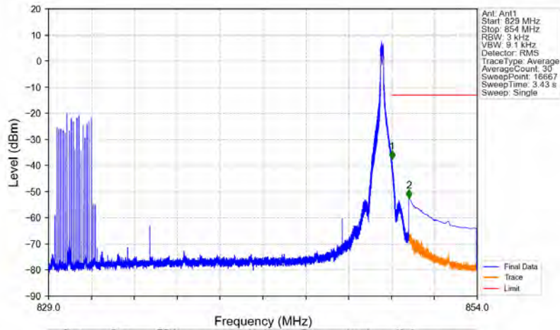
n5_15kHz_SISO_NTNV_20MHz_DFT-s-OFDM QPSK_839MHz_Edge_1RB_Right
