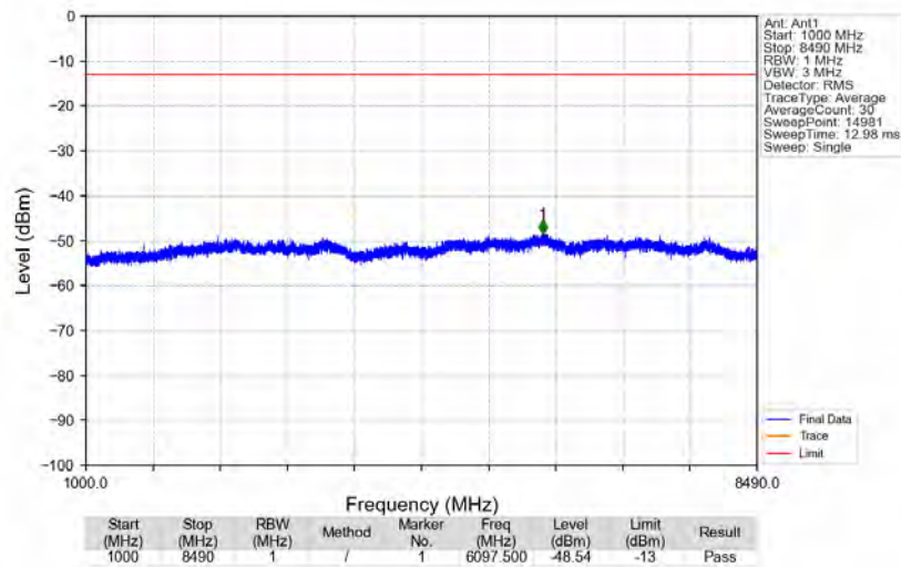
n5_15kHz_SISO_NTNV_20MHz_DFT-s-OFDM_QPSK_834MHz_Edge_1RB_Left
