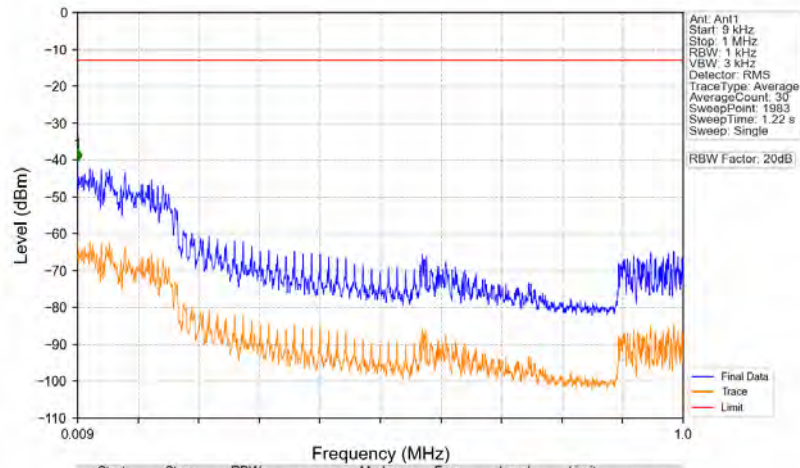
n5_15kHz_SISO_NTNV_10MHz_CP-OFDM QPSK_829MHz_Edge_1RB_Left
