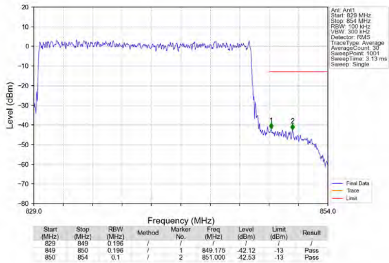
n5_15kHz_SISO_NTNV_20MHz_DFT-s-OFDM PI/2 BPSK_839MHz_Outer_Full
