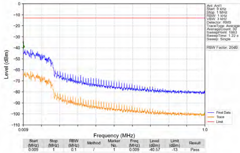
n5_15kHz_SISO_NTNV_15MHz_CP-OFDM QPSK_836.5MHz_Edge_1RB_Left
