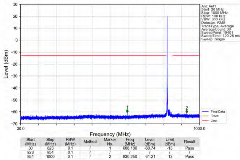
n5_15kHz_SISO_NTNV_20MHz_DFT-s-OFDM_QPSK_834MHz_Edge_1RB_Left
