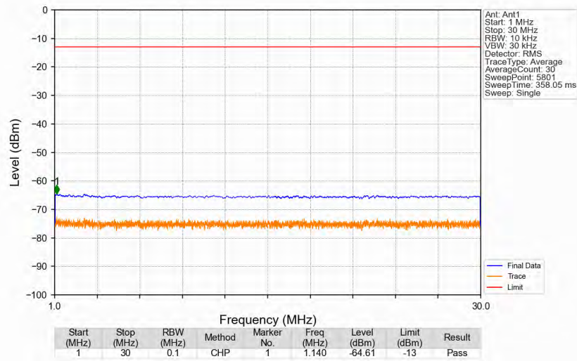
n5_15kHz_SISO_NTNV_20MHz_CP-OFDM QPSK_834MHz_Edge_1RB_Left
