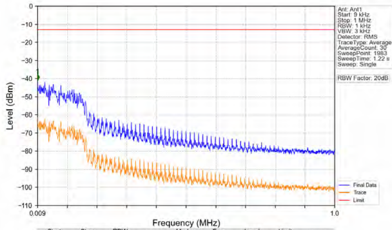
n5_15kHz_SISO_NTNV_20MHz_CP-OFDM QPSK_839MHz_Edge_1RB_Right
