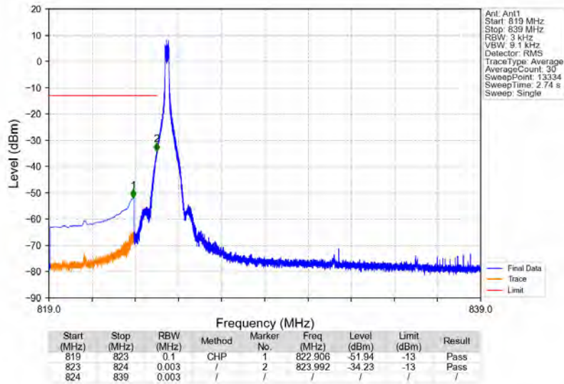
n5_15kHz_SISO_NTNV_15MHz_DFT-s-OFDM QPSK_831.5MHz_Edge_1RB_Left
