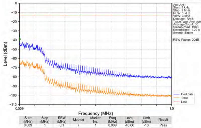
n5_15kHz_SISO_NTNV_20MHz_CP-OFDM QPSK_836.5MHz_Edge_1RB_Left
