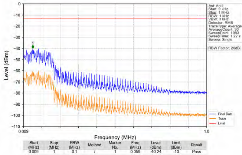
n5_15kHz_SISO_NTNV_10MHz_DFT-s-OFDM QPSK_836.5MHz_Edge_1RB_Left
