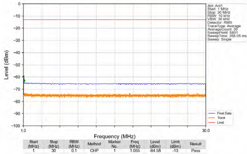
n5_15kHz_SISO_NTNV_20MHz_DFT-s-OFDM QPSK_836.5MHz_Edge_1RB_Left
