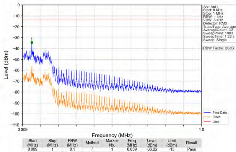
n5_15kHz_SISO_NTNV_20MHz_DFT-s-OFDM PI/2 BPSK_834MHz_Edge_1RB_Left
