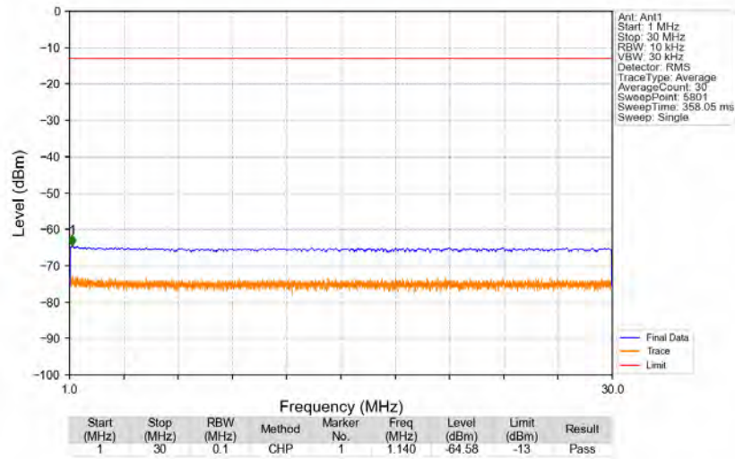
n5_15kHz_SISO_NTNV_20MHz_DFT-s-OFDM_QPSK_834MHz_Edge_1RB_Left
