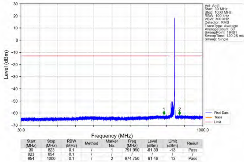
n5_15kHz_SISO_NTNV_20MHz_CP-OFDM QPSK_839MHz_Edge_1RB_Right
