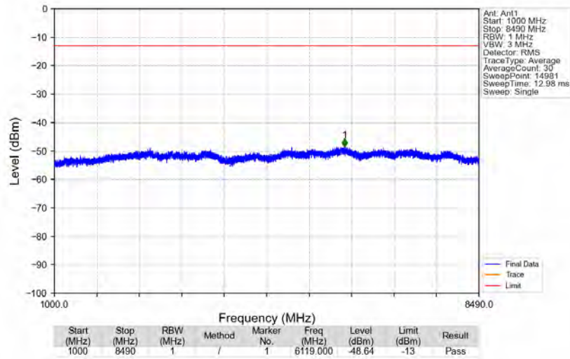
n5_15kHz_SISO_NTNV_10MHz_CP-OFDM QPSK_844MHz_Edge_1RB_Right
