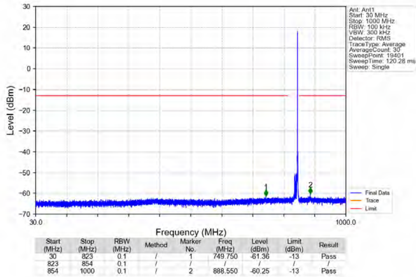
n5_15kHz_SISO_NTNV_10MHz_CP-OFDM QPSK_844MHz_Edge_1RB_Right
