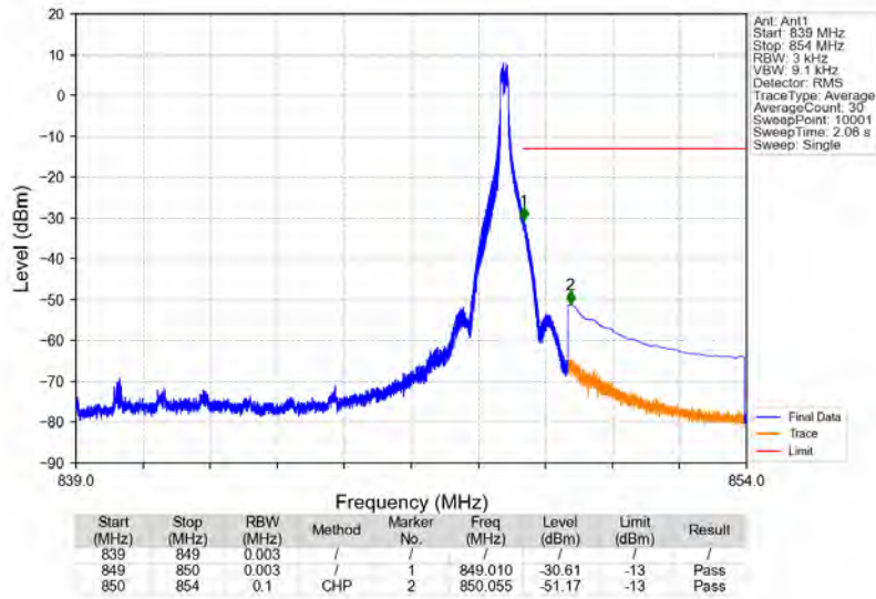
n5_15kHz_SISO_NTNV_10MHz_DFT-s-OFDM QPSK_844MHz_Edge_1RB_Right
