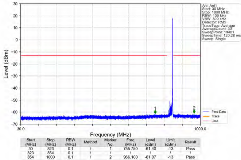
n5_15kHz_SISO_NTNV_15MHz_CP-OFDM QPSK_841.5MHz_Edge_1RB_Right
