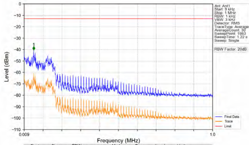
n5_15kHz_SISO_NTNV_10MHz_DFT-s-OFDM PI/2 BPSK_844MHz_Edge_1RB_Right
