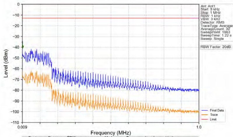
n5_15kHz_SISO_NTNV_20MHz_DFT-s-OFDM QPSK_839MHz_Edge_1RB_Right
