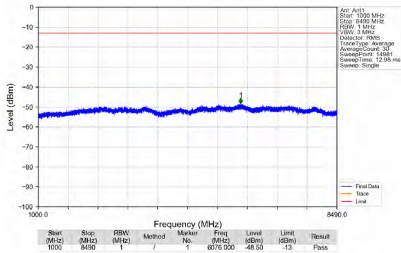
n5_15kHz_SISO_NTNV_15MHz_CP-OFDM QPSK_841.5MHz_Edge_1RB_Right
