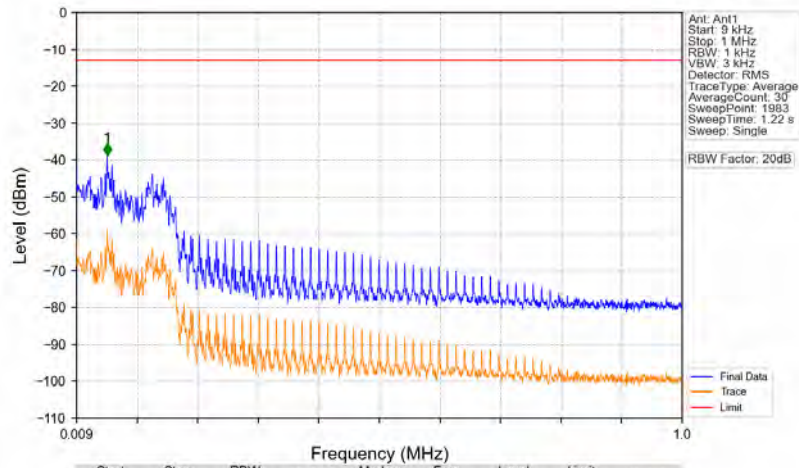
n5_15kHz_SISO_NTNV_20MHz_DFT-s-OFDM PI/2 BPSK_839MHz_Edge_1RB_Right
