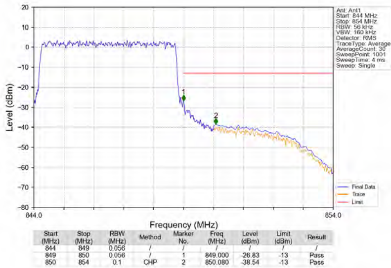
n5_15kHz_SISO_NTNV_5MHz_CP-OFDM QPSK_846.5MHz_Outer_Full
