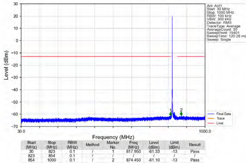
n5_15kHz_SISO_NTNV_20MHz_DFT-s-OFDM QPSK_836.5MHz_Edge_1RB_Left
