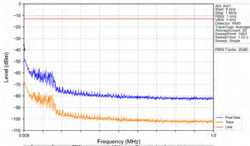
n5_15kHz_SISO_NTNV_15MHz_DFT-s-OFDM QPSK_841.5MHz_Edge_1RB_Right
