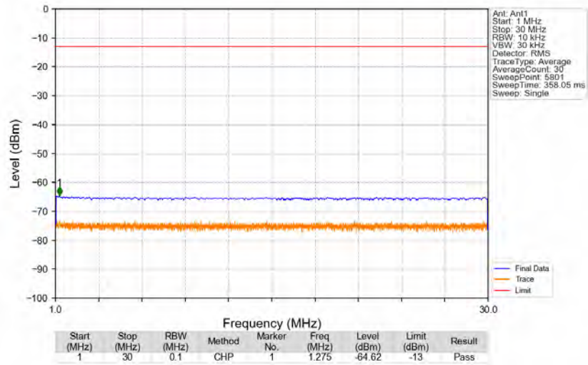
n5_15kHz_SISO_NTNV_15MHz_CP-OFDM QPSK_831.5MHz_Edge_1RB_Left
