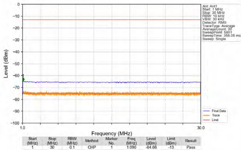
n5_15kHz_SISO_NTNV_15MHz_DFT-s-OFDM QPSK_841.5MHz_Edge_1RB_Right
