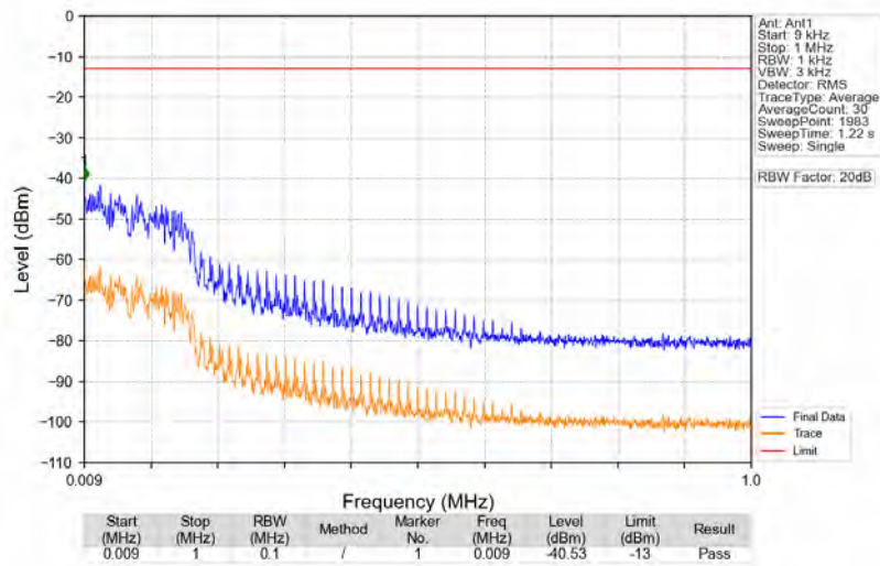
n5_15kHz_SISO_NTNV_5MHz_CP-OFDM QPSK_846.5MHz_Edge_1RB_Right
