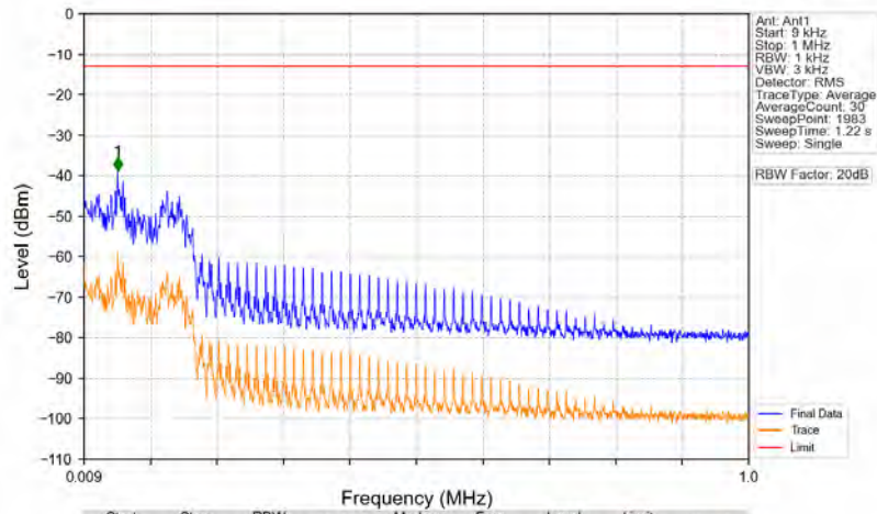
n5_15kHz_SISO_NTNV_15MHz_DFT-s-OFDM PI/2 BPSK_841.5MHz_Edge_1RB_Right
