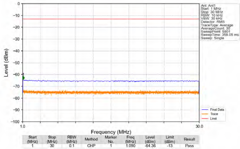
n5_15kHz_SISO_NTNV_10MHz_DFT-s-OFDM QPSK_829MHz_Edge_1RB_Left
