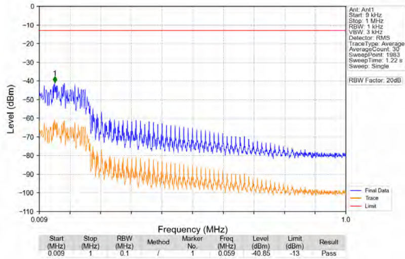
n5_15kHz_SISO_NTNV_20MHz_DFT-s-OFDM QPSK_836.5MHz_Edge_1RB_Left
