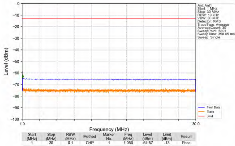
n5_15kHz_SISO_NTNV_20MHz_DFT-s-OFDM QPSK_839MHz_Edge_1RB_Right
