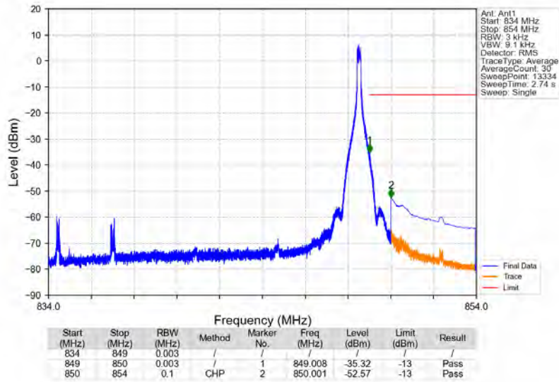
n5_15kHz_SISO_NTNV_15MHz_CP-OFDM QPSK_841.5MHz_Edge_1RB_Right
