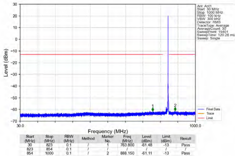
n5_15kHz_SISO_NTNV_10MHz_DFT-s-OFDM PI/2 BPSK_844MHz_Edge_1RB_Right
