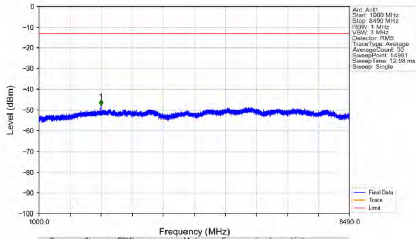
n5_15kHz_SISO_NTNV_10MHz_DFT-s-OFDM QPSK_836.5MHz_Edge_1RB_Left
