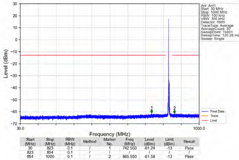
n5_15kHz_SISO_NTNV_5MHz_CP-OFDM QPSK_836.5MHz_Edge_1RB_Left
