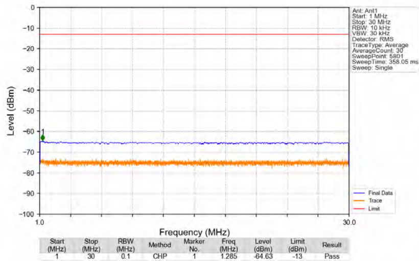
n5_15kHz_SISO_NTNV_20MHz_CP-OFDM QPSK_836.5MHz_Edge_1RB_Left
