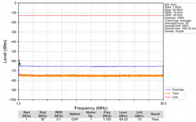
n5_15kHz_SISO_NTNV_10MHz_DFT-s-OFDM QPSK_836.5MHz_Edge_1RB_Left
