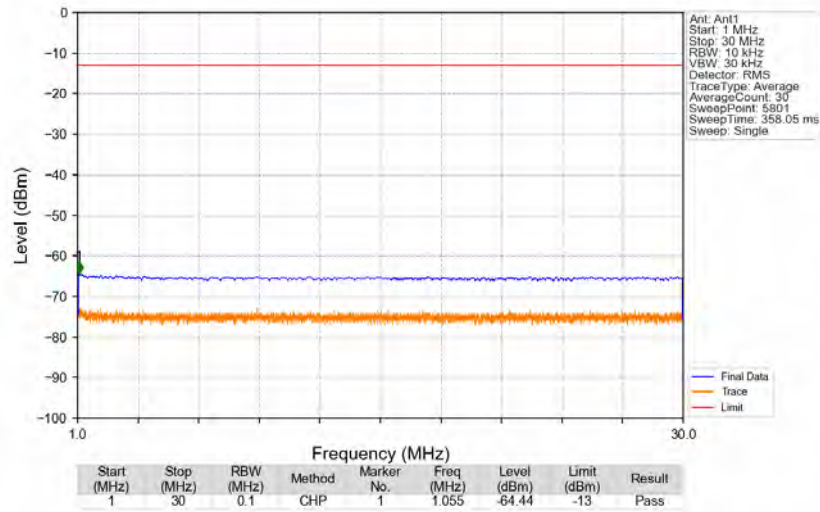
n5_15kHz_SISO_NTNV_10MHz_DFT-s-OFDM QPSK_844MHz_Edge_1RB_Right
