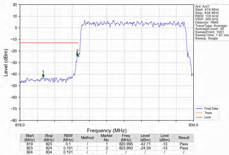
n5_15kHz_SISO_NTNV_10MHz_DFT-s-OFDM PI/2 BPSK_829MHz_Outer_Full
