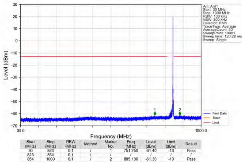
n5_15kHz_SISO_NTNV_15MHz_DFT-s-OFDM QPSK_841.5MHz_Edge_1RB_Right
