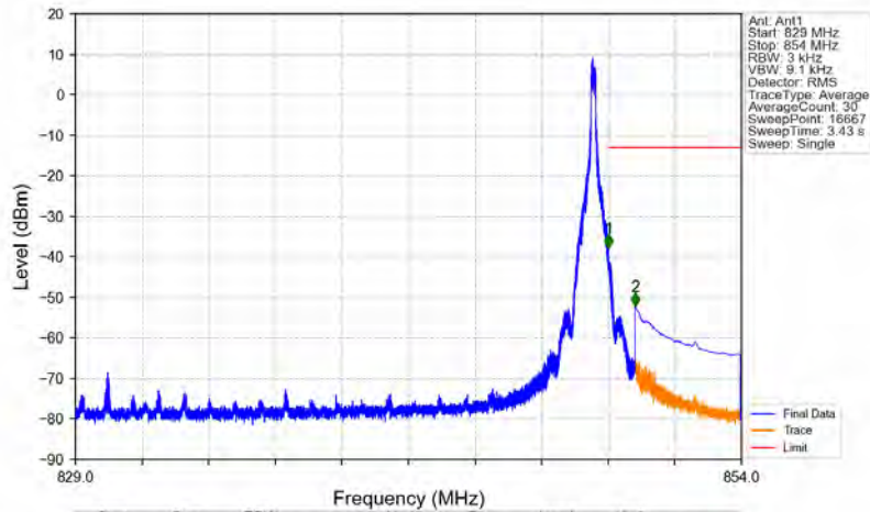
n5_15kHz_SISO_NTNV_20MHz_DFT-s-OFDM PI/2 BPSK_839MHz_Edge_1RB_Right
