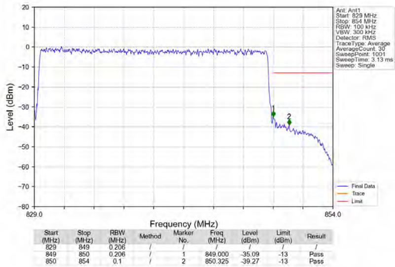
n5_15kHz_SISO_NTNV_20MHz_CP-OFDM QPSK_839MHz_Outer_Full
