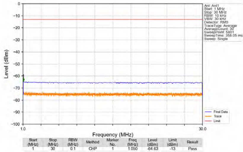
n5_15kHz_SISO_NTNV_10MHz_CP-OFDM QPSK_844MHz_Edge_1RB_Right
