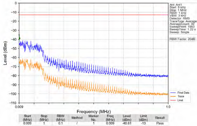
n5_15kHz_SISO_NTNV_10MHz_CP-OFDM QPSK_836.5MHz_Edge_1RB_Left
