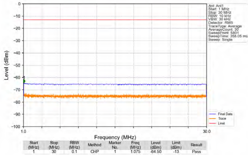
n5_15kHz_SISO_NTNV_20MHz_CP-OFDM QPSK_839MHz_Edge_1RB_Right
