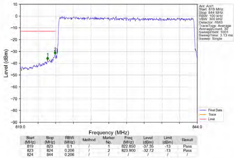
n5_15kHz_SISO_NTNV_20MHz_CP-OFDM QPSK_834MHz_Outer_Full
