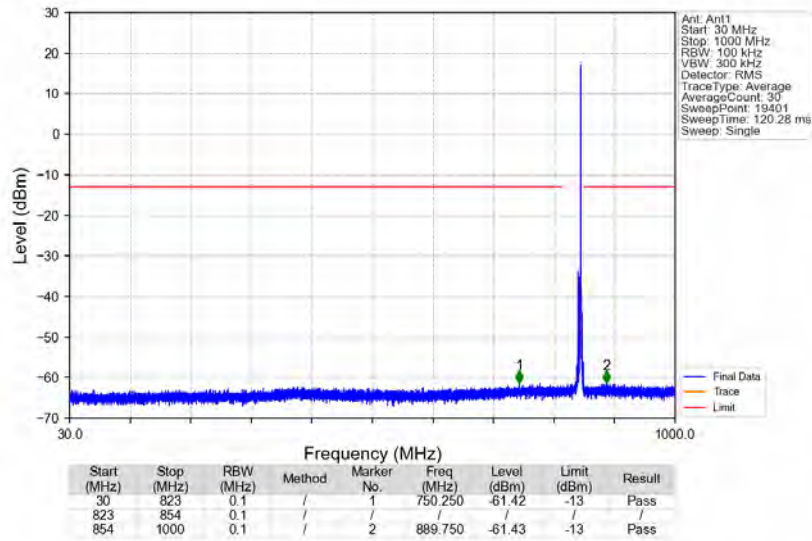
n5_15kHz_SISO_NTNV_5MHz_CP-OFDM QPSK_846.5MHz_Edge_1RB_Right
