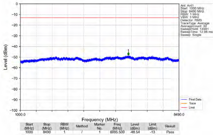
n5_15kHz_SISO_NTNV_10MHz_CP-OFDM QPSK_829MHz_Edge_1RB_Left
