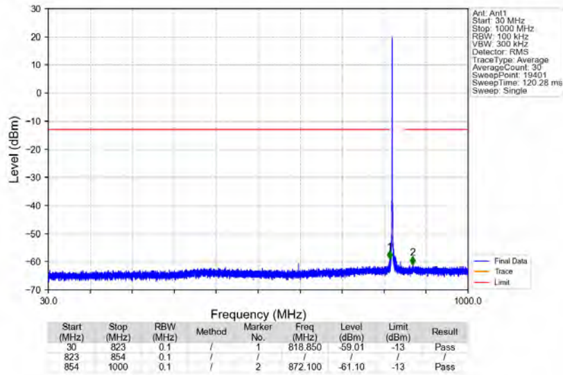
n5_15kHz_SISO_NTNV_15MHz_DFT-s-OFDM QPSK_831.5MHz_Edge_1RB_Left
