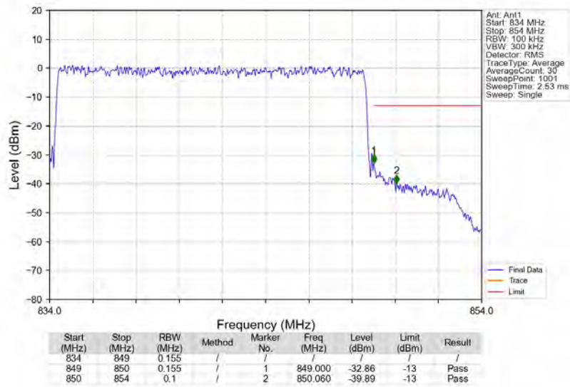
n5_15kHz_SISO_NTNV_15MHz_CP-OFDM QPSK_841.5MHz_Outer_Full
