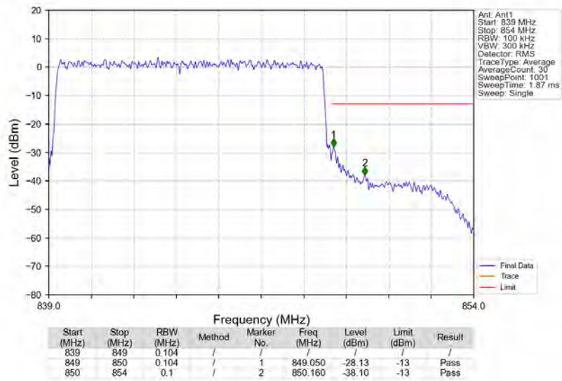
n5_15kHz_SISO_NTNV_10MHz_CP-OFDM QPSK_844MHz_Outer_Full
