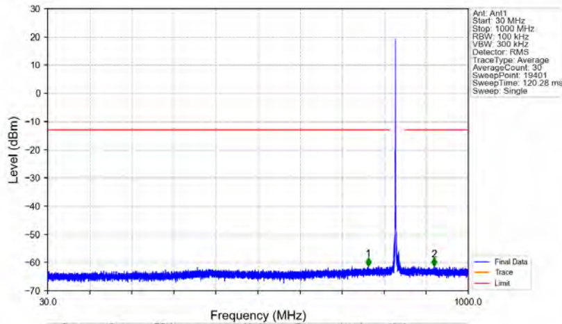
n5_15kHz_SISO_NTNV_10MHz_DFT-s-OFDM QPSK_836.5MHz_Edge_1RB_Left
