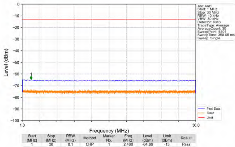
n5_15kHz_SISO_NTNV_15MHz_CP-OFDM QPSK_836.5MHz_Edge_1RB_Left
