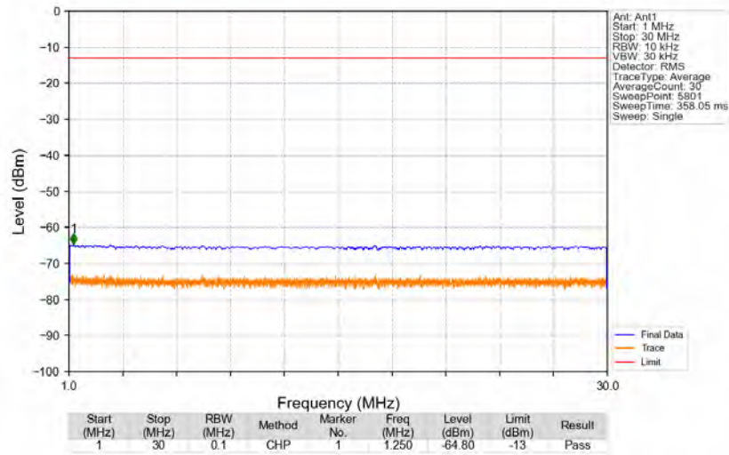
n5_15kHz_SISO_NTNV_15MHz_CP-OFDM QPSK_841.5MHz_Edge_1RB_Right
