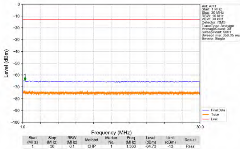
n5_15kHz_SISO_NTNV_10MHz_CP-OFDM QPSK_836.5MHz_Edge_1RB_Left
