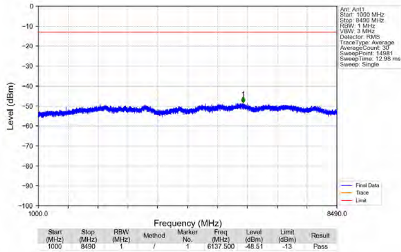
n5_15kHz_SISO_NTNV_15MHz_DFT-s-OFDM QPSK_841.5MHz_Edge_1RB_Right
