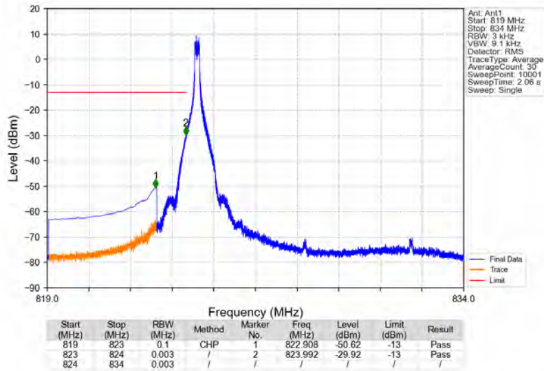
n5_15kHz_SISO_NTNV_10MHz_DFT-s-OFDM QPSK_829MHz_Edge_1RB_Left
