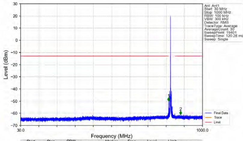
n5_15kHz_SISO_NTNV_15MHz_DFT-s-OFDM PI/2 BPSK_836.5MHz_Edge_1RB_Left
