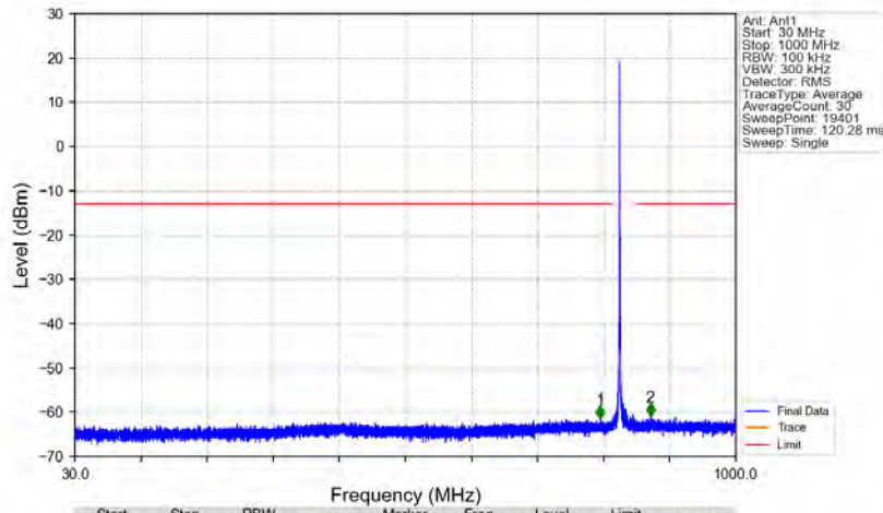
n5_15kHz_SISO_NTNV_15MHz_DFT-s-OFDM QPSK_836.5MHz_Edge_1RB_Left
