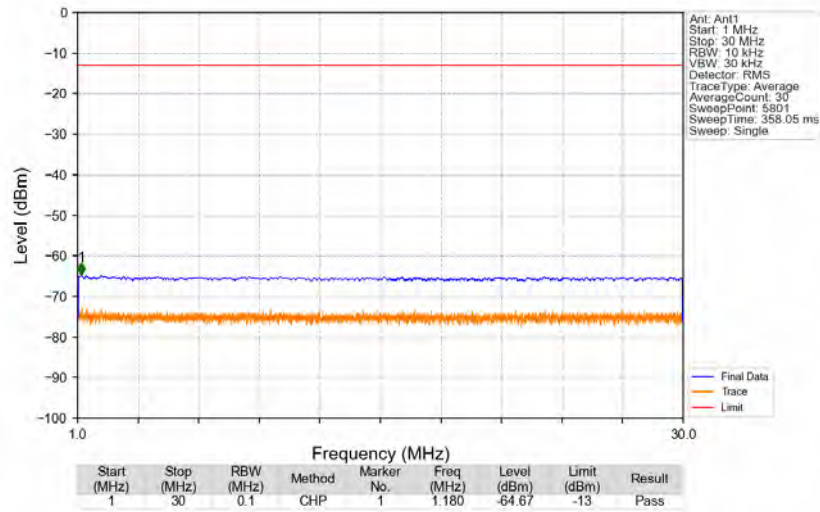
n5_15kHz_SISO_NTNV_15MHz_DFT-s-OFDM QPSK_836.5MHz_Edge_1RB_Left
