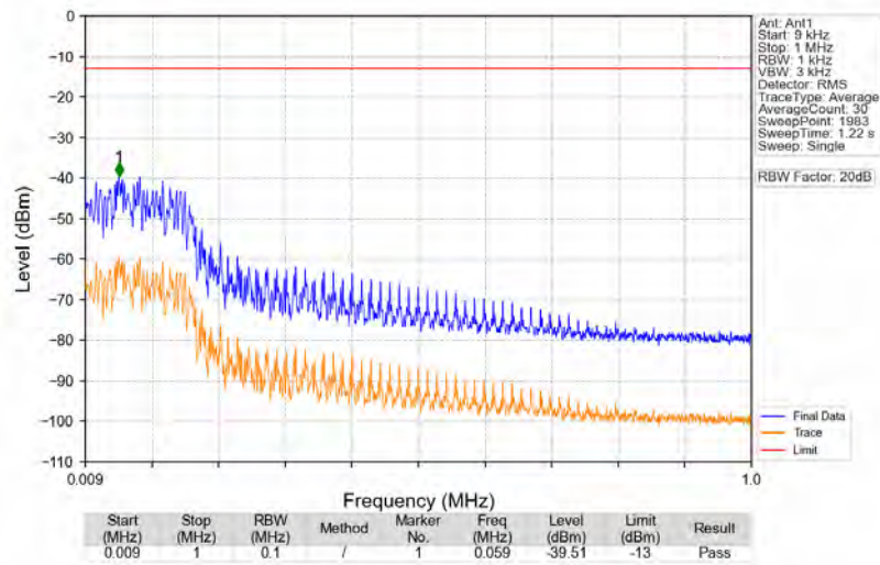
n5_15kHz_SISO_NTNV_20MHz_DFT-s-OFDM QPSK_834MHz_Edge_1RB_Left
