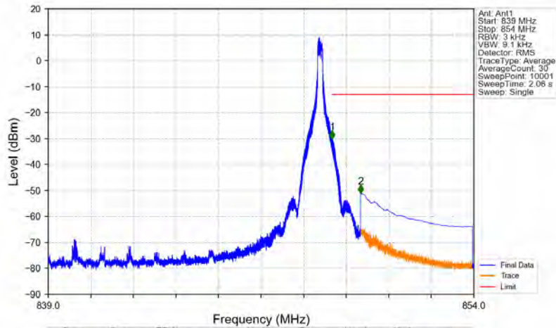
n5_15kHz_SISO_NTNV_10MHz_DFT-s-OFDM PI/2 BPSK_844MHz_Edge_1RB_Right
