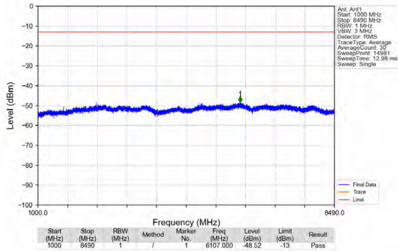
n5_15kHz_SISO_NTNV_15MHz_DFT-s-OFDM PI/2 BPSK_831.5MHz_Edge_1RB_Left
