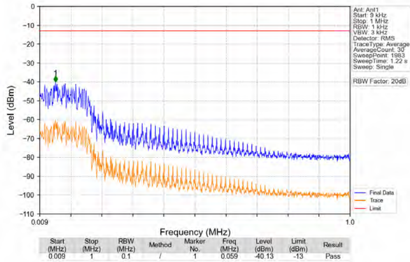
n5_15kHz_SISO_NTNV_10MHz_DFT-s-OFDM QPSK_829MHz_Edge_1RB_Left
