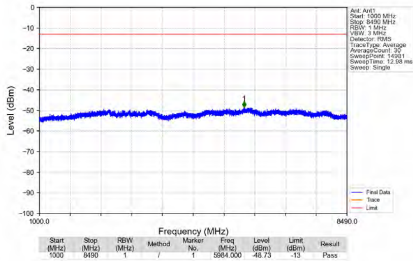
n5_15kHz_SISO_NTNV_15MHz_CP-OFDM QPSK_831.5MHz_Edge_1RB_Left
