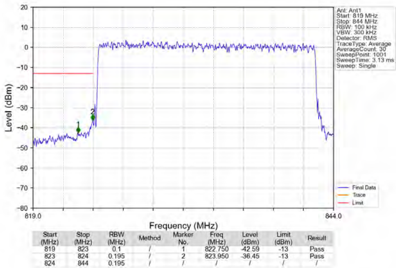
n5_15kHz_SISO_NTNV_20MHz_DFT-s-OFDM PI/2 BPSK_834MHz_Outer_Full
