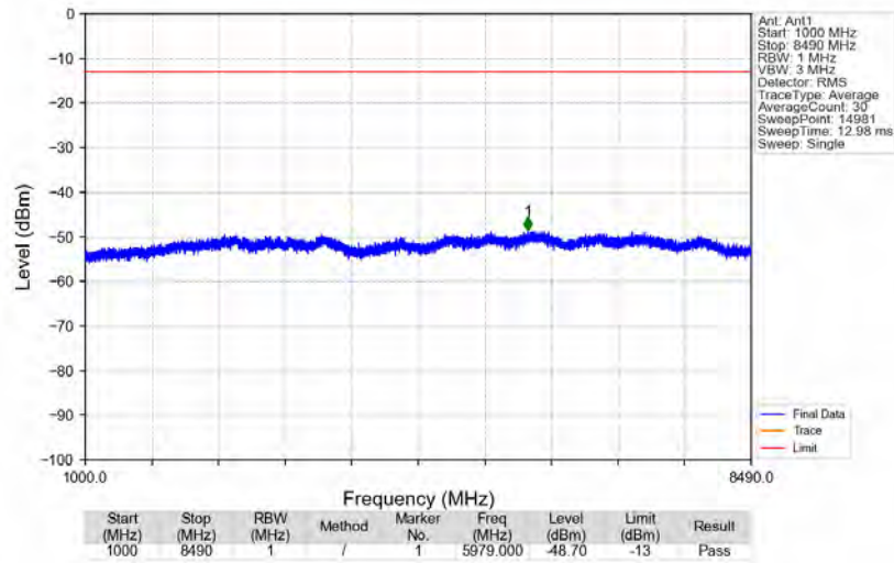
n5_15kHz_SISO_NTNV_20MHz_CP-OFDM QPSK_839MHz_Edge_1RB_Right
