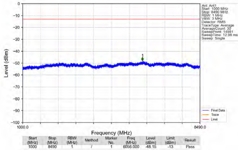
n5_15kHz_SISO_NTNV_20MHz_DFT-s-OFDM PI/2 BPSK_839MHz_Edge_1RB_Right
