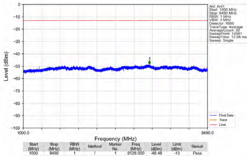
n5_15kHz_SISO_NTNV_15MHz_DFT-s-OFDM QPSK_831.5MHz_Edge_1RB_Left
