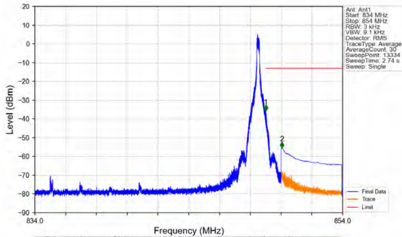
n5_15kHz_SISO_NTNV_15MHz_DFT-s-OFDM PI/2 BPSK_841.5MHz_Edge_1RB_Right
