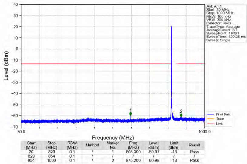
n5_15kHz_SISO_NTNV_10MHz_DFT-s-OFDM QPSK_829MHz_Edge_1RB_Left
