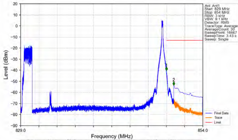
n5_15kHz_SISO_NTNV_20MHz_CP-OFDM QPSK_839MHz_Edge_1RB_Right
