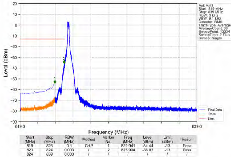
n5_15kHz_SISO_NTNV_15MHz_CP-OFDM QPSK_831.5MHz_Edge_1RB_Left
