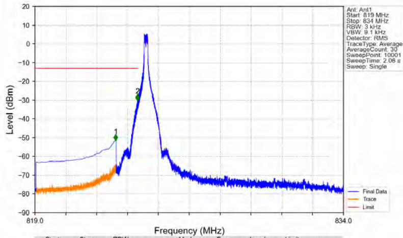
n5_15kHz_SISO_NTNV_10MHz_CP-OFDM QPSK_829MHz_Edge_1RB_Left
