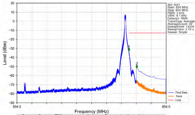
n5_15kHz_SISO_NTNV_15MHz_DFT-s-OFDM QPSK_841.5MHz_Edge_1RB_Right
