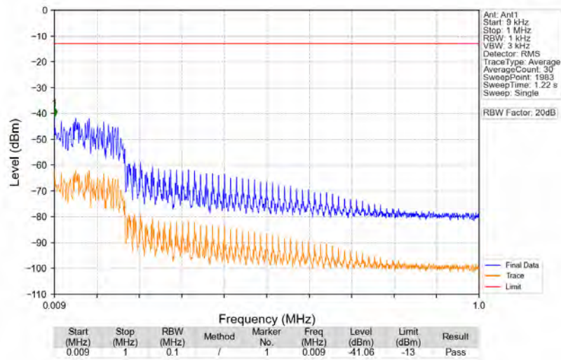
n5_15kHz_SISO_NTNV_10MHz_DFT-s-OFDM QPSK_844MHz_Edge_1RB_Right
