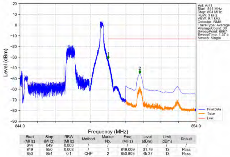
n5_15kHz_SISO_NTNV_5MHz_CP-OFDM QPSK_846.5MHz_Edge_1RB_Right
