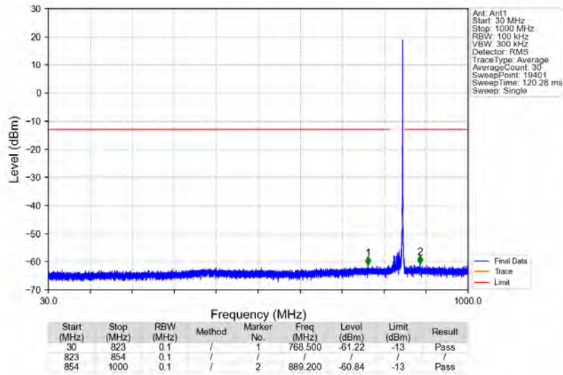
n5_15kHz_SISO_NTNV_20MHz_DFT-s-OFDM QPSK_839MHz_Edge_1RB_Right
