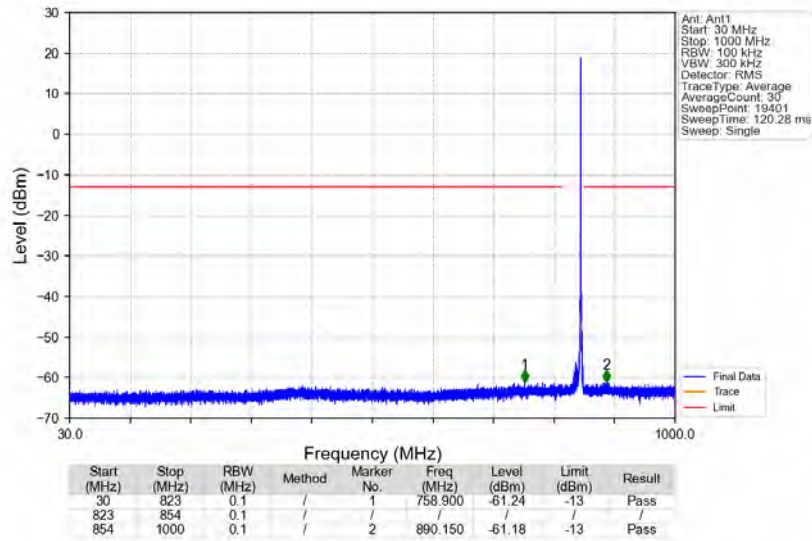
n5_15kHz_SISO_NTNV_10MHz_DFT-s-OFDM QPSK_844MHz_Edge_1RB_Right
