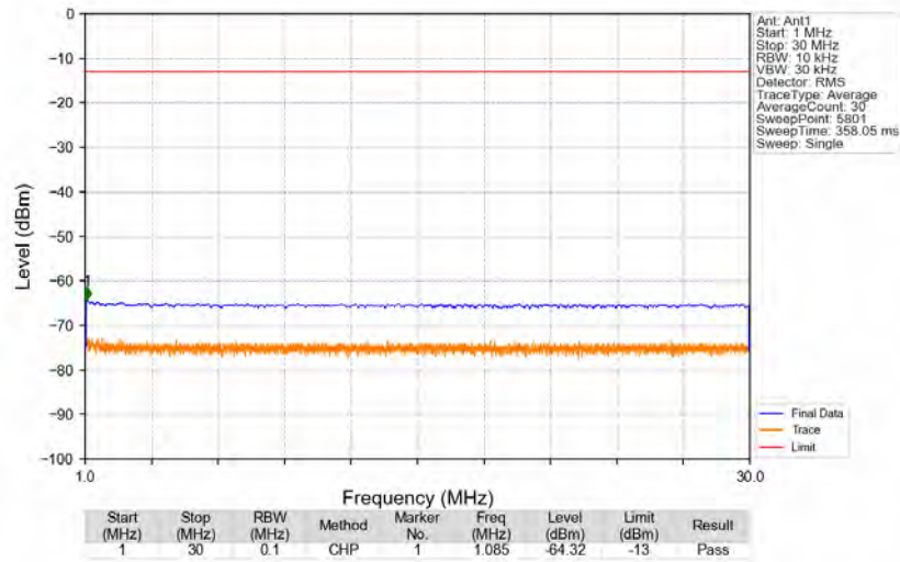
n5_15kHz_SISO_NTNV_5MHz_CP-OFDM QPSK_846.5MHz_Edge_1RB_Right
