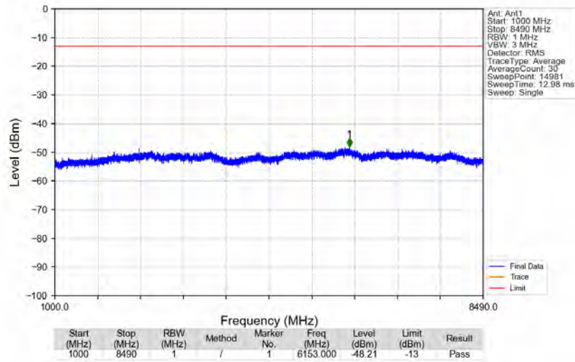
n5_15kHz_SISO_NTNV_10MHz_DFT-s-OFDM QPSK_829MHz_Edge_1RB_Left
