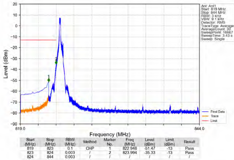
n5_15kHz_SISO_NTNV_20MHz_DFT-s-OFDM PI/2 BPSK_834MHz_Edge_1RB_Left
