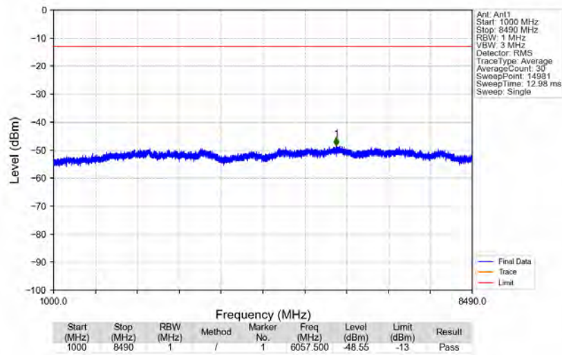
n5_15kHz_SISO_NTNV_20MHz_DFT-s-OFDM QPSK_839MHz_Edge_1RB_Right
