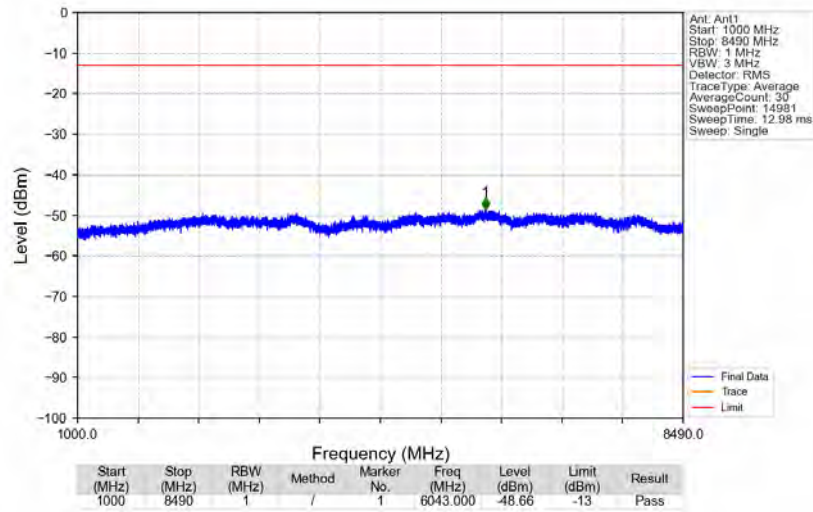
n5_15kHz_SISO_NTNV_10MHz_DFT-s-OFDM QPSK_844MHz_Edge_1RB_Right
