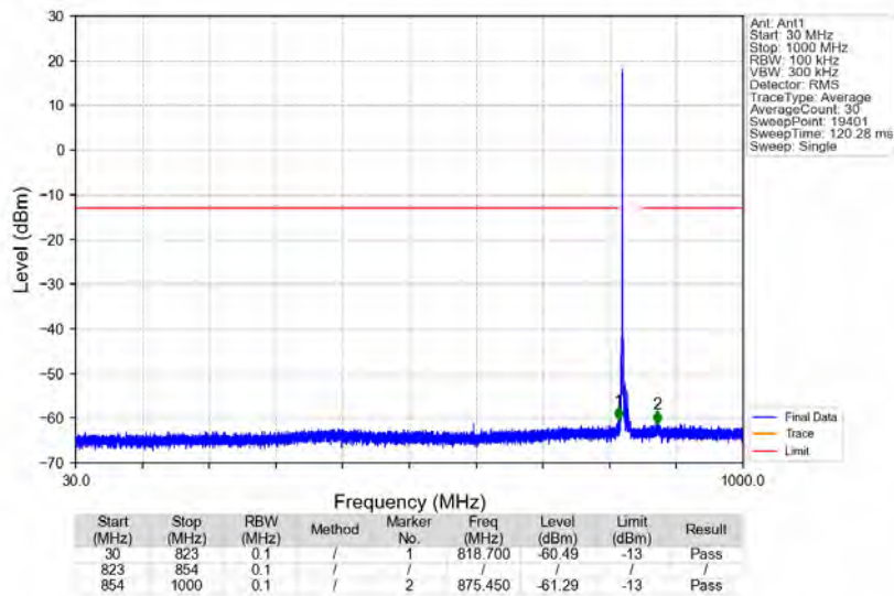
n5_15kHz_SISO_NTNV_10MHz_CP-OFDM QPSK_829MHz_Edge_1RB_Left
