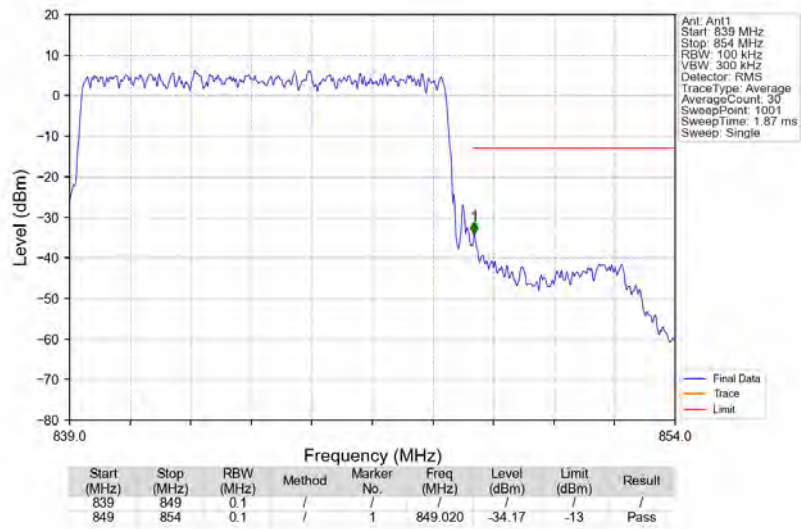
n5_15kHz_SISO_NTNV_10MHz_DFT-s-OFDM PI/2 BPSK_844MHz_Outer_Full
