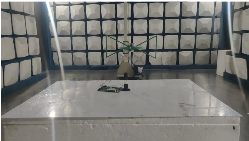
Radiated Spurious Emissions (30MHz-1GHz)
