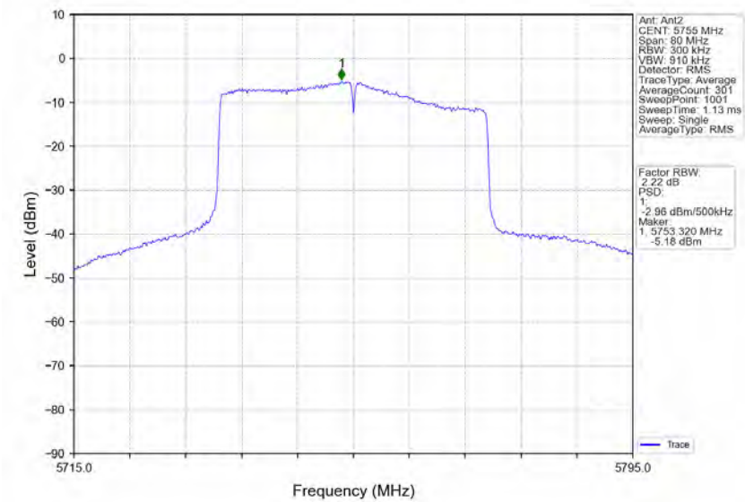
802.11ax(HEW40)_LCH_5755MHz_RU484_Left_MIMO_NTNV
