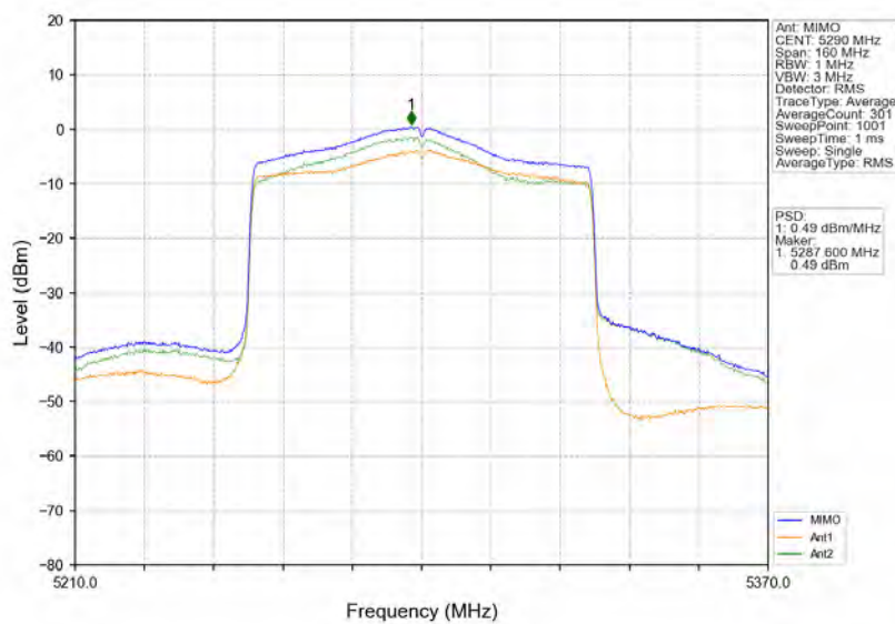
802.11ax(HEW80)_MCH_5290MHz_RU996_Left_MIMO_NTNV
