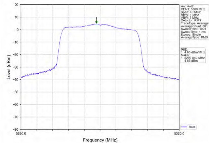
802.11ax(HEW20)_MCH_5300MHz_RU242_Left_Ant2_NTNV
