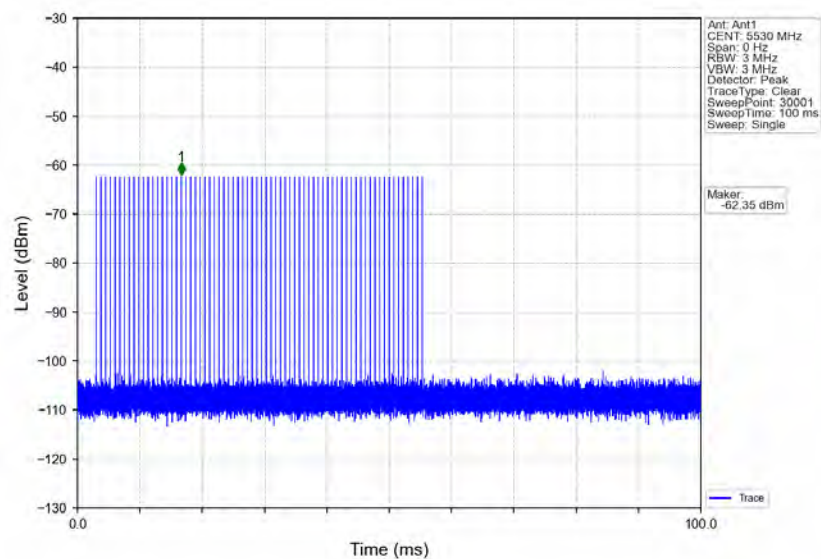
Signal Calibration 802.11ax(HEW80) 2C 5530MHz_RadarType2_Trial0
