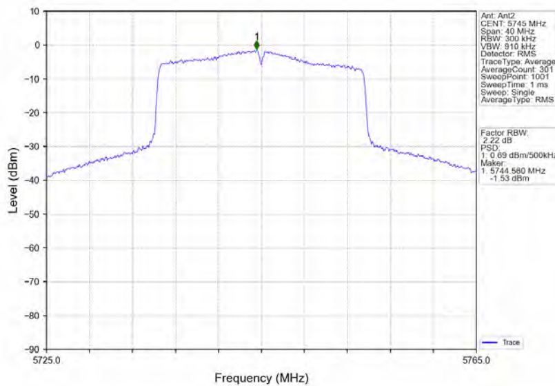
802.11ax(HEW20)_LCH_5745MHz_RU242_Left_Ant2_NTNV
