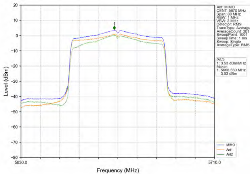
802.11ax(HEW40)_HCH_5670MHz_RU484_Left_MIMO_NTNV
