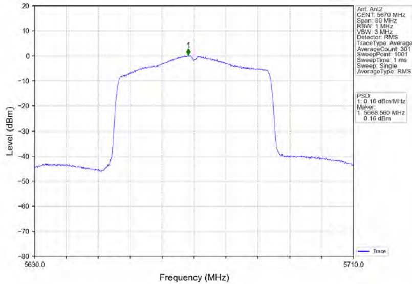
802.11ax(HEW40)_HCH_5670MHz_RU484_Left_MIMO_NTNV
