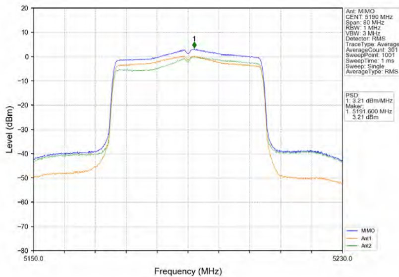
802.11ax(HEW40)_LCH_5190MHz_RU484_Left_MIMO_NTNV
