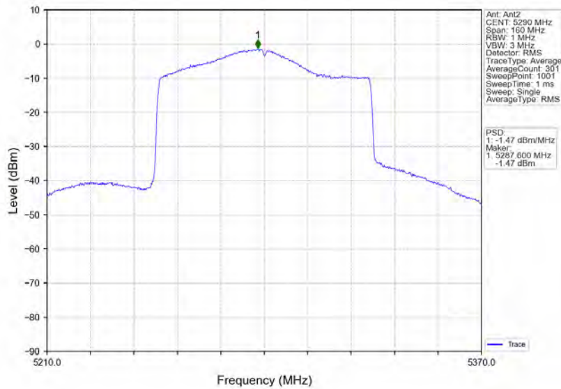
802.11ax(HEW80)_MCH_5290MHz_RU996_Left_MIMO_NTNV
