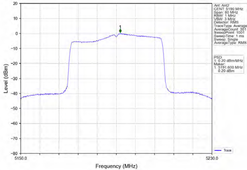
802.11ax(HEW40)_LCH_5190MHz_RU484_Left_MIMO_NTNV
