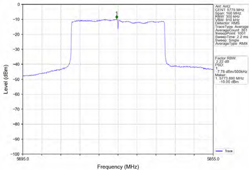
802.11ax(HEW80)_MCH_5775MHz_RU996_Left_MIMO_NTNV
