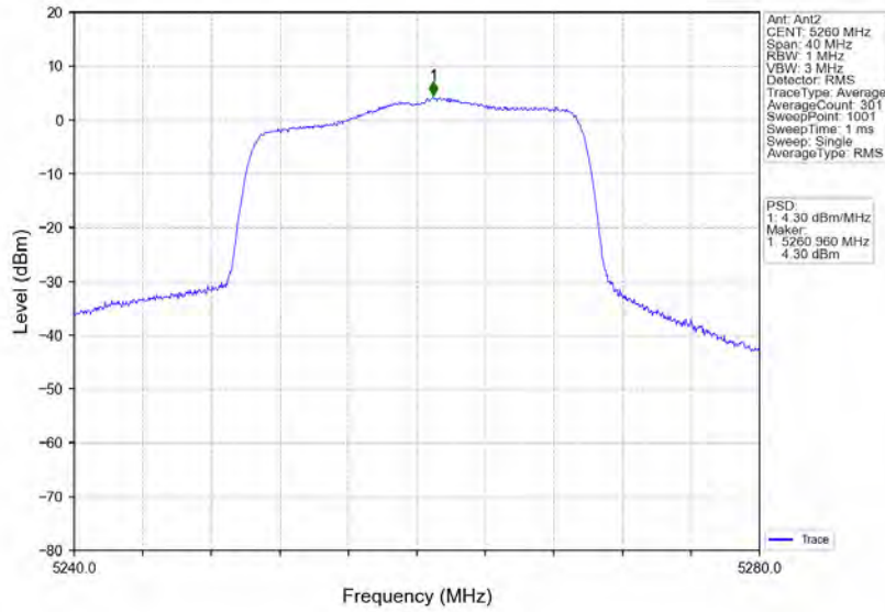
802.11ax(HEW20)_LCH_5260MHz_RU242_Left_MIMO_NTNV
