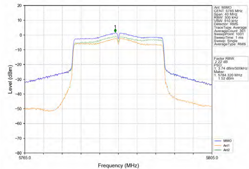
802.11ax(HEW20)_MCH_5785MHz_RU242_Left_MIMO_NTNV
