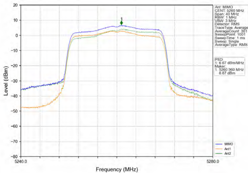
802.11ax(HEW20)_LCH_5260MHz_RU242_Left_MIMO_NTNV
