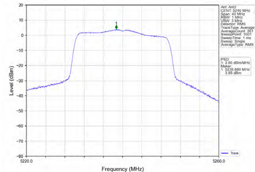
802.11ax(HEW20)_HCH_5240MHz_RU242_Left_Ant2_NTNV
