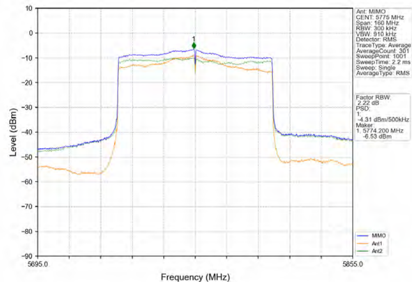
802.11ax(HEW80)_MCH_5775MHz_RU996_Left_MIMO_NTNV
