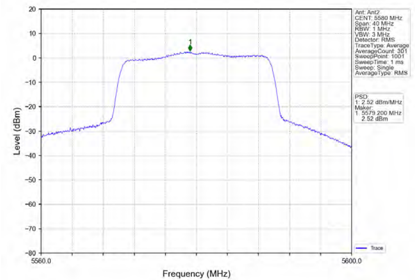
802.11ax(HEW20)_MCH_5580MHz_RU242_Left_MIMO_NTNV
