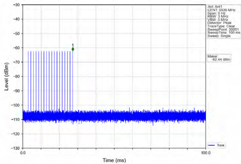
Signal Calibration 802.11ax(HEW80) 2C 5530MHz_RadarType1_Trial0
