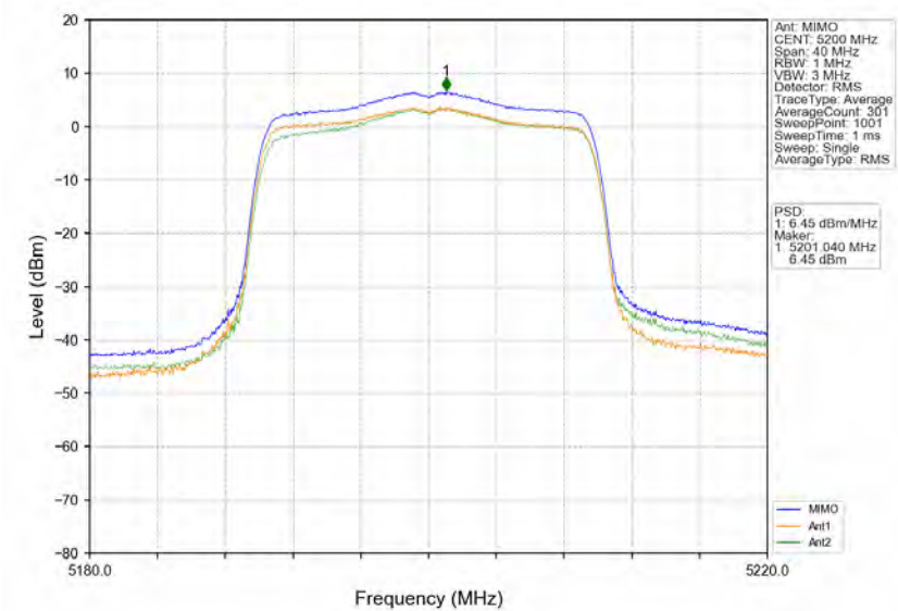
802.11ax(HEW20)_MCH_5200MHz_RU242_Left_MIMO_NTNV
