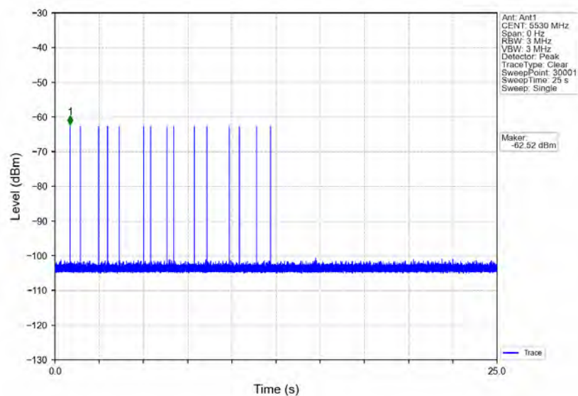
Signal Calibration_802.11ax(HEW80)_2C_5530MHz_RadarType6_Trial0
