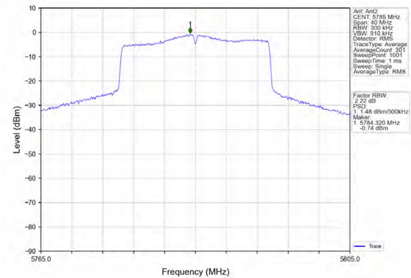
802.11ax(HEW20)_MCH_5785MHz_RU242_Left_MIMO_NTNV
