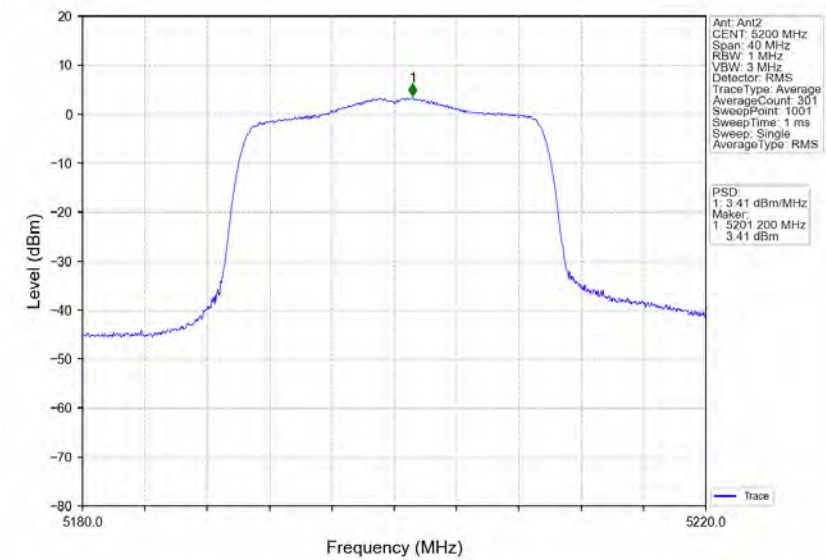
802.11ax(HEW20)_MCH_5200MHz_RU242_Left_MIMO_NTNV
