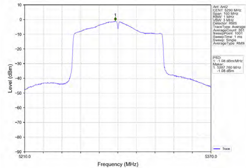
802.11ac(VHT80)_MCH_5290MHz_MIMO_NTNV
