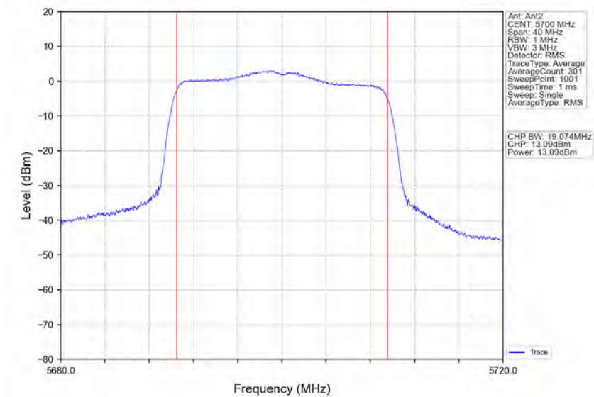
802.11ax(HEW20)_HCH_5700MHz_RU242_Left_Ant2_NTNV
