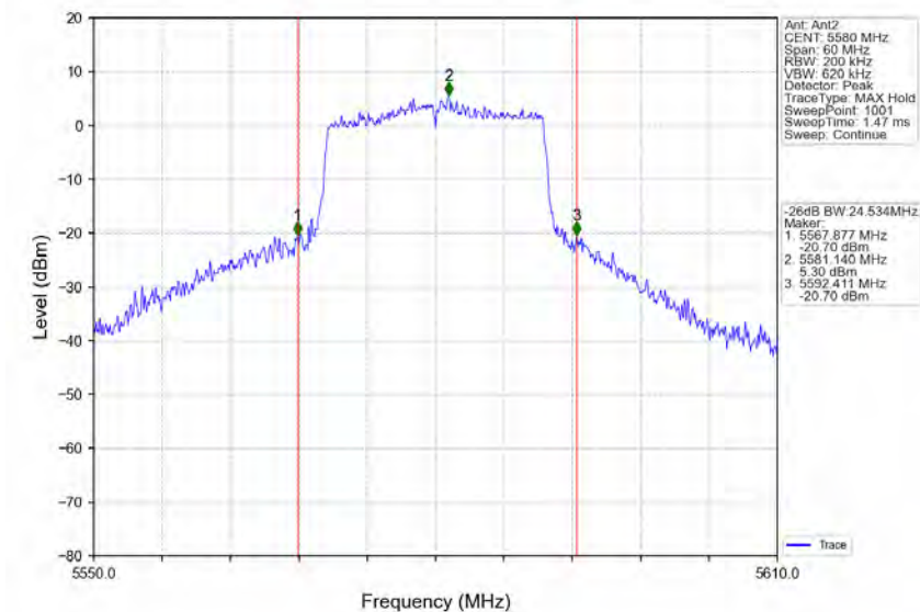
802.11ax(HEW20)_MCH_5580MHz_RU242_Left_Ant2_NTNV
