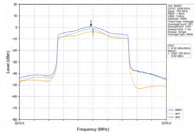
802.11ac(VHT80)_MCH_5290MHz_MIMO_NTNV
