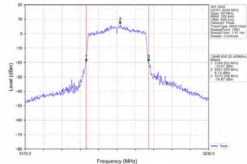
802.11ax(HEW20)_MCH_5200MHz_RU242_Left_Ant2_NTNV
