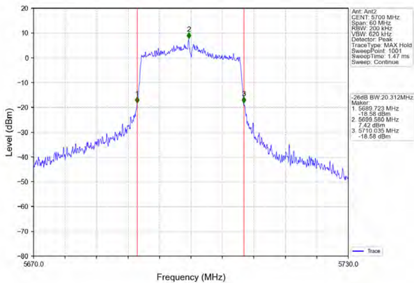
802.11ax(HEW20)_HCH_5700MHz_RU242_Left_Ant2_NTNV
