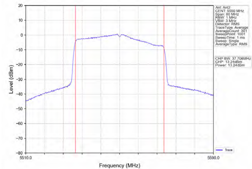
802.11ax(HEW40)_MCH_5550MHz_RU484_Left_Ant2_NTNV
