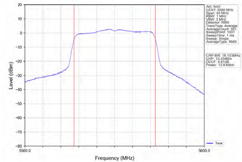
802.11n(HT20)_MCH_5580MHz_Ant2_NTNV
