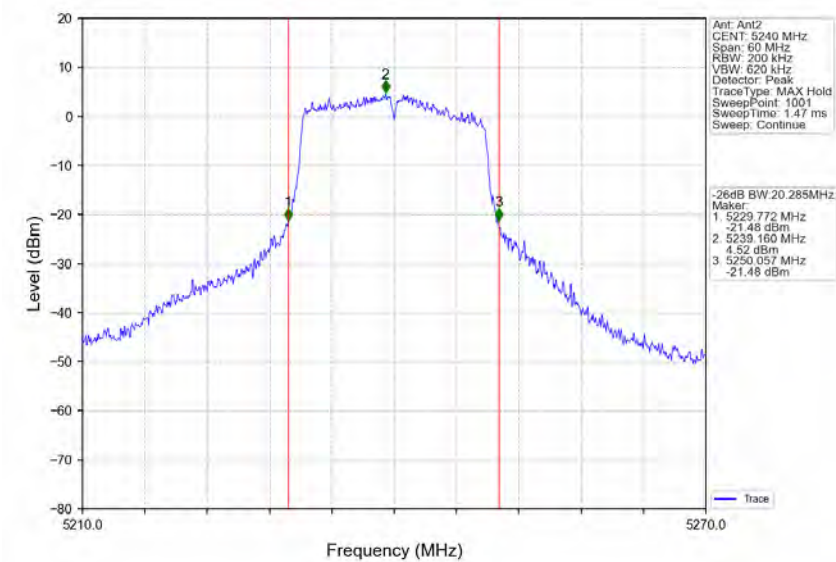
802.11n(HT20)_HCH_5240MHz_Ant2_NTNV
