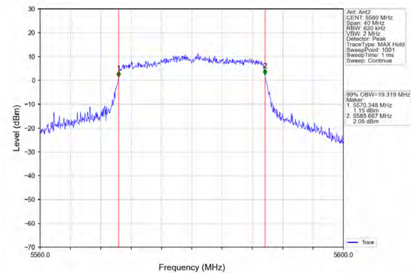
802.11ax(HEW20)_MCH_5580MHz_RU242_Left_Ant2_NTNV
