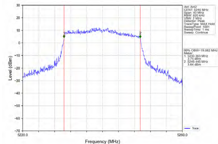
802.11ax(HEW20)_HCH_5240MHz_RU242_Left_Ant2_NTNV
