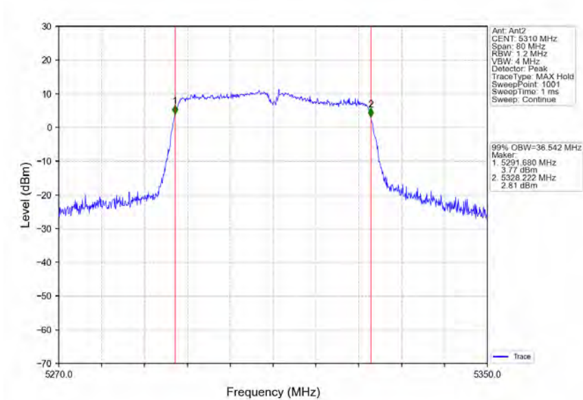
802.11n(HT40)_HCH_5310MHz_Ant2_NTNV
