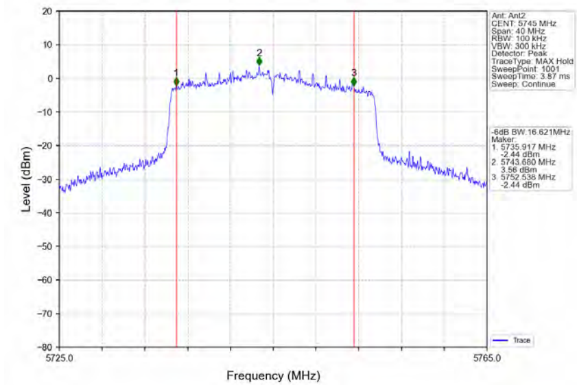
802.11ax(HEW20)_LCH_5745MHz_RU242_Left_Ant2_NTNV
