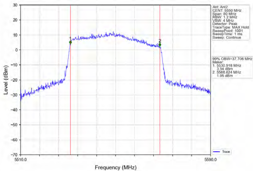
802.11ax(HEW40)_MCH_5550MHz_RU484_Left_Ant2_NTNV
