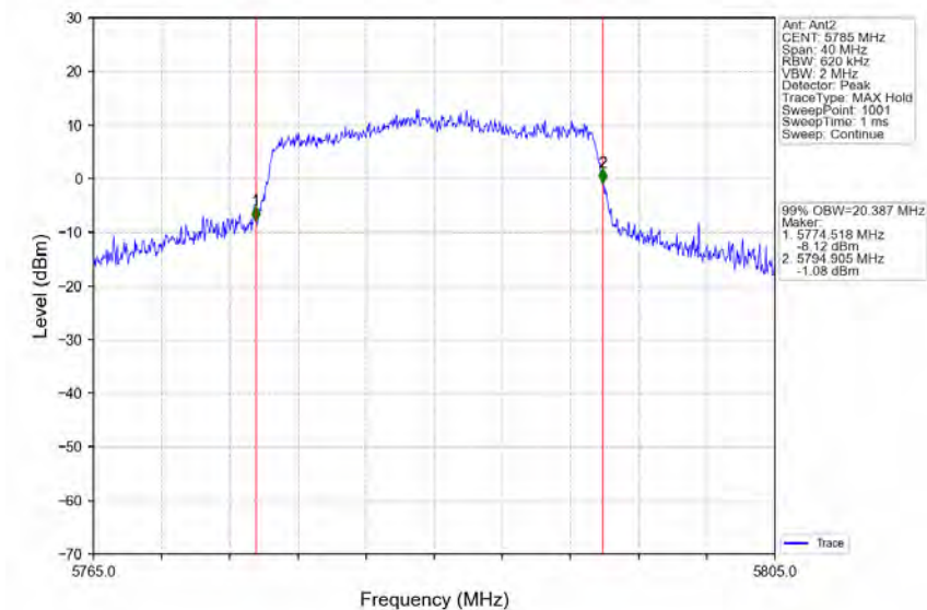
802.11ax(HEW20)_MCH_5785MHz_RU242_Left_Ant2_NTNV
