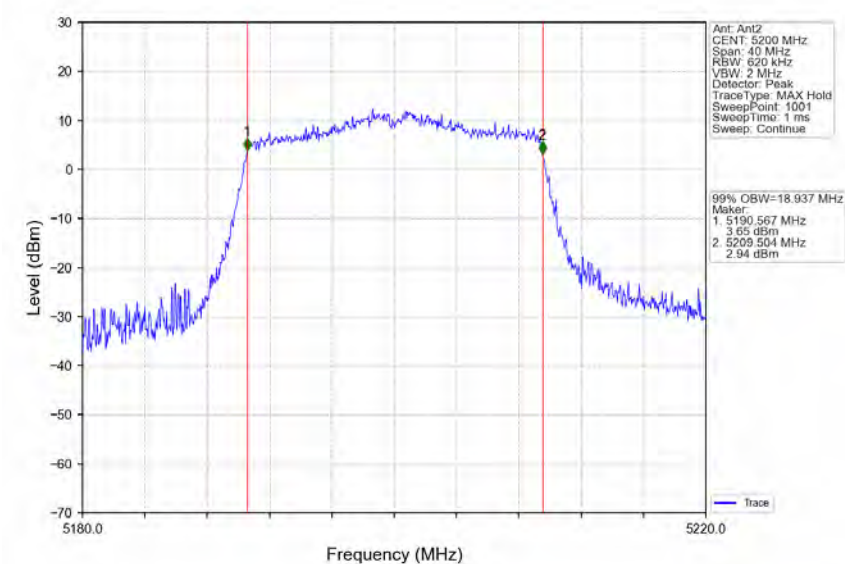
802.11ax(HEW20)_MCH_5200MHz_RU242_Left_Ant2_NTNV
