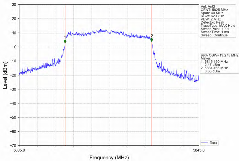
802.11ax(HEW20)_HCH_5825MHz_RU242_Left_Ant2_NTNV
