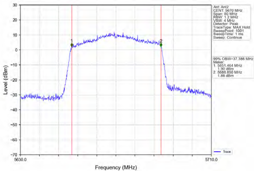
802.11ax(HEW40)_HCH_5670MHz_RU484_Left_Ant2_NTNV
