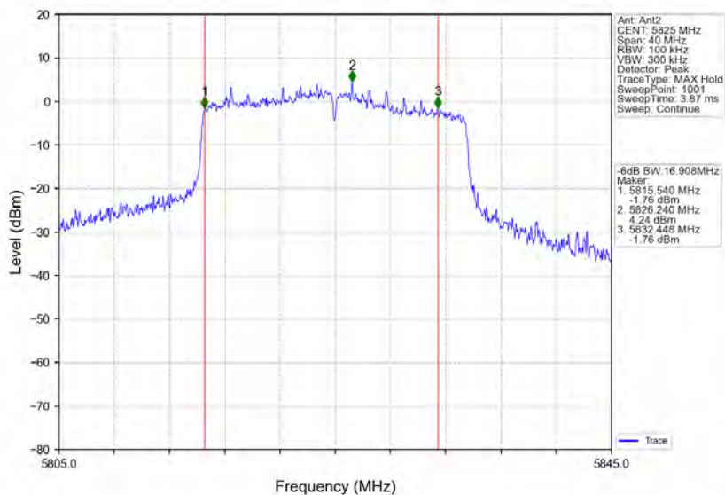
802.11ax(HEW20)_HCH_5825MHz_RU242_Left_Ant2_NTNV
