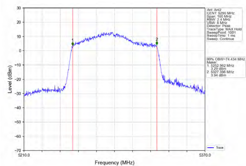
802.11ac(VHT80)_MCH_5290MHz_Ant2_NTNV
