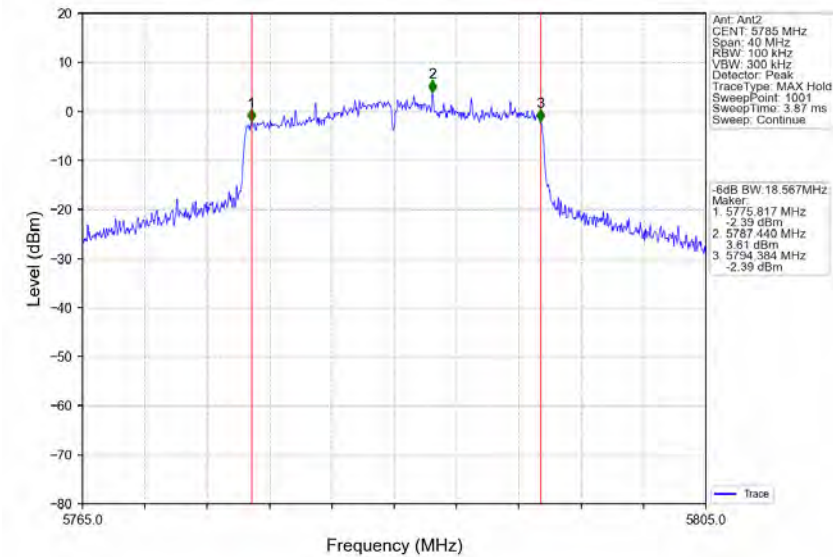
802.11ax(HEW20)_MCH_5785MHz_RU242_Left_Ant2_NTNV
