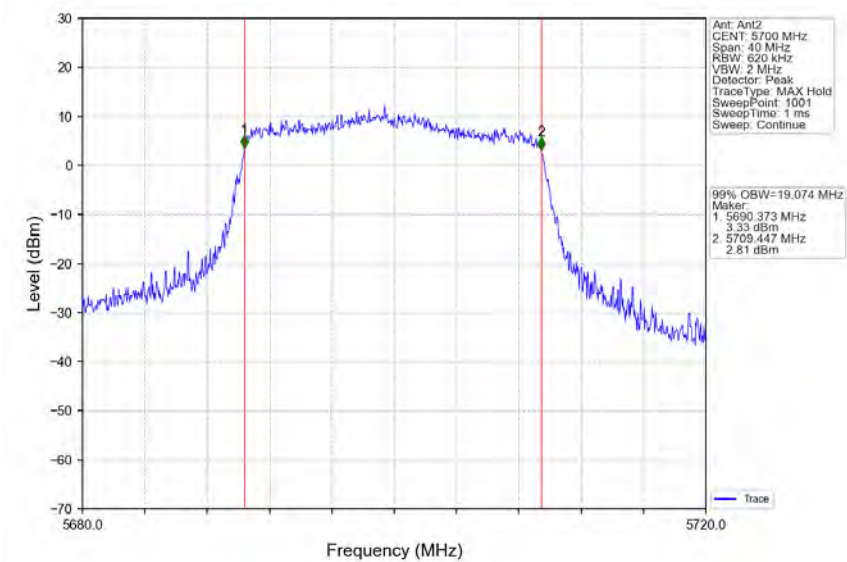
802.11ax(HEW20)_HCH_5700MHz_RU242_Left_Ant2_NTNV
