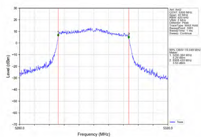
802.11ax(HEW20)_MCH_5300MHz_RU242_Left_Ant2_NTNV
