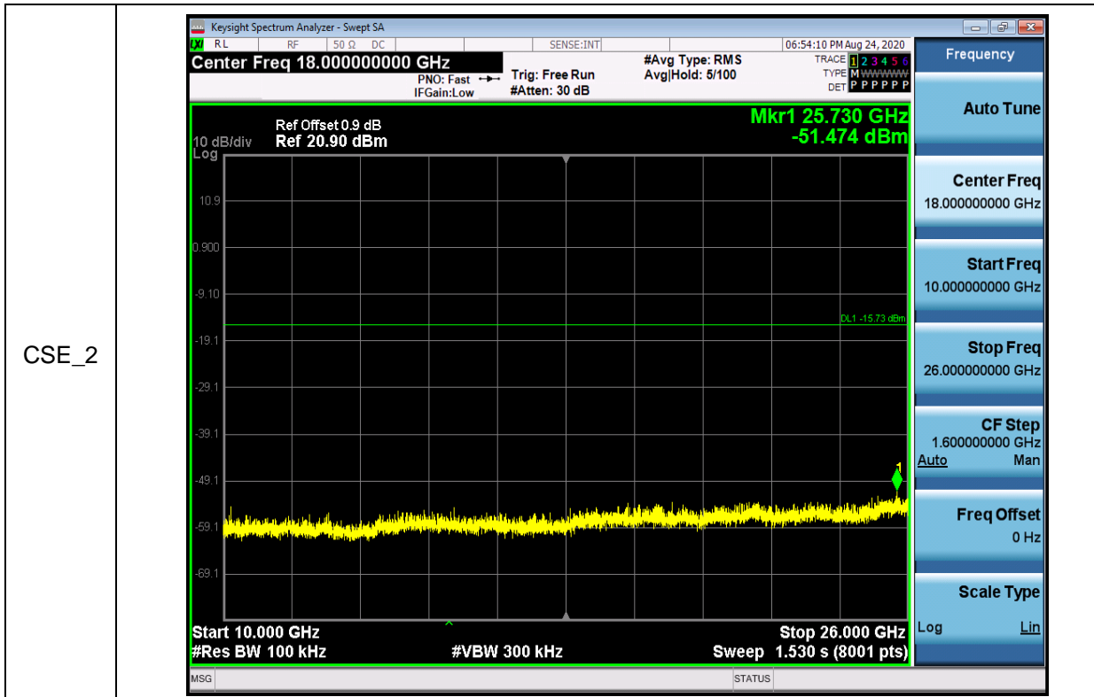
RF Conducted Spurious Emissions_DH5_2441
