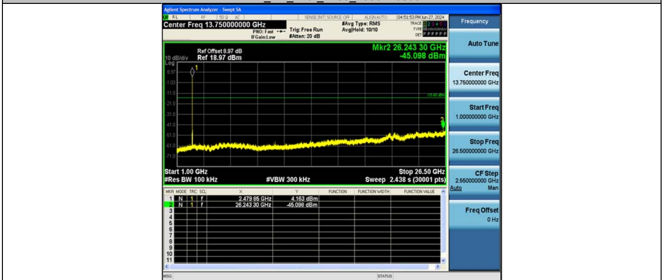
BLE_1M_Ant2_2480_0~Reference
