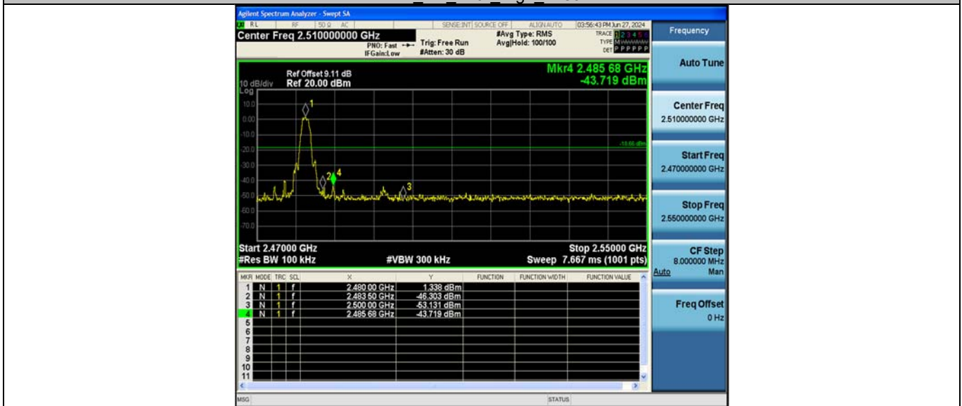
BLE_2M_Ant2_High_2480
