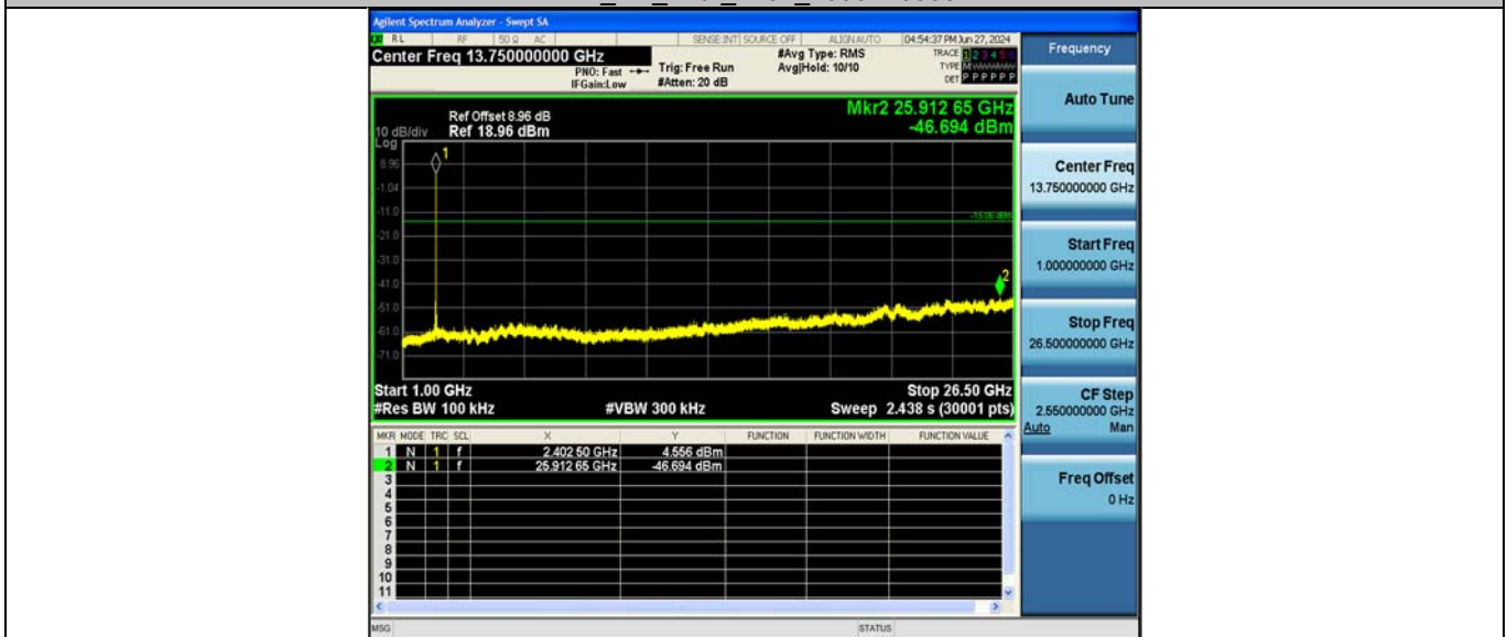
BLE_2M_Ant2_2402_0~Reference
