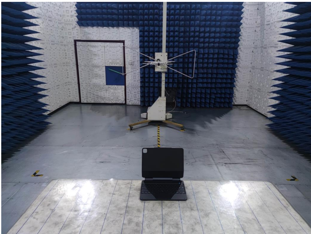
The series model: 6B016A RADIATED EMISSION TEST SETUP BELOW 1GHz
