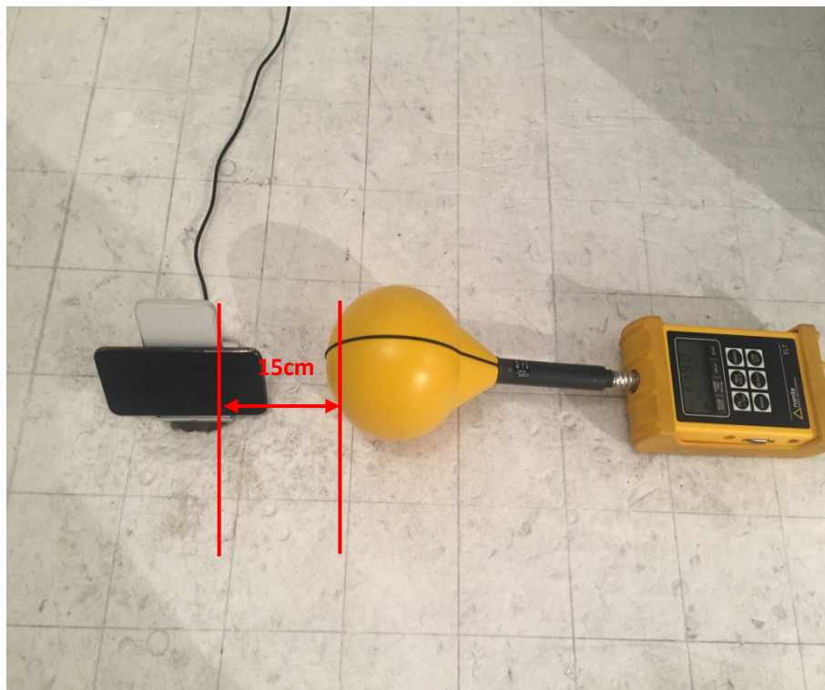
Test Position D-Exposure photo from side edge surface-Right (TM4)
