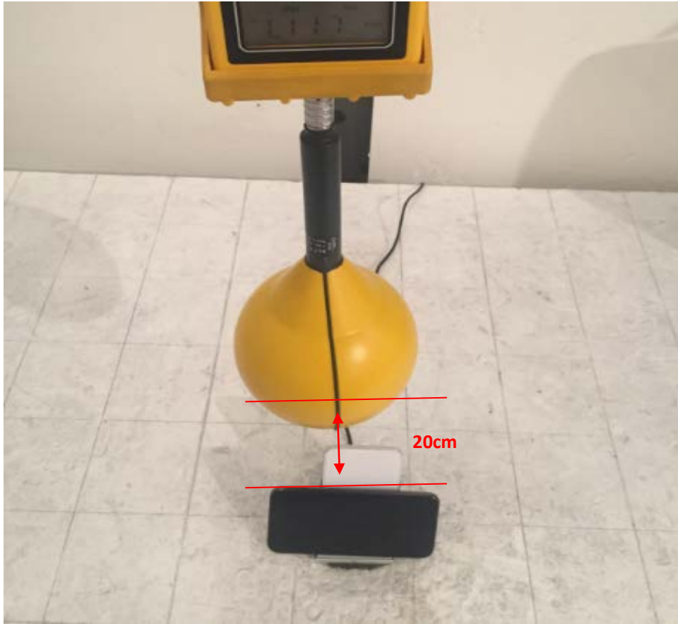
Test Position E-Exposure photo from top surface (20cm) (TM4)
