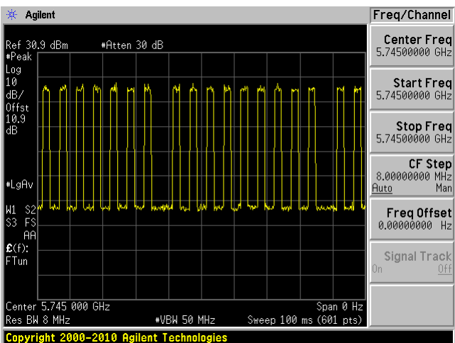
802.11ac20 mode # of Pulses in 100 ms
