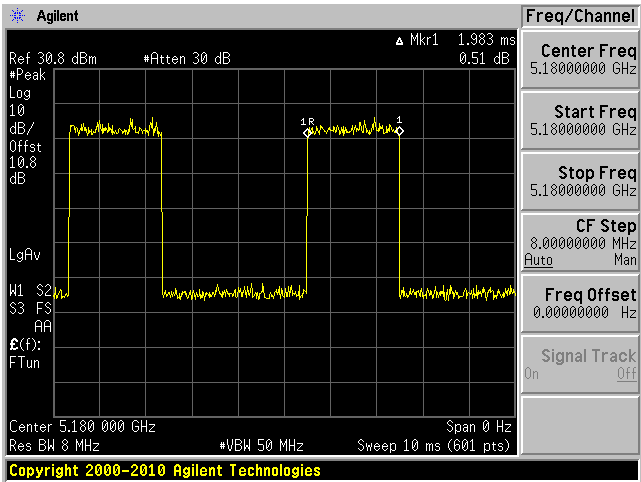
802.11ac20 mode Pulse Width
