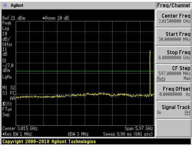
High Channel 5850 MHz (30MHz-6GHz)
