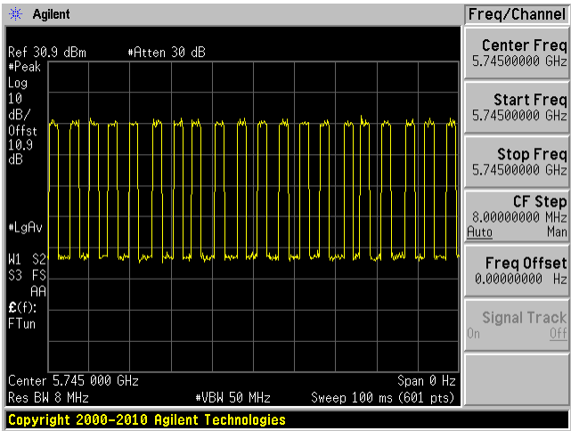
802.11a mode # of Pulses in 100 ms
