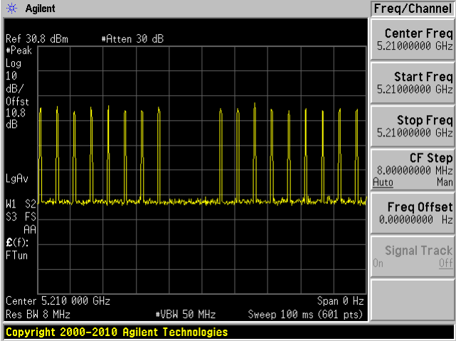
802.11ac80 mode # of Pulses in 100 ms
