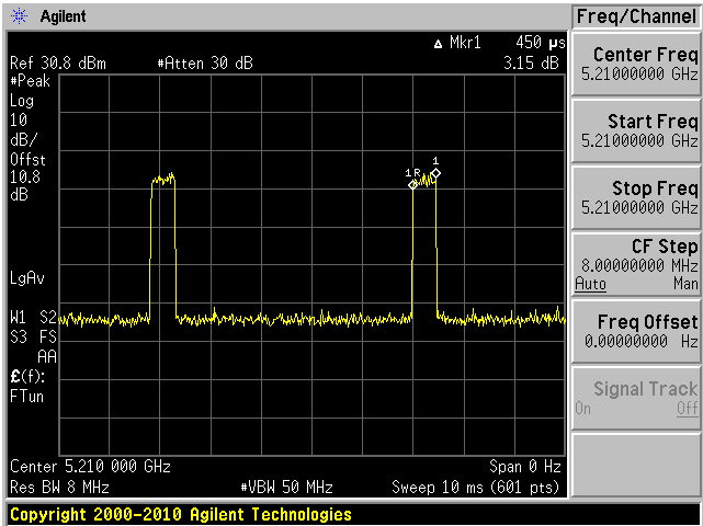
802.11ac80 mode Pulse Width
