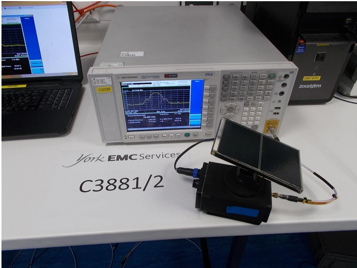
Conducted tests: 20dB bandwidth measurement shown
