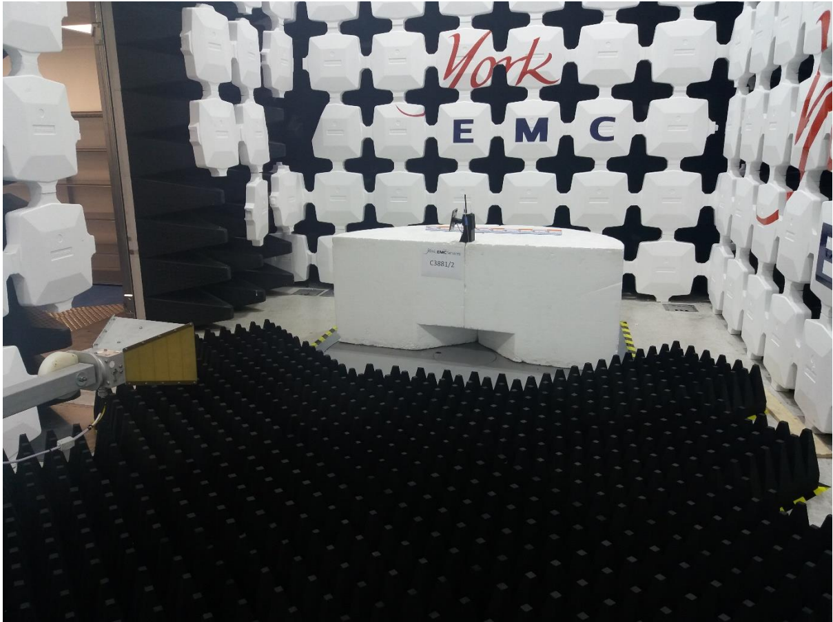
Final radiated electric field emissions 1-10GHz
