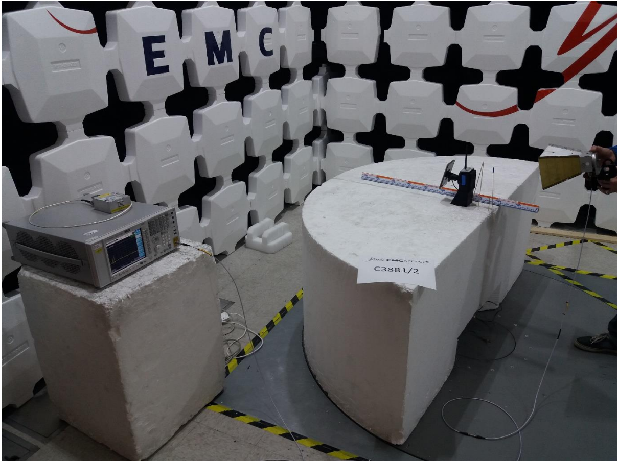
Exploratory radiated electric field emissions 1-10GHz
