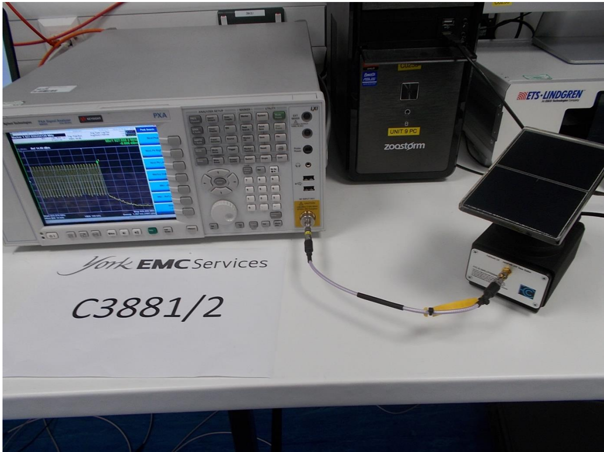
FHSS parameters: Measurement of number of hopping channels shown
