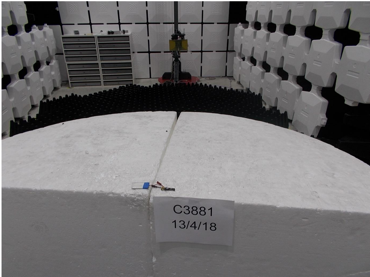
Radiated electric field emissions 1-10GHz
