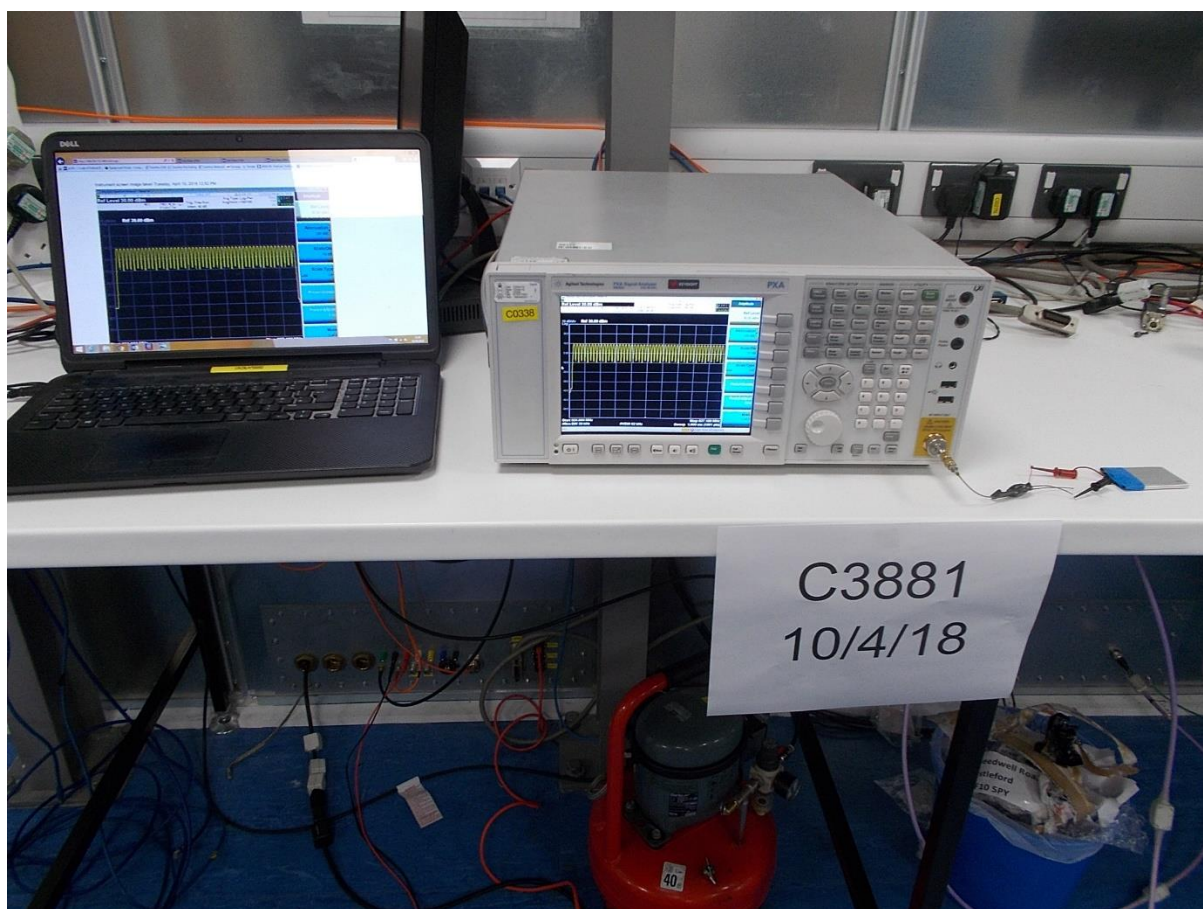
FHSS Parameters – Number of Hopping Channels
