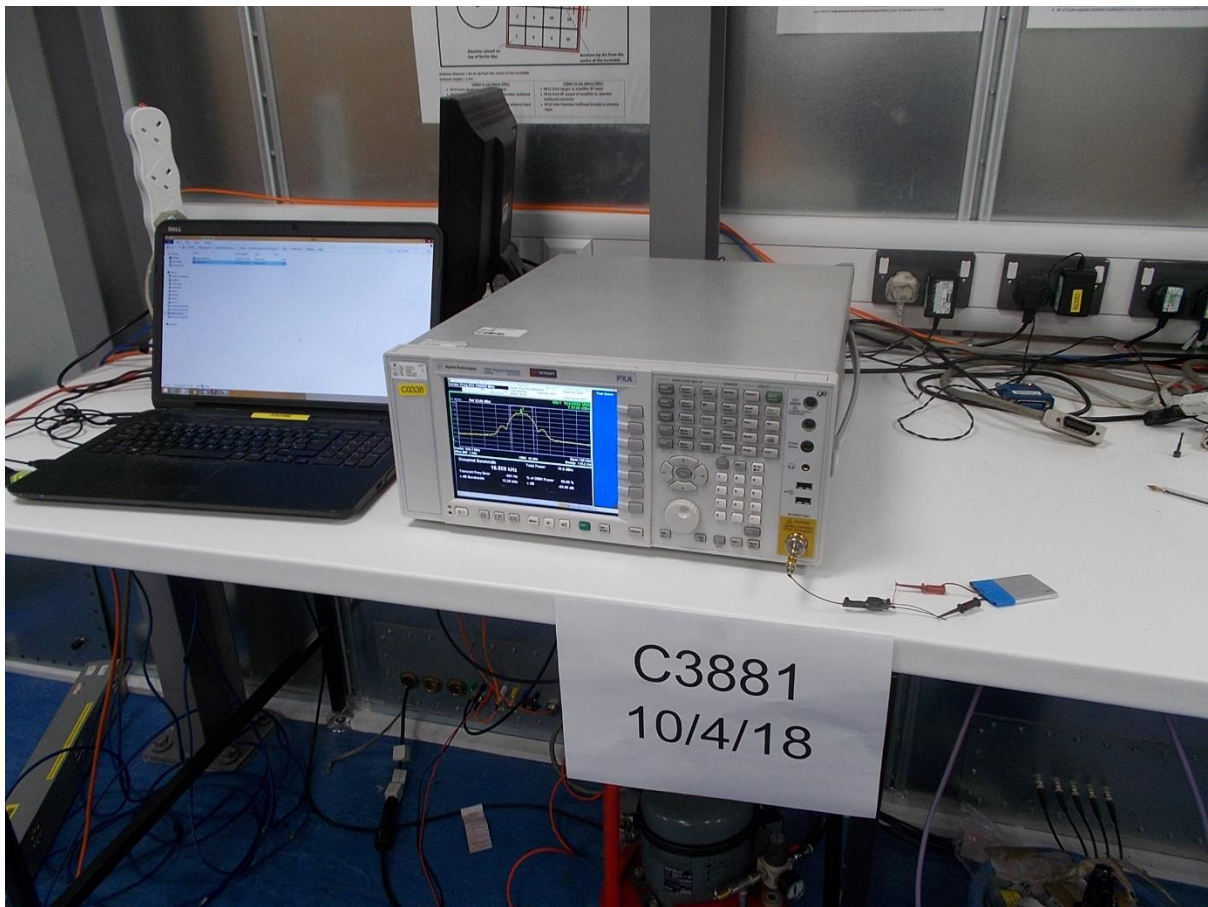
20dB Bandwidth Test
