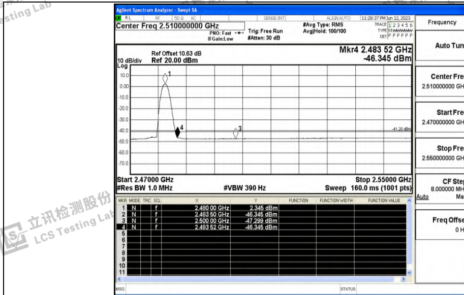
3DH5_Ant1_High_2480_Peak
