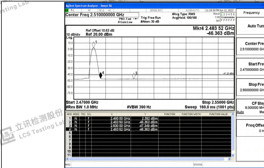
2DH5_Ant1_High_2480_Peak
