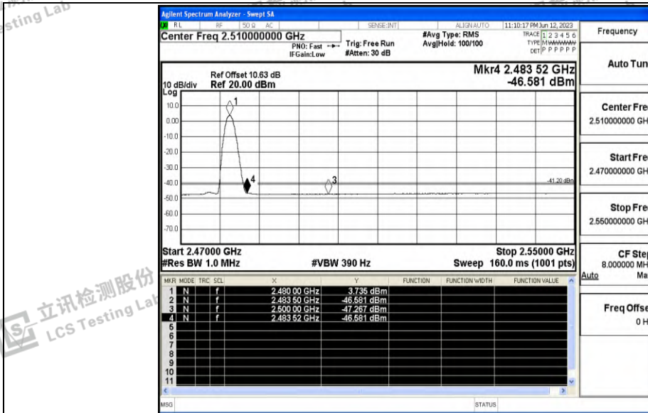
DH5_Ant1_High_2480_Peak
