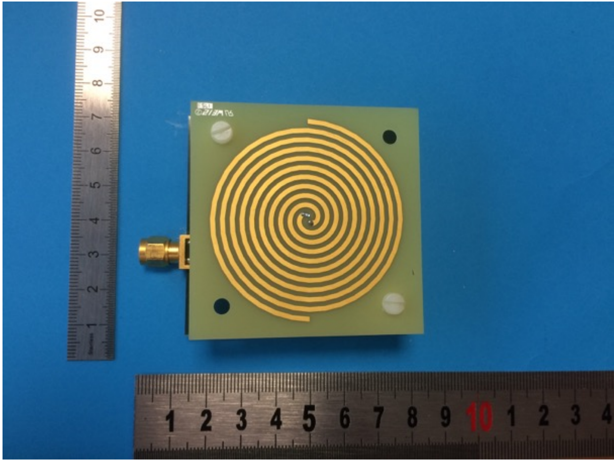
Antenna PCB view
