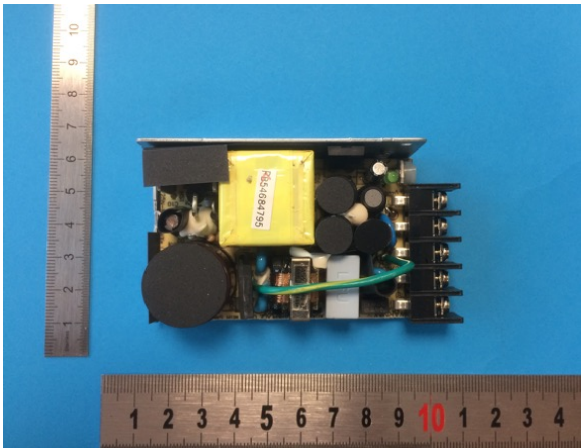
Internal power unit view
