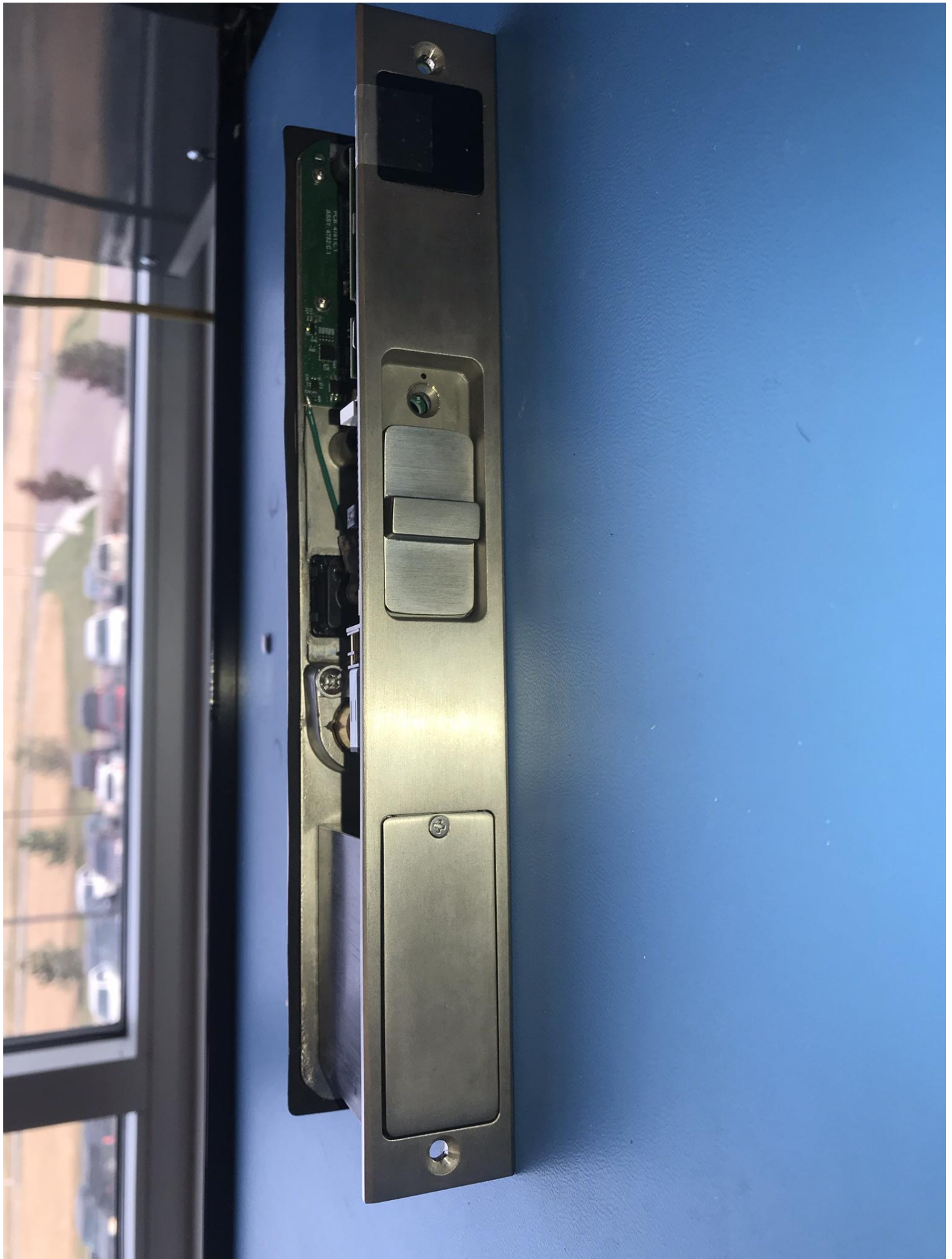
Figure 16 - Interior View, Battery Compartment at Bottom of Photo
