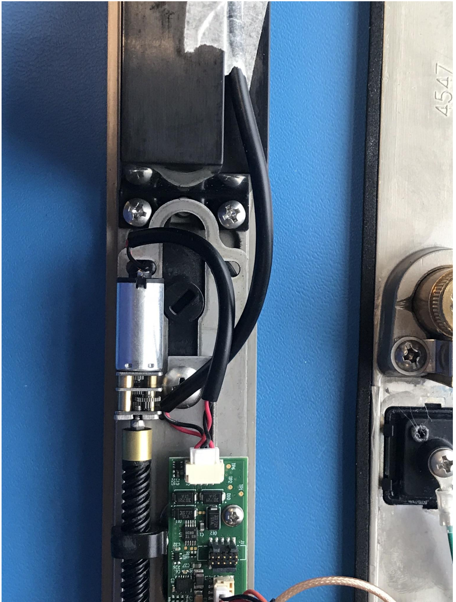
Figure 14 - Battery and Motor Connection
