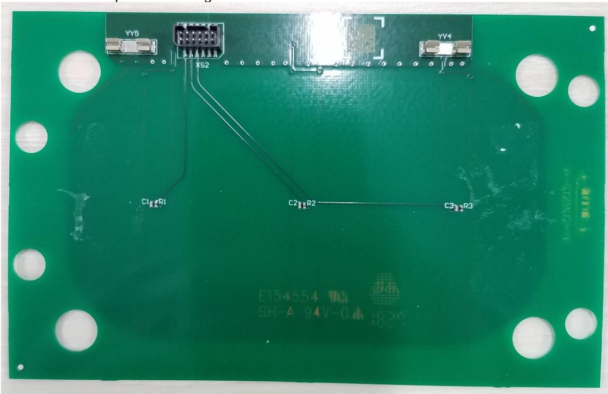
Bottom view of capacitor sensing board
