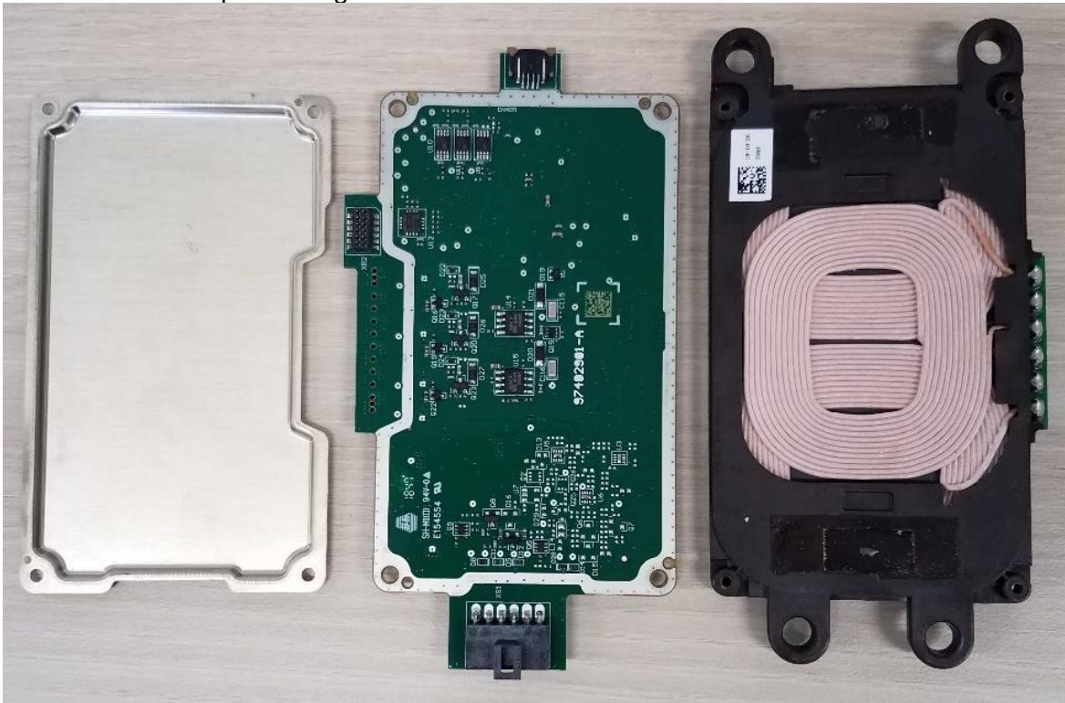
Main board with top shielding
