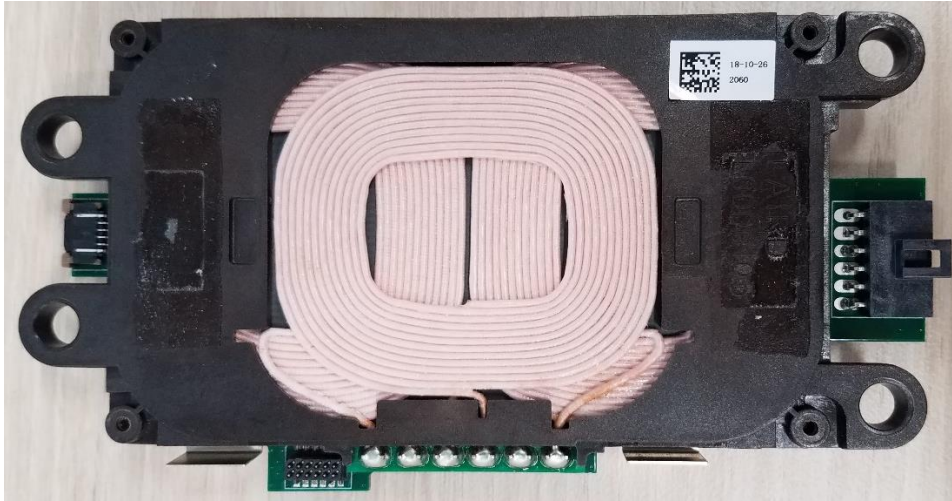
Coil module
