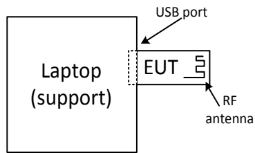
Figure 3.6-1: Setup diagram
