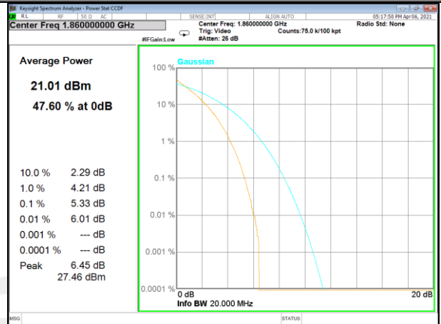
Band 2_100_Q16_Low
