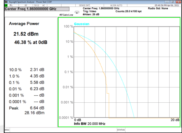
Band 25_100_Q16_Low
