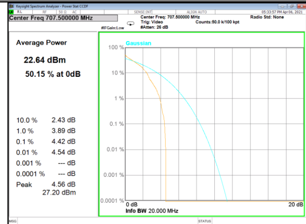
Band 12_1_QPSK_Middle
