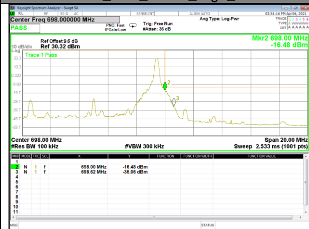
Band71_10M_QPSK_High_1-RB
