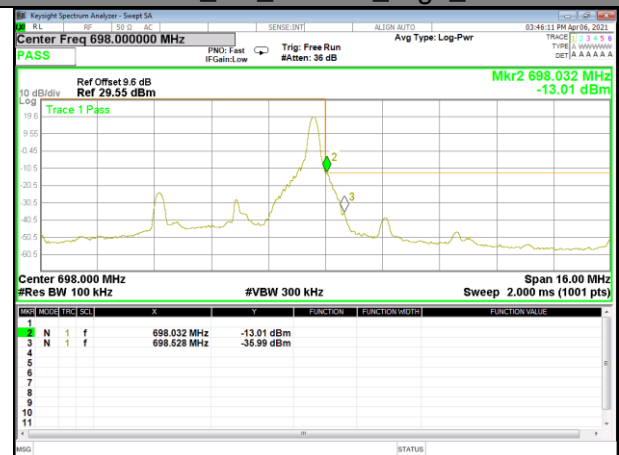
Band71_5M_16QAM_High_1-RB
