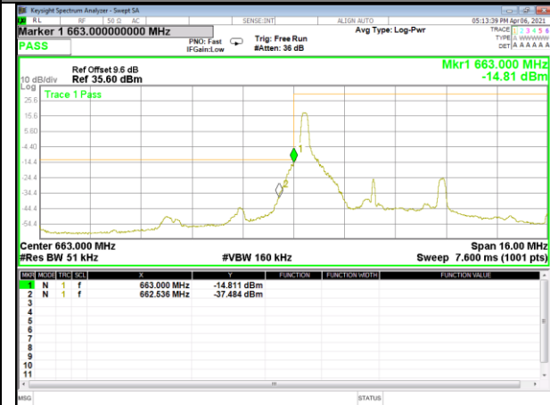
Band71_5M_QPSK_Low_Full-RB
