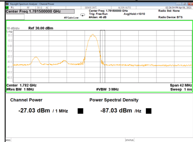
Band66_15M_16QAM_High_1-RB
