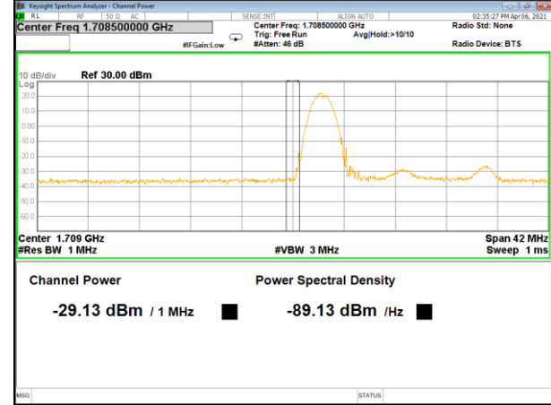
Band66_15M_16QAM_Low_Full-RB
