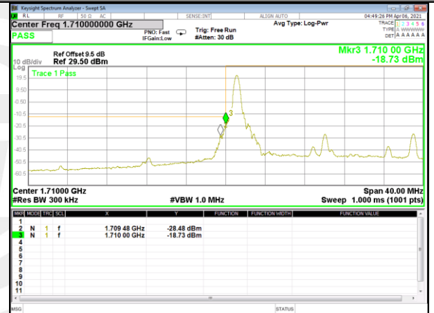
Band 66_20M_QPSK_Low_Full-RB
