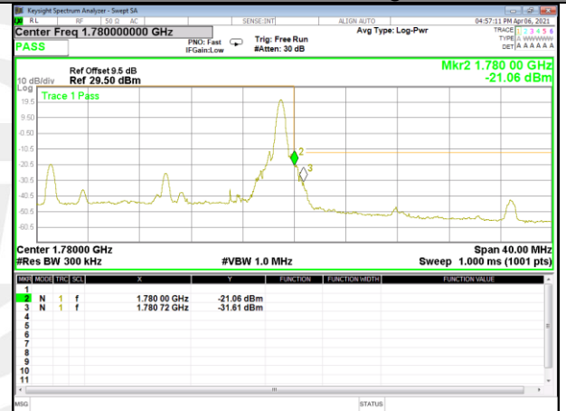
Band 66_20M_16QAM_High_Full-RB
