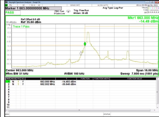
Band71_5M_16QAM_Low_Full-RB
