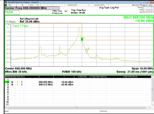
Band 71_5M_QPSK_High_Full-RB
