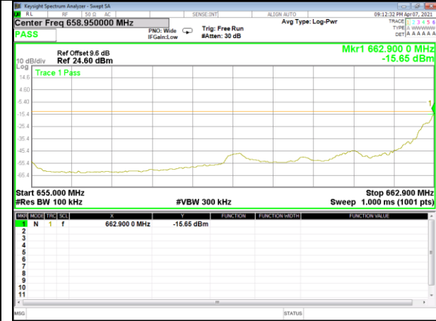
Band71_5M_QPSK_Low_1-RB
