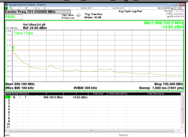
Band 71_5M_QPSK_High_1-RB
