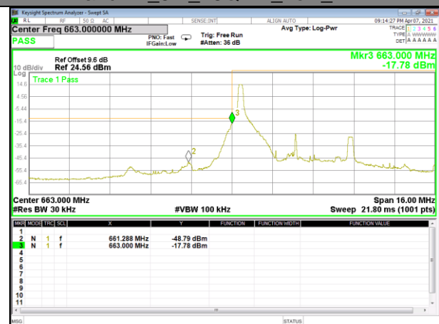
Band 71_5M_16QAM_Low_1-RB
