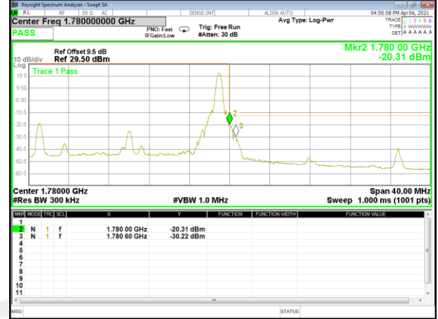
Band 66_20M_QPSK_High_Full-RB
