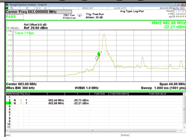
Band71_20M_16QAM_Low_1-RB
