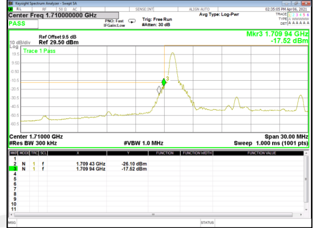
Band66_15M_16QAM_Low_Full-RB
