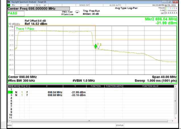
Band71_20M_16QAM_High_Full-RB
