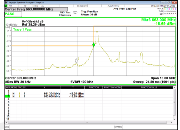
Band 71_5M_QPSK_Low_Full-RB
