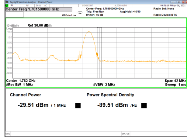
Band 66_20M_QPSK_High_Full-RB
