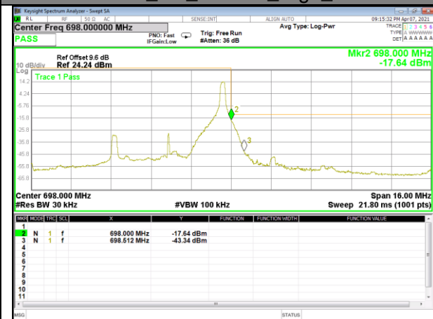
Band 71_5M_16QAM_High_1-RB
