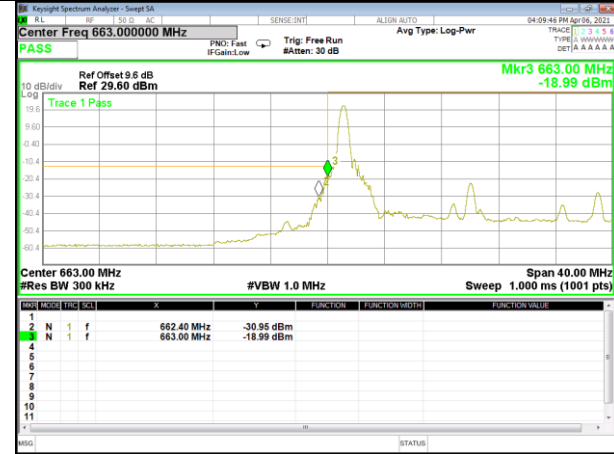
Band71_20M_QPSK_High_1-RB
