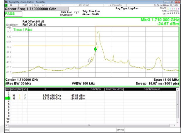
Band66_3M_16QAM_Low_Full-RB
