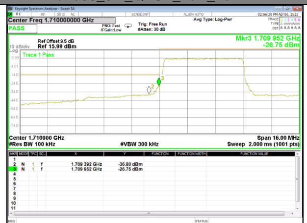
Band66_5M_QPSK_Low_Full-RB
