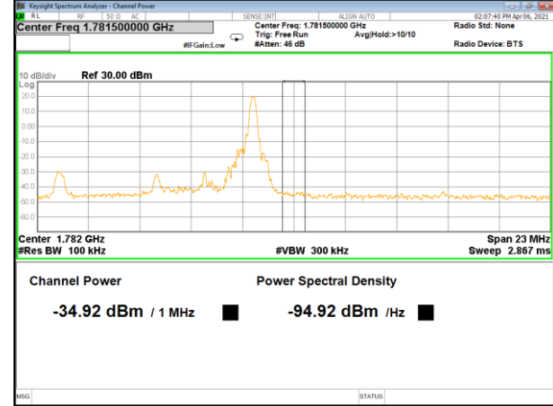
Band66_5M_QPSK_High_Full-RB
