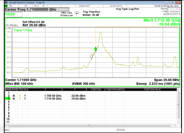
Band 66_10M_QPSK_Low_Full-RB
