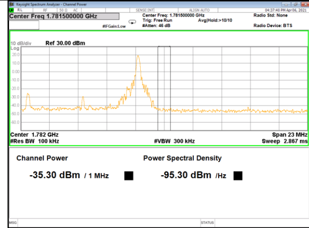
Band 66_10M_16QAM_High_Full-RB
