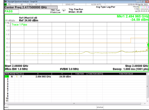
Band 41_20M_16QAM_Low_Full-RB
