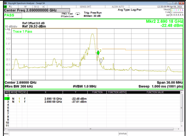
Band 41_15M_QPSK_High_1-RB
