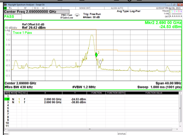
Band 41_20M_16QAM_High_1-RB
