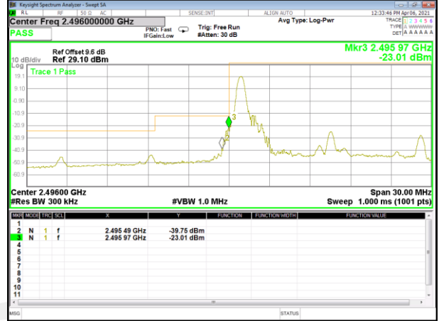
Band 41_15M_QPSK_Low_Full-RB
