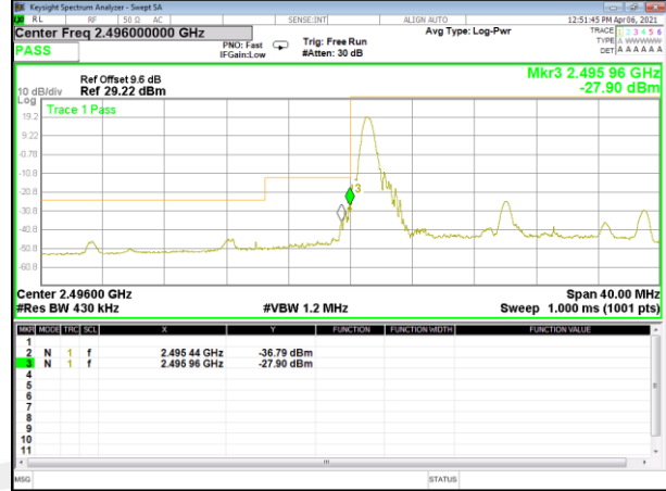
Band 41_20M_16QAM_Low_Full-RB
