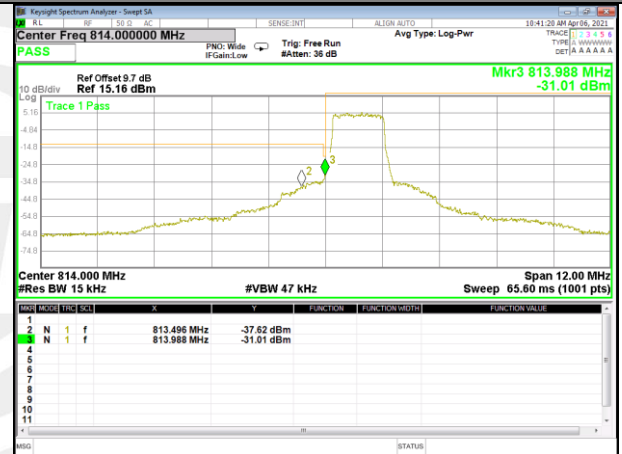
Band 26_1.4M_QPSK_High_1-RB
