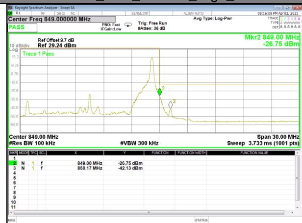
Band 26_15M_16QAM_High_1-RB
