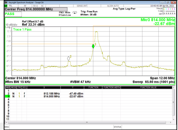
Band 26_1.4M_QPSK_Low_Full-RB
