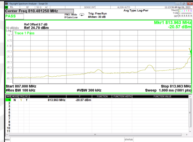
Band 26_5M_16QAM_Low_Full-RB
