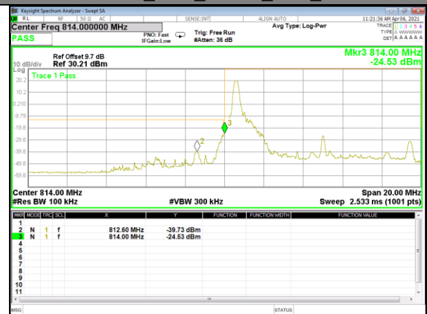
Band 26_10M_QPSK_Low_1-RB
