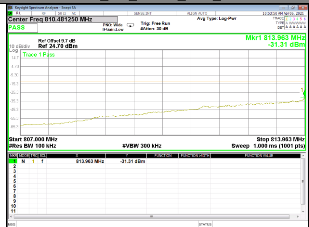
Band 26_3M_QPSK_Low_Full-RB
