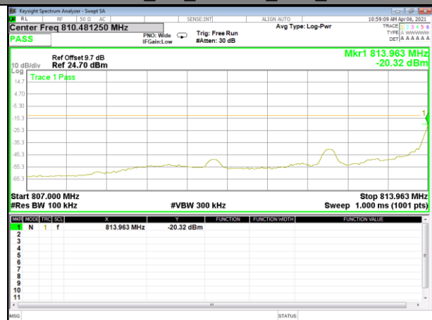
Band 26_3M_16QAM_Low_1-RB
