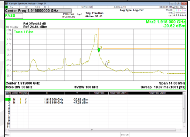
Band 25_3M_QPSK_High_Full-RB
