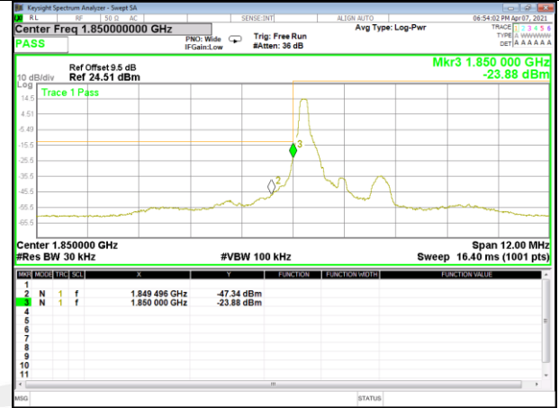
Band 25_1.4M_QPSK_Low_Full-RB
