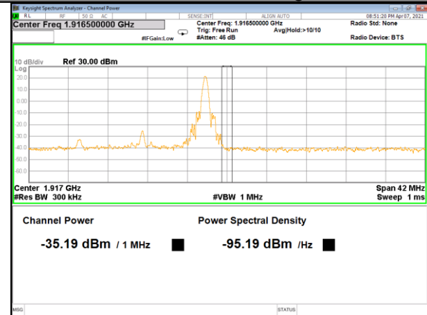
Band 25_15M_QPSK_High_Full-RB
