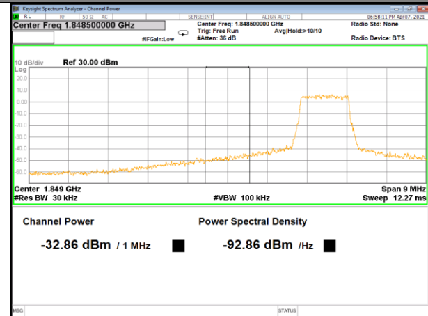
Band 25_1.4M_16QAM_Low_Full-RB
