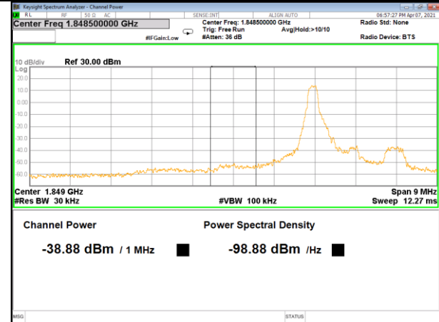
Band 25_1.4M_16QAM_Low_Full-RB
