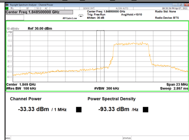
Band 25_5M_QPSK_Low_Full-RB
