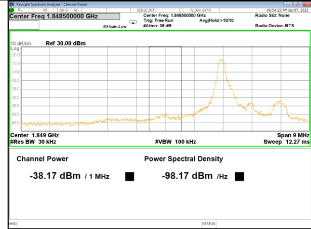
Band 25_1.4M_QPSK_Low_Full-RB
