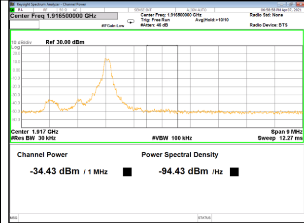
Band 25_1.4M_16QAM_High_Full-RB
