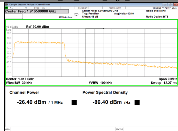
Band 25_3M_QPSK_High_Full-RB
