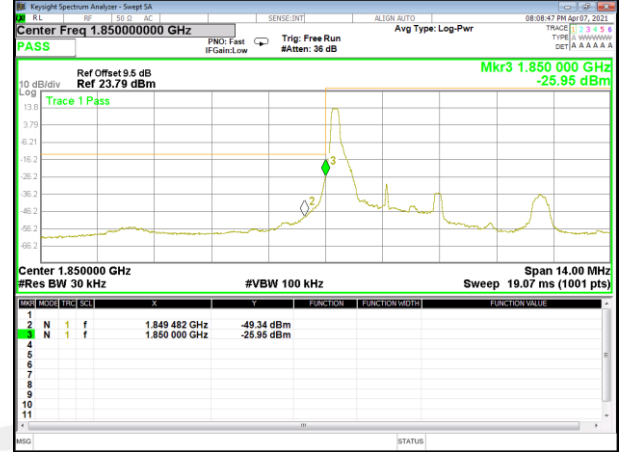
Band 25_3M_16QAM_Low_Full-RB
