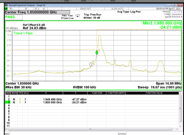
Band 25_3M_QPSK_Low_1-RB
