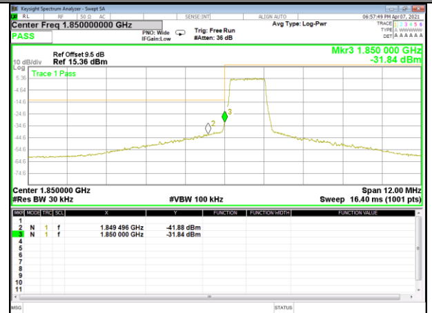
Band 25_1.4M_16QAM_Low_Full-RB
