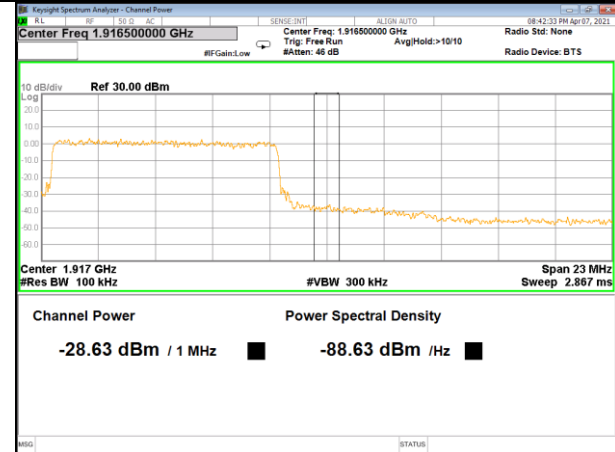
Band 25_15M_QPSK_Low_1-RB
