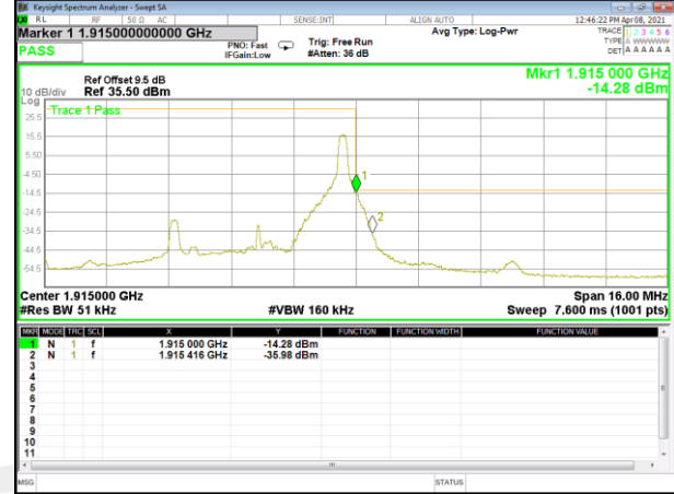
Band 25_5M_QPSK_High_Full-RB
