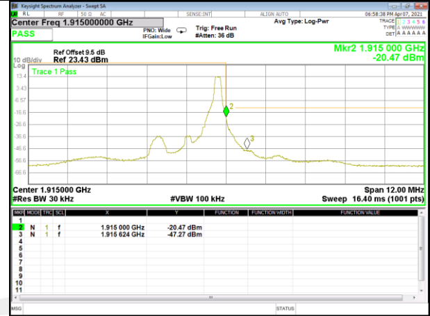
Band 25_1.4M_16QAM_High_Full-RB
