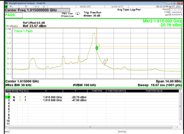
Band 25_3M_16QAM_High_1-RB
