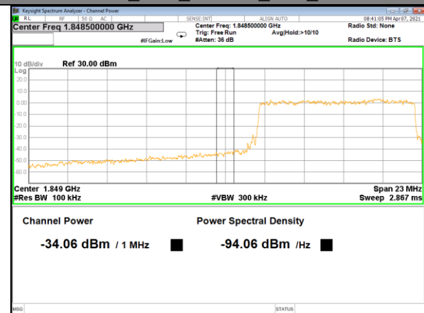
Band 25_10M_16QAM_Low_Full-RB
