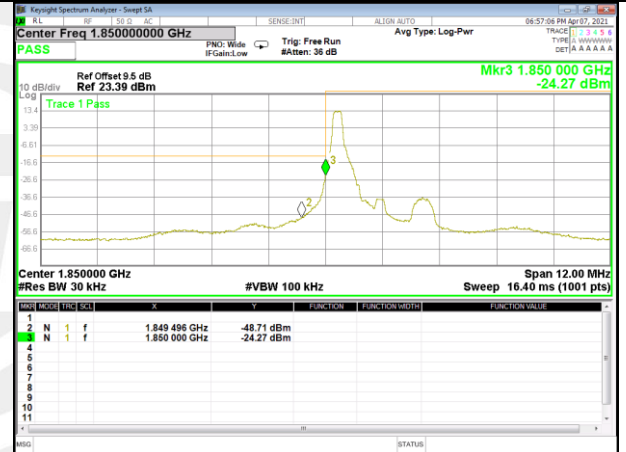
Band 25_1.4M_16QAM_Low_Full-RB
