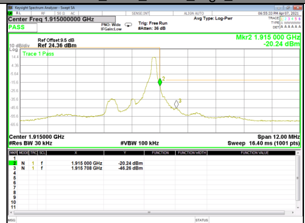
Band 25_1.4M_QPSK_High_1-RB
