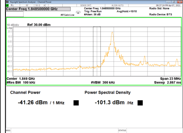
Band 25_10M_QPSK_Low_Full-RB
