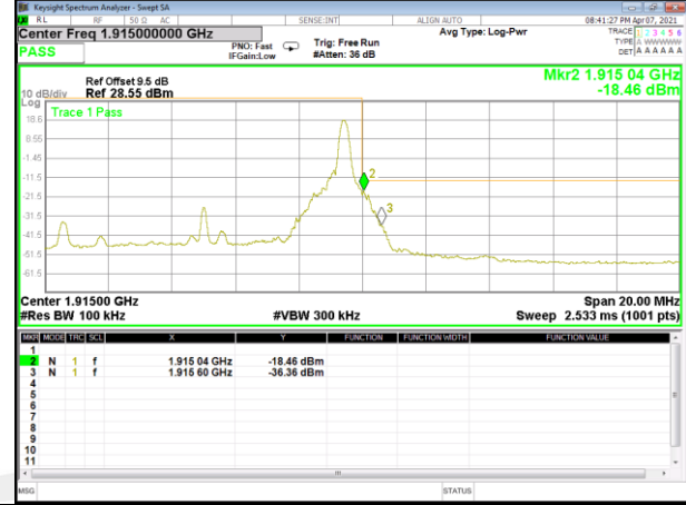
Band 25_10M_16QAM_High_Full-RB
