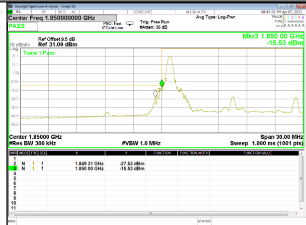
Band 25_15M_QPSK_Low_1-RB
