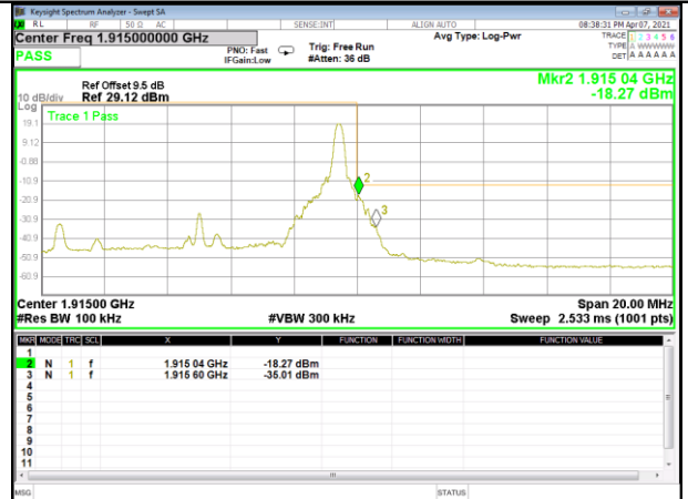
Band 25_10M_QPSK_High_1-RB
