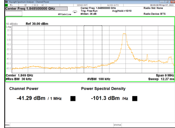
Band 25_3M_16QAM_Low_Full-RB
