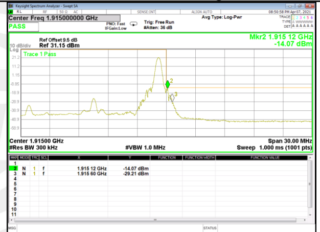
Band 25_15M_QPSK_High_Full-RB
