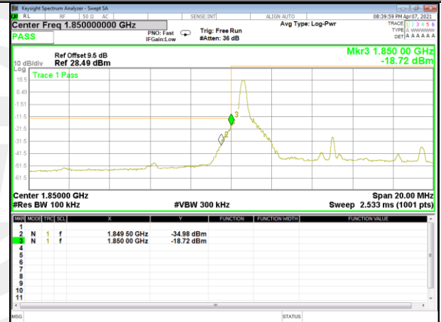
Band 25_10M_16QAM_Low_Full-RB
