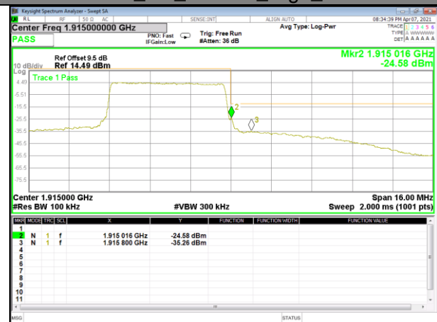
Band 25_5M_16QAM_High_Full-RB
