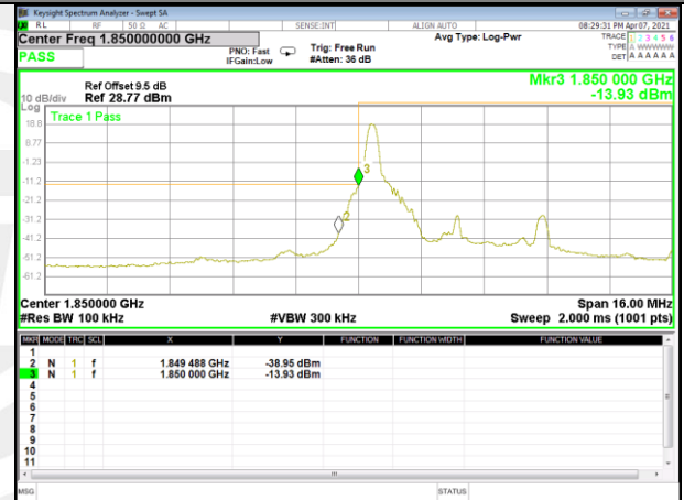
Band 25_5M_QPSK_Low_Full-RB
