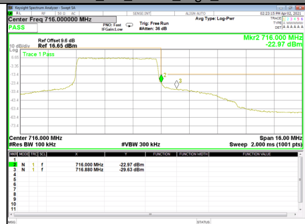
Band12_5M_QPSK_High_Full-RB
