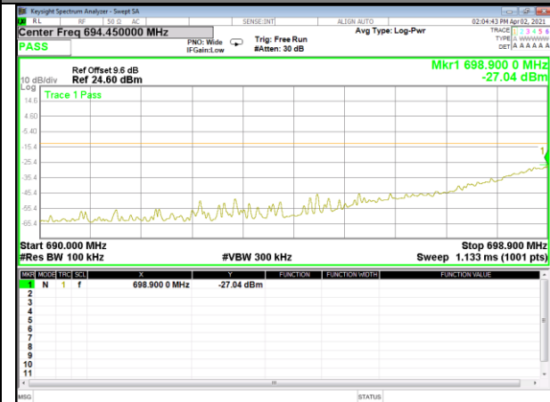
Band12_1.4M_16QAM_Low_Full-RB
