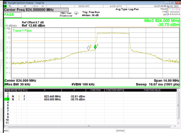
Band 5_3M_16QAM_High_1-RB
