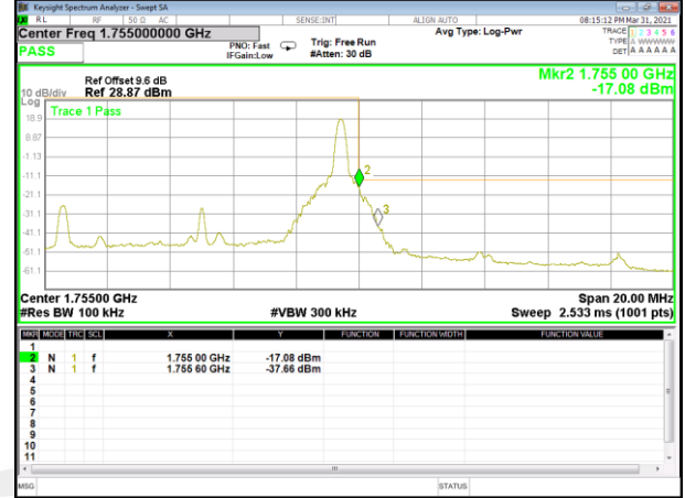
Band 4_10M_16QAM_High_Full-RB
