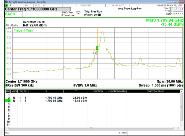
Band 4_15M_16QAM_Low_Full-RB
