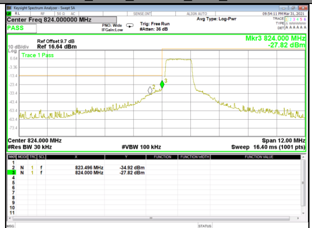
Band 5_1.4M_16QAM_Low_Full-RB
