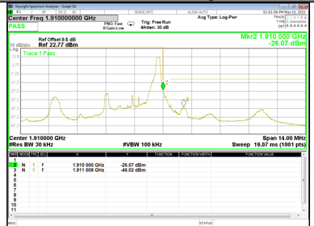
Band 2_3M_16QAM_High_1-RB
