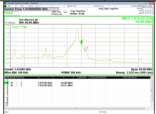
Band 2_10M_QPSK_High_1-RB
