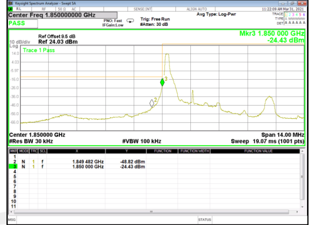
Band 2_3M_16QAM_Low_Full-RB
