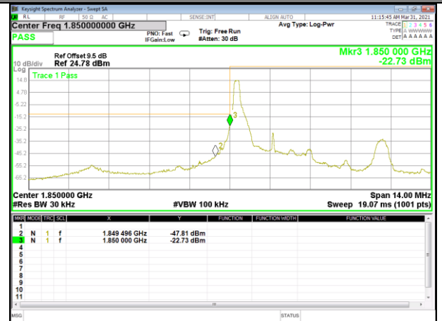
Band 2_3M_QPSK_Low_1-RB
