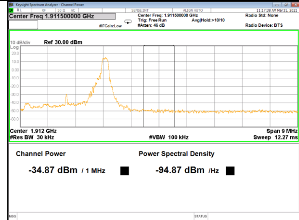
Band 2_3M_QPSK_High_Full-RB
