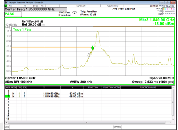
Band 2_10M_QPSK_Low_Full-RB
