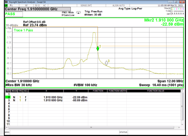
Band 2_1.4M_16QAM_High_Full-RB
