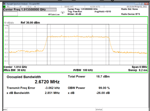
Band25_3M_16QAM_High
