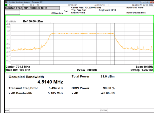
Band12_5M_QPSK_Middle
