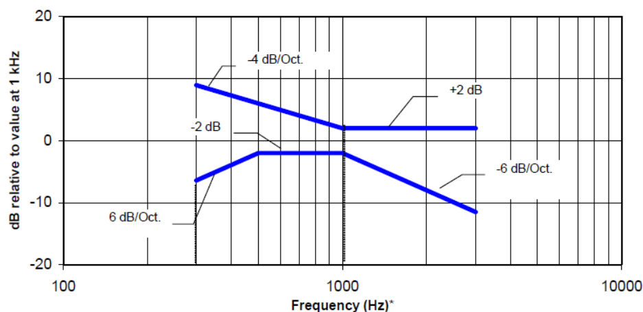
Fig 2.1 Magnetic field frequency response for WDs with field strength \leq -15 dB (A/m) at 1 kHz
