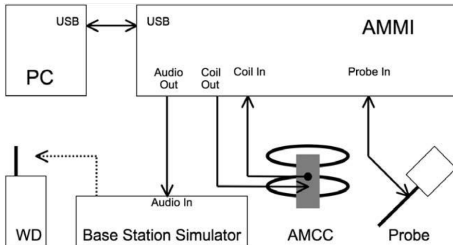
Fig 5.1 SPEAG T-Coil System Configurations
