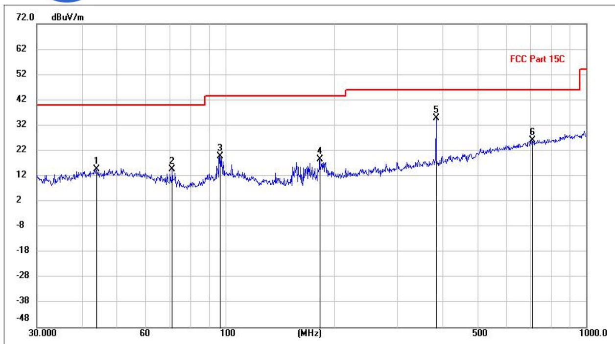
(802.11b _2467MHz, Antenna Horizontal, 30MHz to 1GHz)
