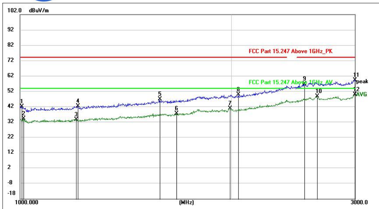
(802.11b _2472MHz, Antenna Vertical , 1GHz to 3GHz)
