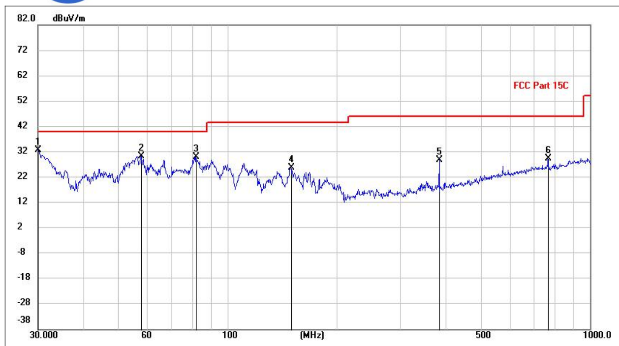
(802.11n_20M_2467MHz, Antenna Vertical, 30MHz to 1GHz)
