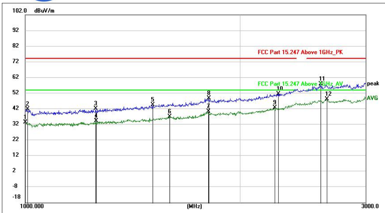
(802.11g _2467MHz, Antenna Vertical , 1GHz to 3GHz)
