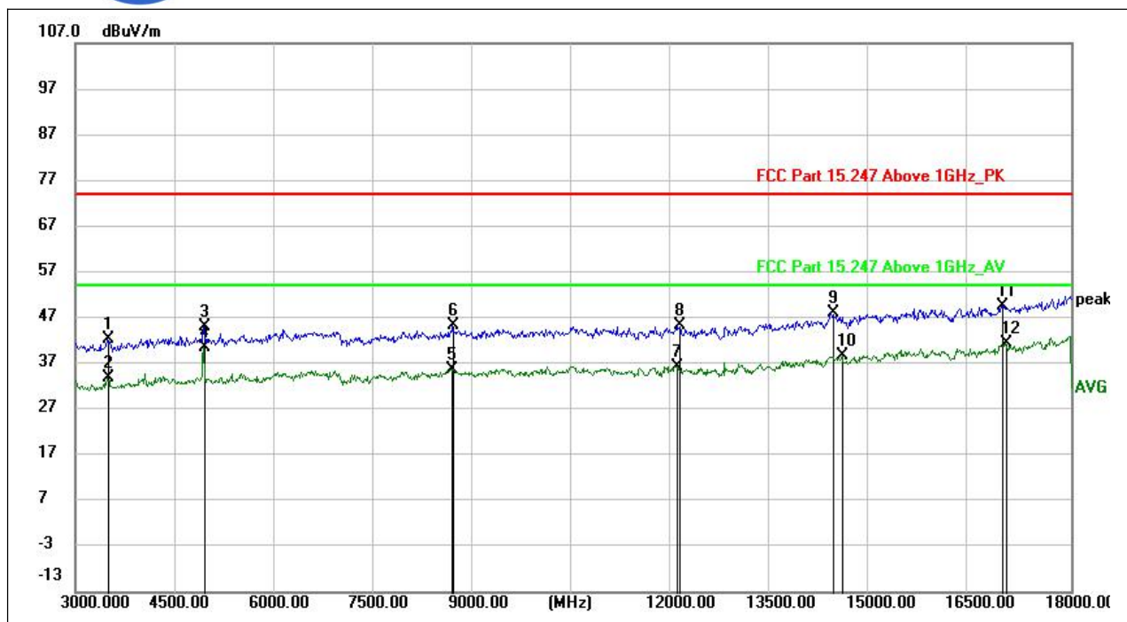
(802.11b _2472MHz, Antenna Horizontal, 3GHz to 18GHz)
