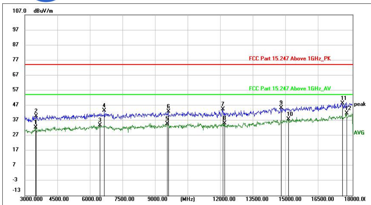
(802.11g _2472MHz, Antenna Horizontal, 3GHz to 18GHz)
