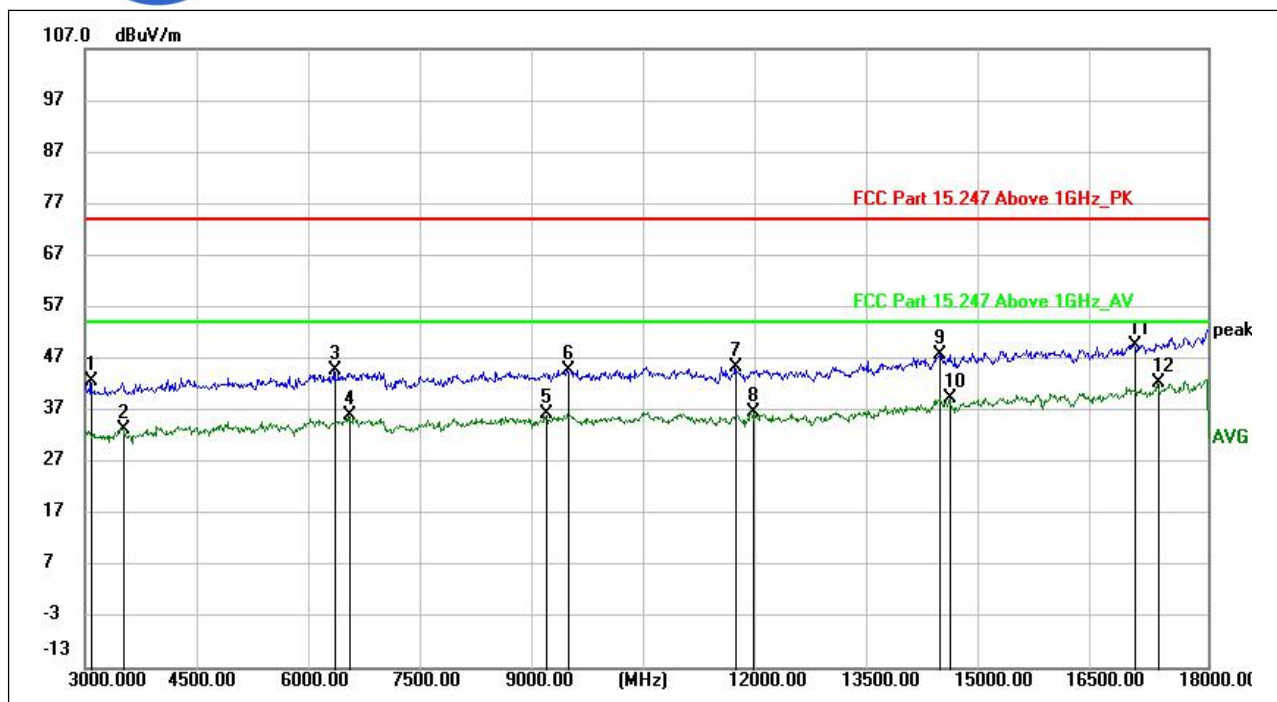
(802.11g _2467MHz, Antenna Vertical, 3GHz to 18GHz)
