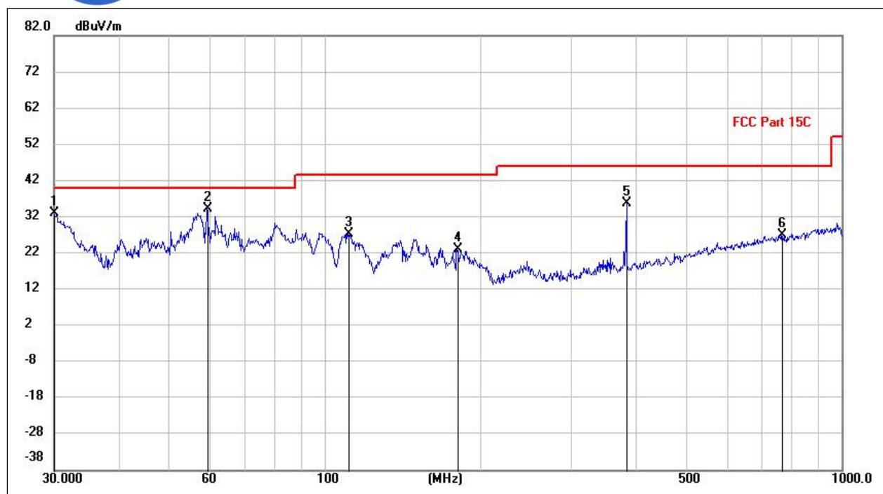
(802.11g _2472MHz, Antenna Vertical, 30MHz to 1GHz)
