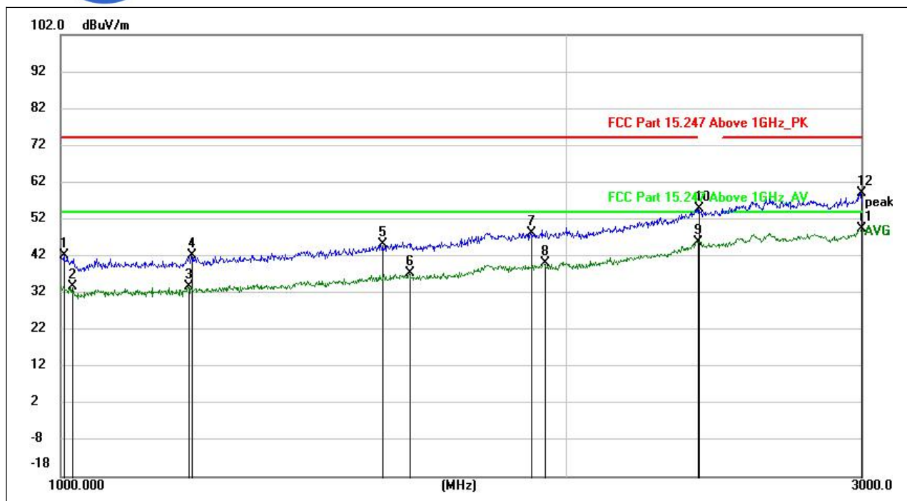
(802.11b _2467MHz, Antenna Vertical , 1GHz to 3GHz)
