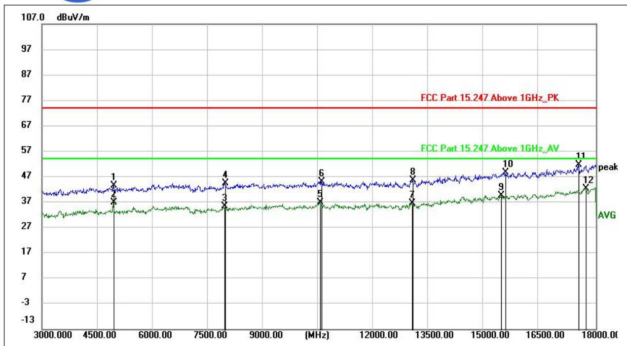
(802.11b_2472MHz, Antenna Vertical, 3GHz to 18GHz)
