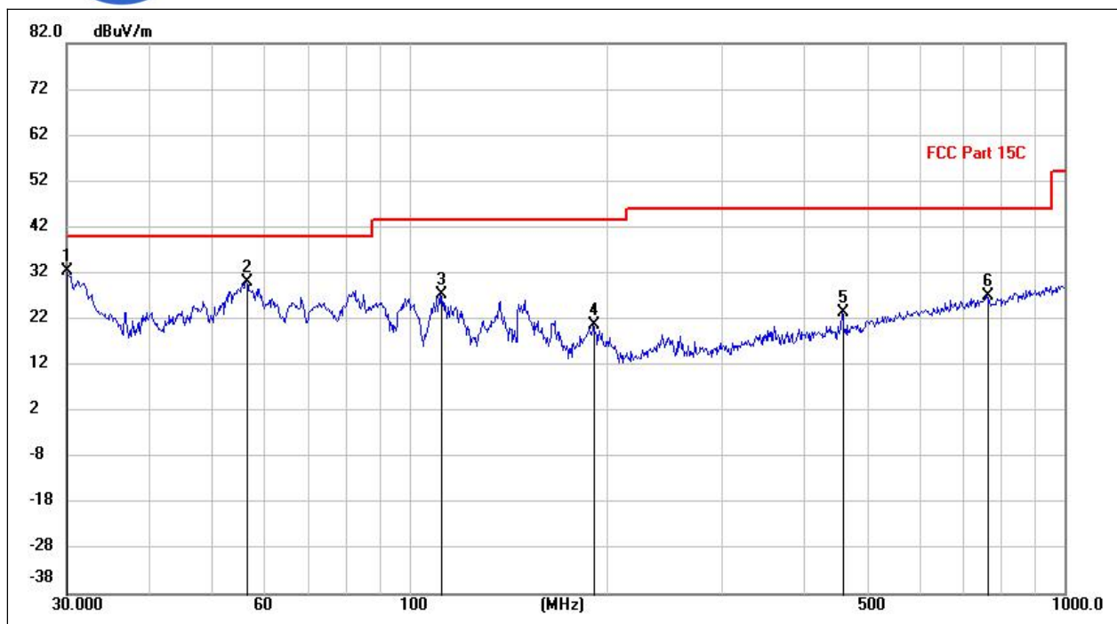
(802.11b _2467MHz, Antenna Vertical, 30MHz to 1GHz)
