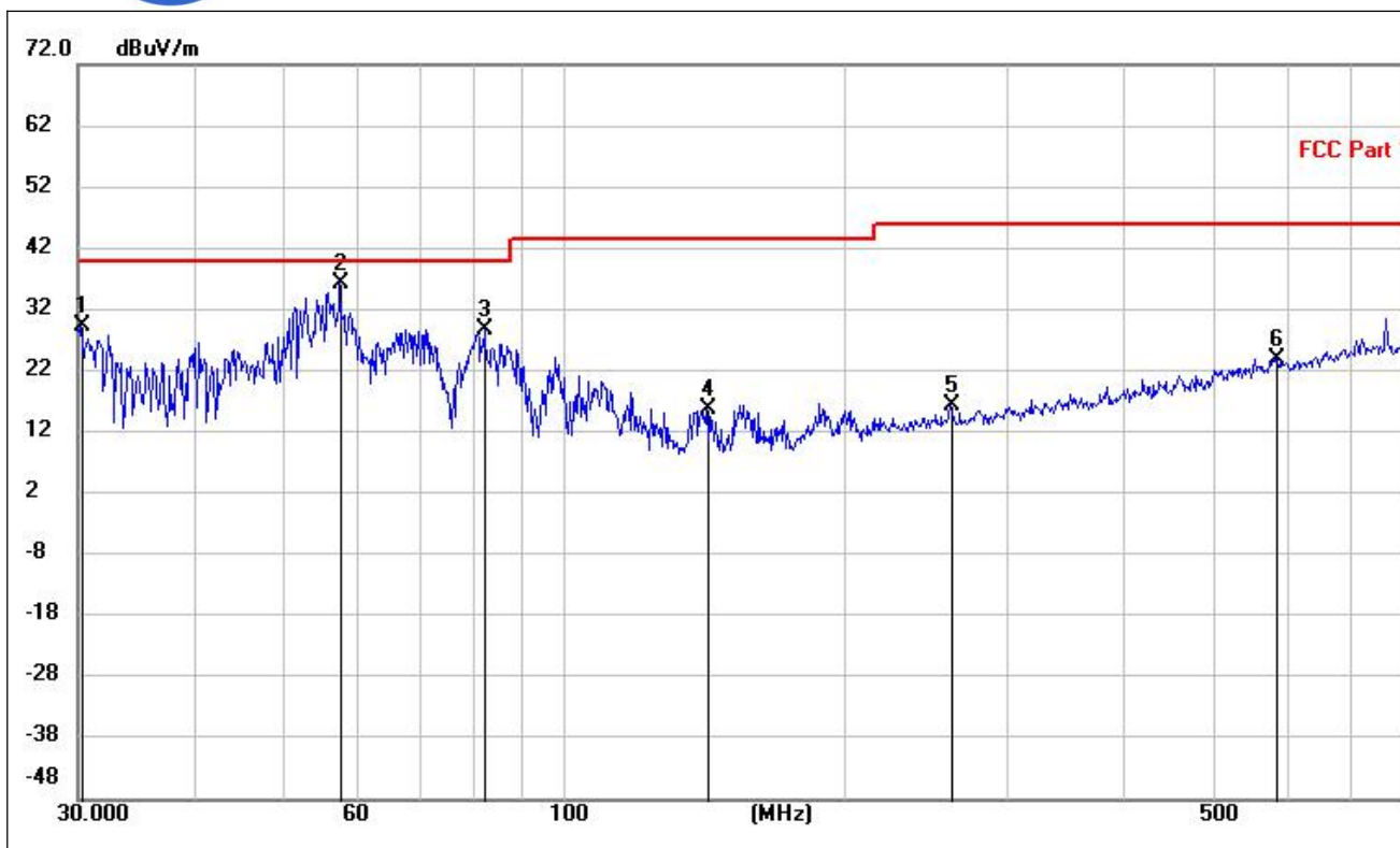
(802.11b _2437MHz, Antenna Vertical, 30MHz to 1GHz)
