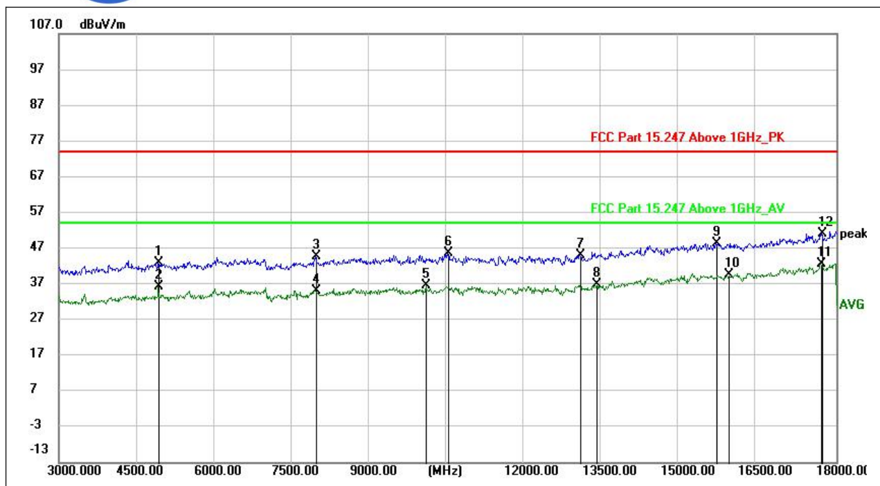
(802.11b _2467MHz, Antenna Vertical, 3GHz to 18GHz)
