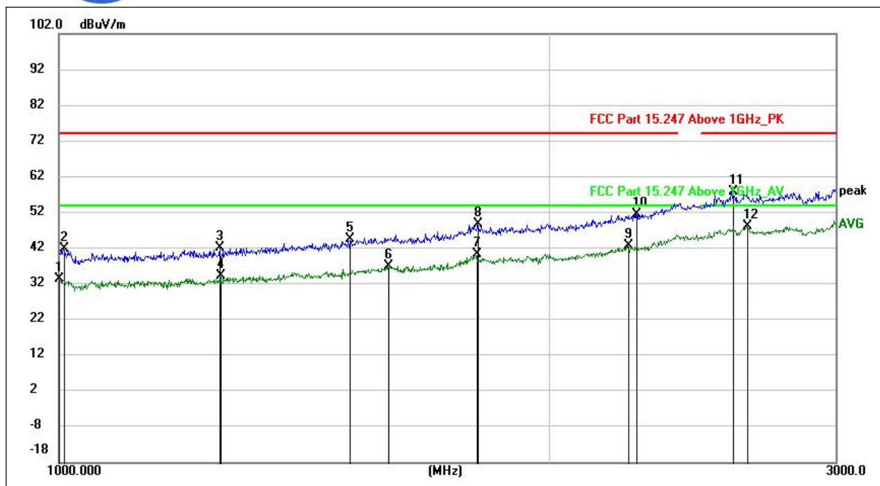
(802.11g _2472MHz, Antenna Vertical , 1GHz to 3GHz)
