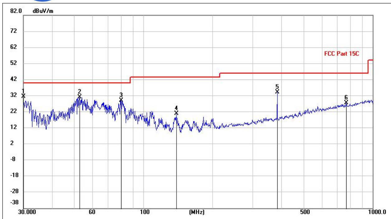
(802.11n_20M_2472MHz, Antenna Vertical, 30MHz to 1GHz)
