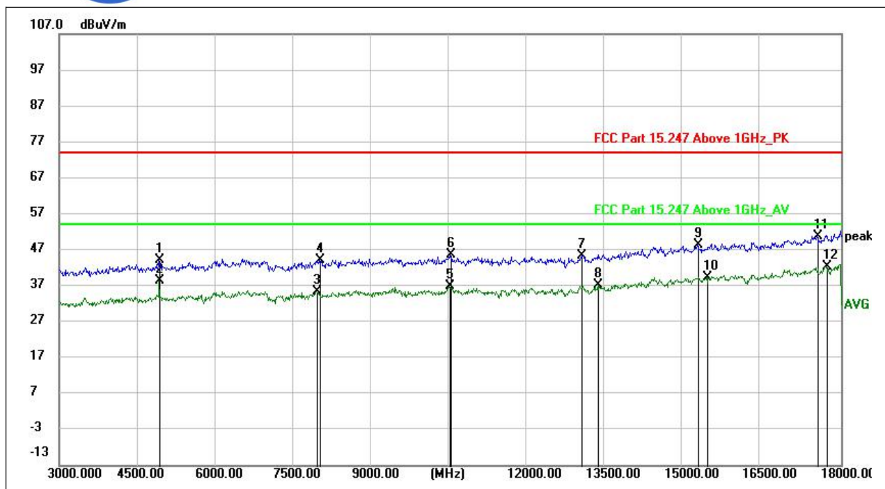
(802.11b _2467MHz, Antenna Horizontal, 3GHz to 18GHz)
