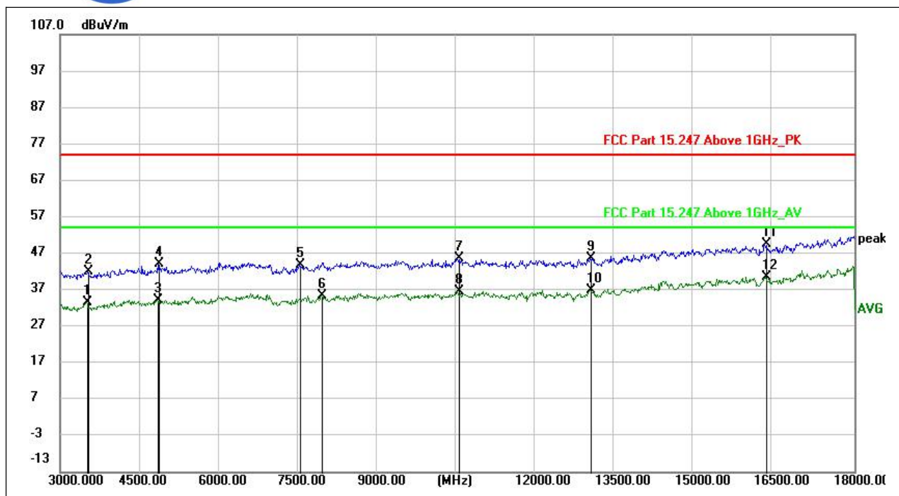
(802.11g _2472MHz, Antenna Vertical, 3GHz to 18GHz)
