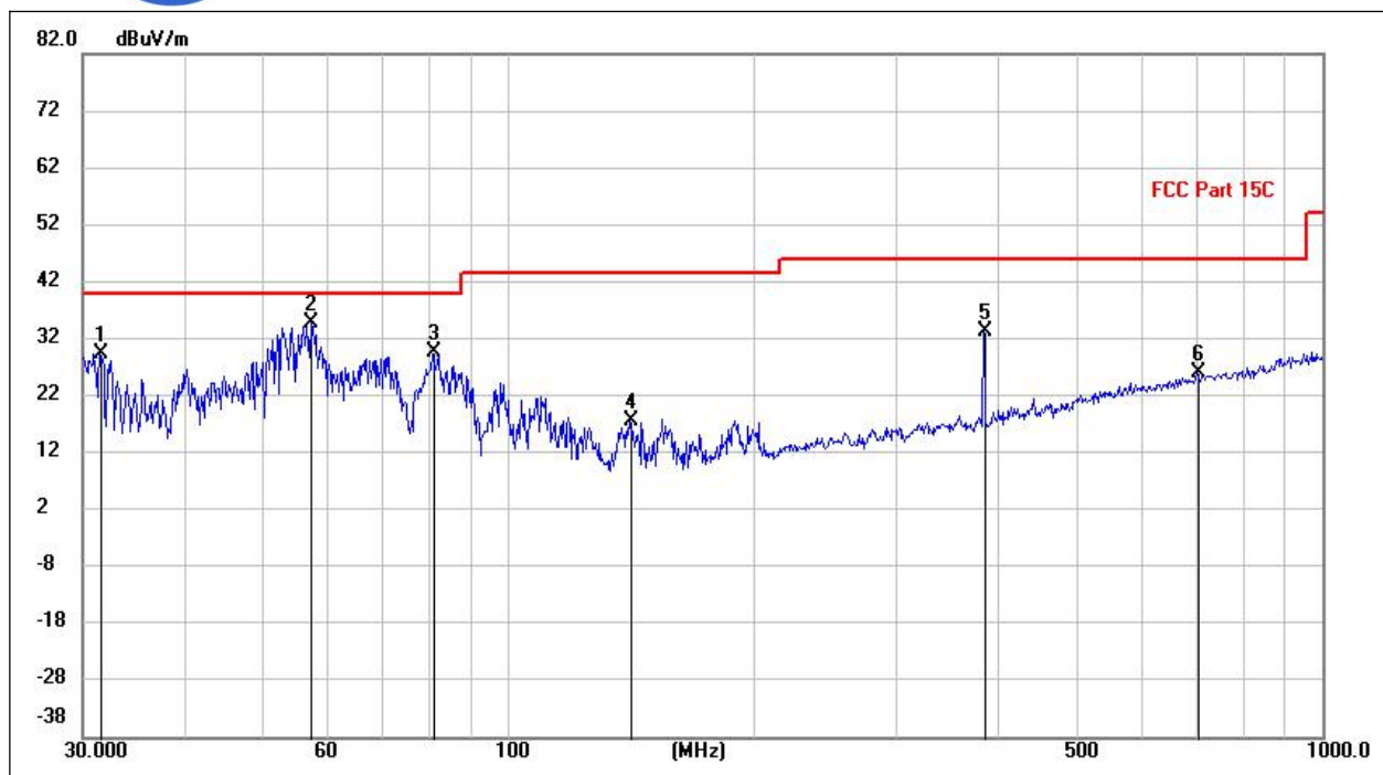
(802.11b _2472MHz, Antenna Vertical, 30MHz to 1GHz)
