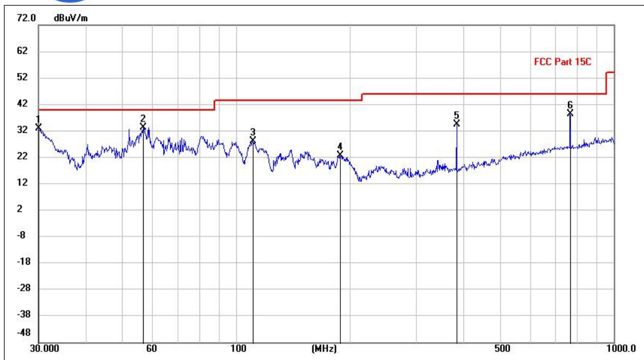
(802.11g _2467MHz, Antenna Vertical, 30MHz to 1GHz)
