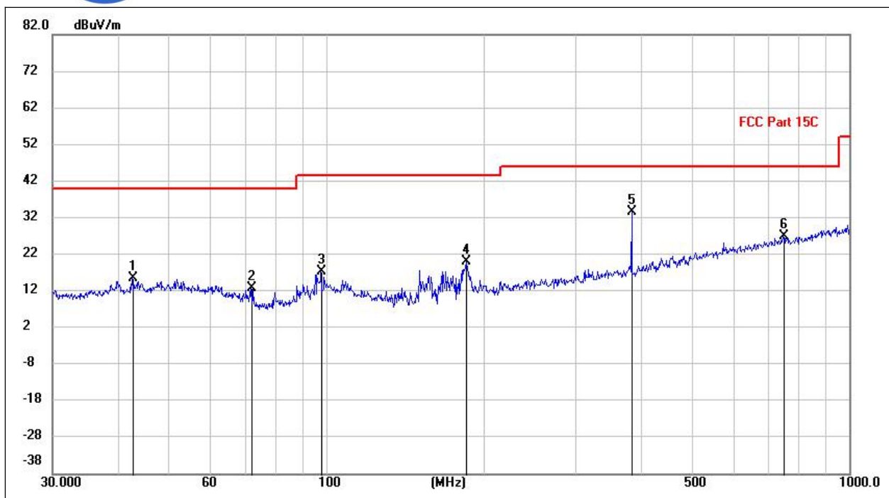
(802.11b _2472MHz, Antenna Horizontal, 30MHz to 1GHz)
