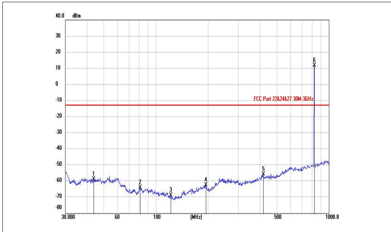
(1XEVD0 Rev 0 BC 0 _ CH 1013 _ 30MHz to 1GHz _ Vertical)
