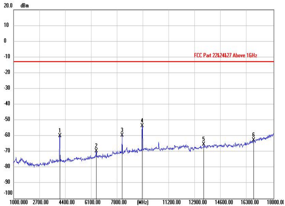
(WCDMA Band V_ 1GHz to 18GHz _ Middle Channel _ Vertical)
