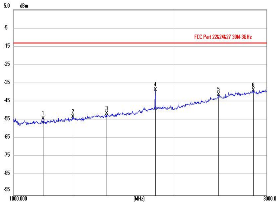
(EDGE 1900MHz _ 1GHz to 3GHz_ 512 Channel _ Vertical)
