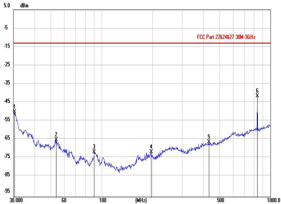
(EDGE 850MHz _ 30MHz to 1GHz_ 190 Channel _ Vertical)
