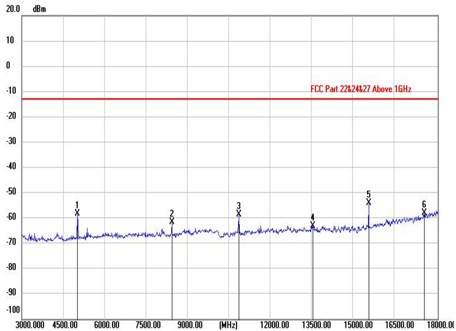
(EDGE 1900MHz _ 3GHz to 18GHz _ 810 Channel_ Horizontal)
