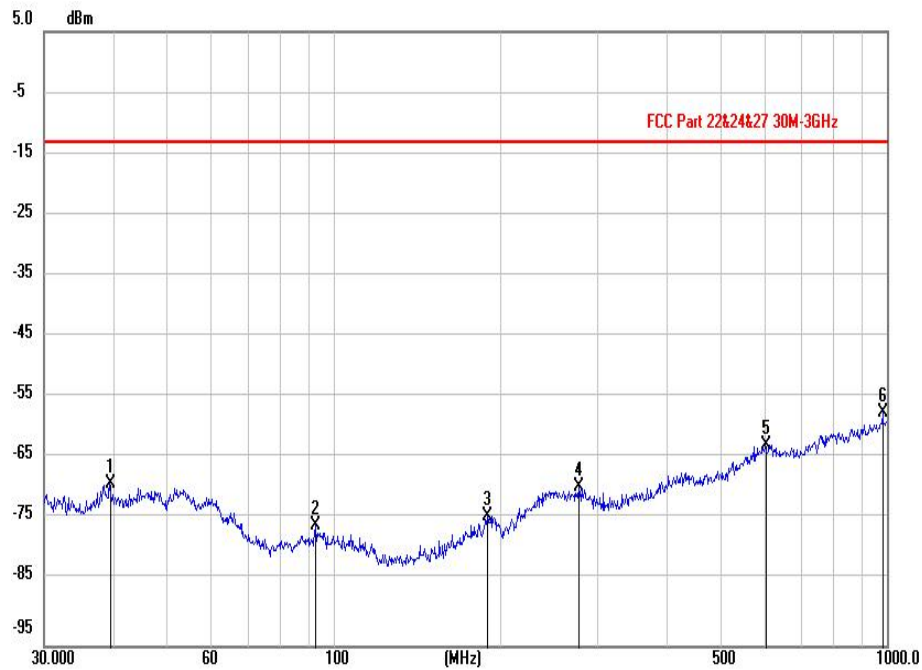
(EDGE 1900MHz _ 30MHz to 1GHz _ 810 Channel _ Horizontal)
