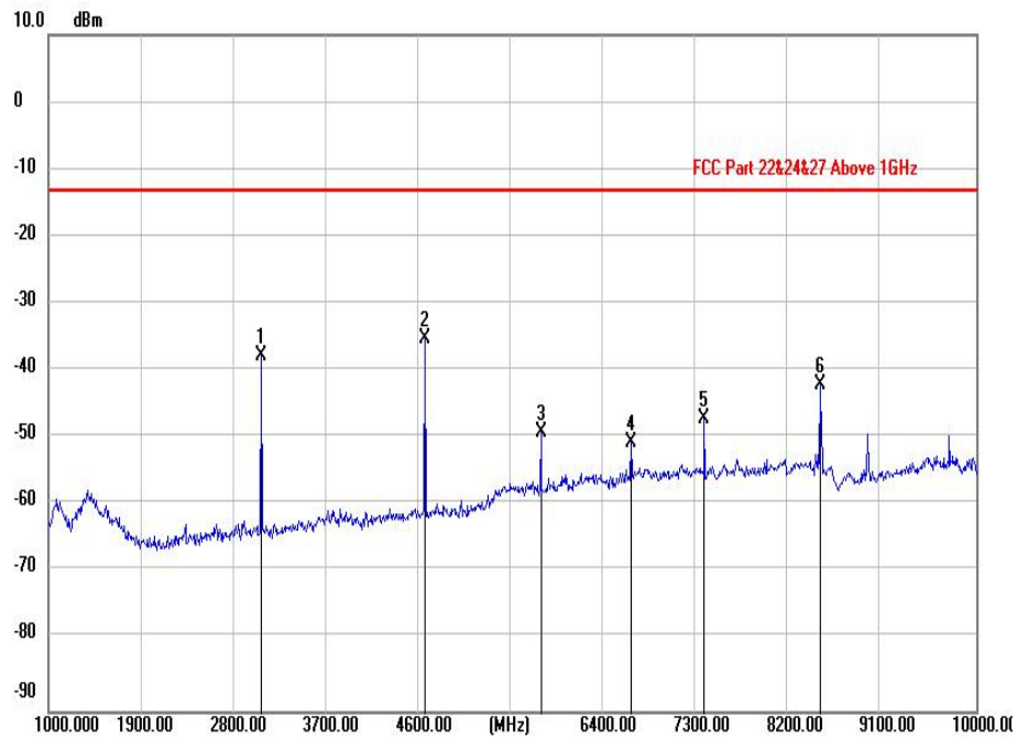
(EDGE 850MHz _ 1GHz to 10GHz_ 251 Channel _ Vertical)
