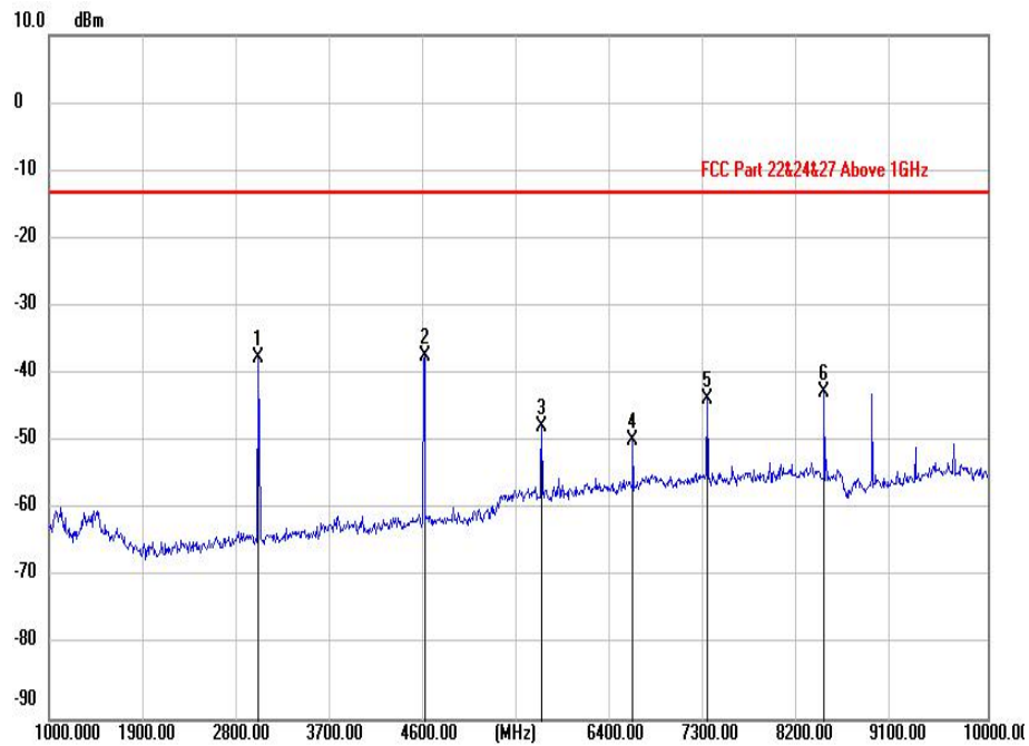
(EDGE 850MHz _ 1GHz to 10GHz_ 190 Channel _ Vertical)
