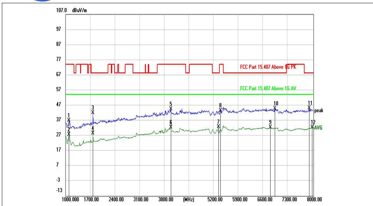
(802.11ac_5310MHz, Antenna Horizontal, 1GHz to 8GHz)
