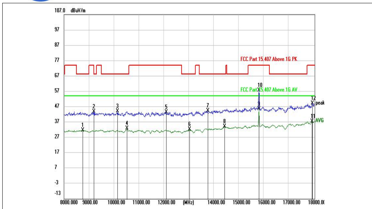
(802.11ac _5260MHz, Antenna Horizontal, 8GHz to 18GHz)
