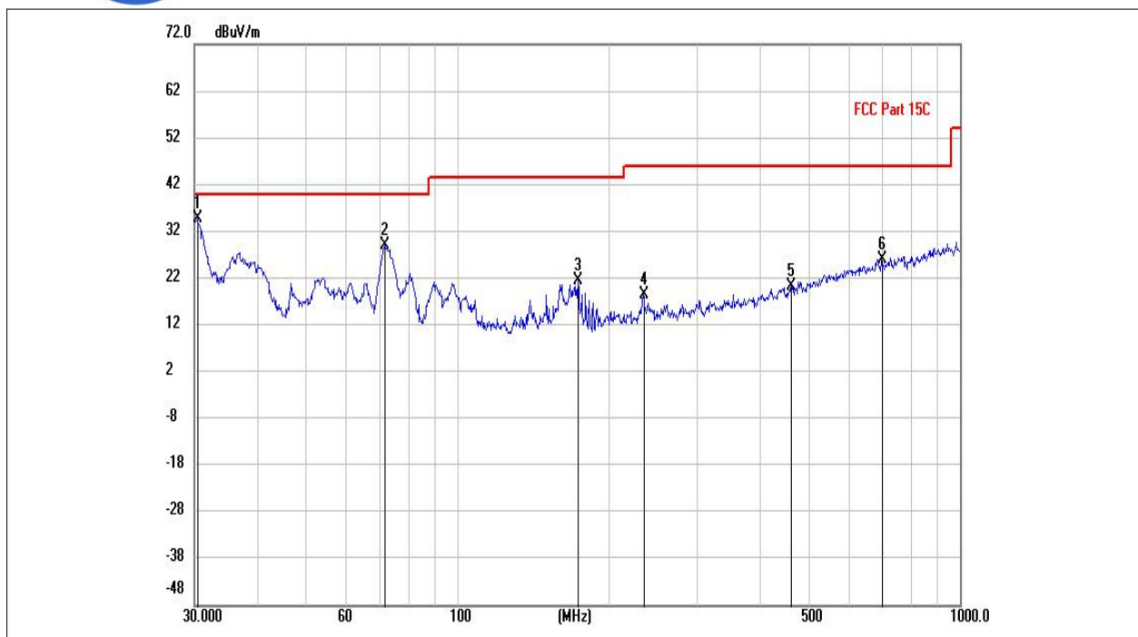
(802.11a _5825MHz, Antenna Vertical, 30MHz to 1GHz)
