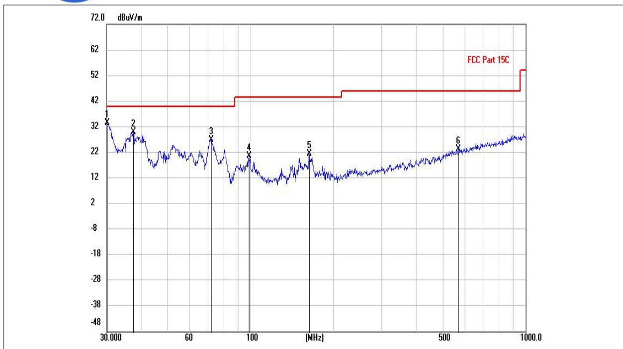
(802.11n _5745MHz, Antenna Vertical, 30MHz to 1GHz)
