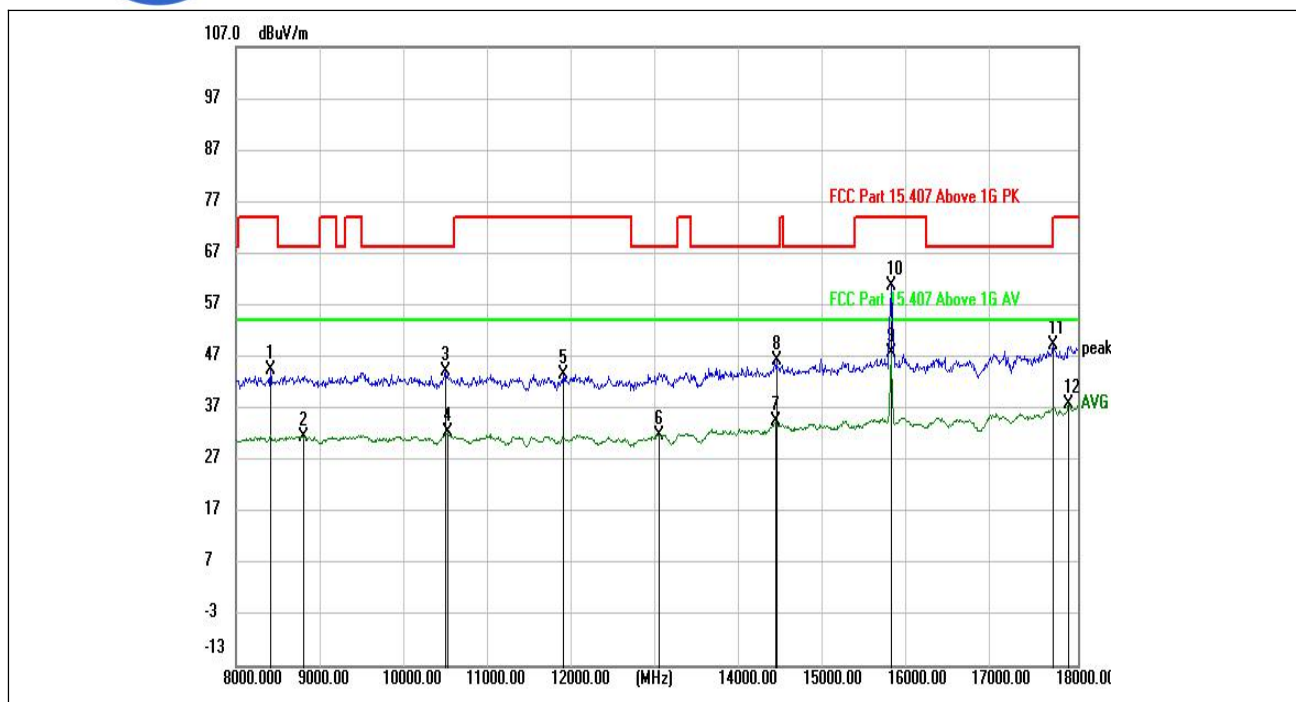
(802.11n_5260MHz, Antenna Vertical, 8GHz to 18GHz)
