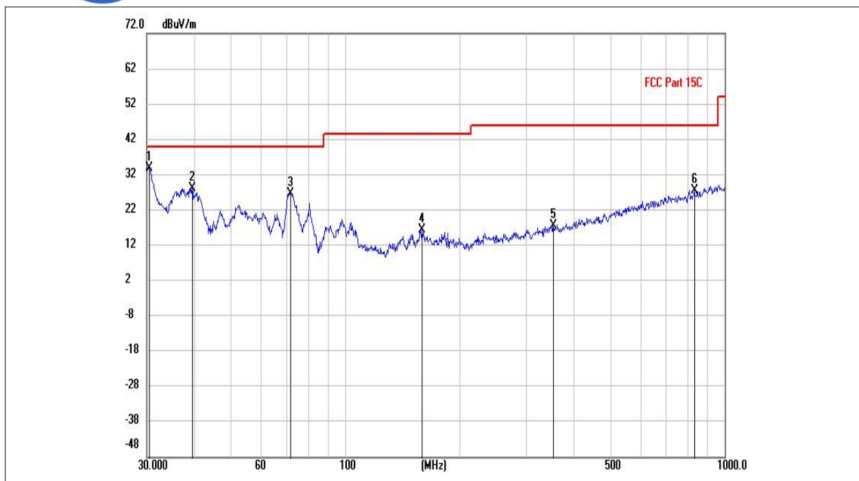
(802.11n _5300MHz, Antenna Vertical, 30MHz to 1GHz)
