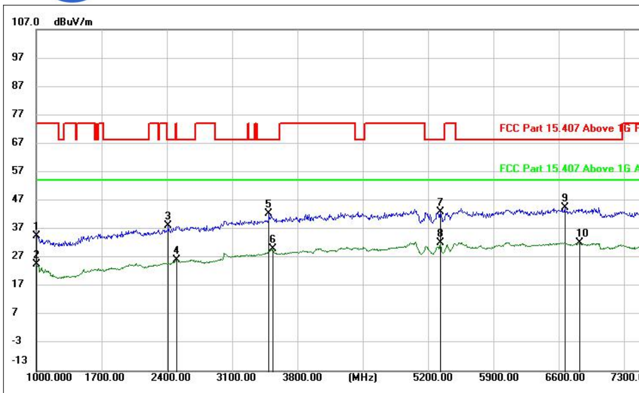
(802.11a _5300MHz, Antenna Vertical, 1GHz to 8GHz)
