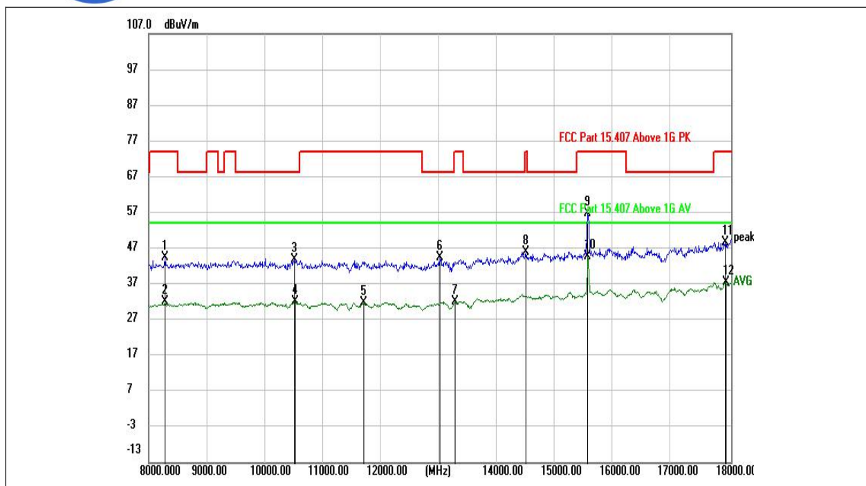
(802.11ac _5180MHz, Antenna Horizontal, 8GHz to 18GHz)
