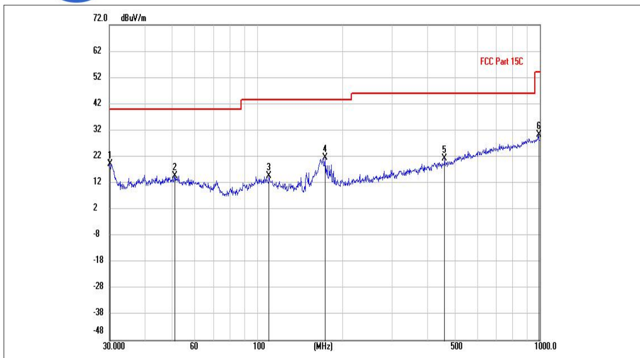
(802.11n_5230MHz, Antenna Vertical, 30MHz to 1GHz)
