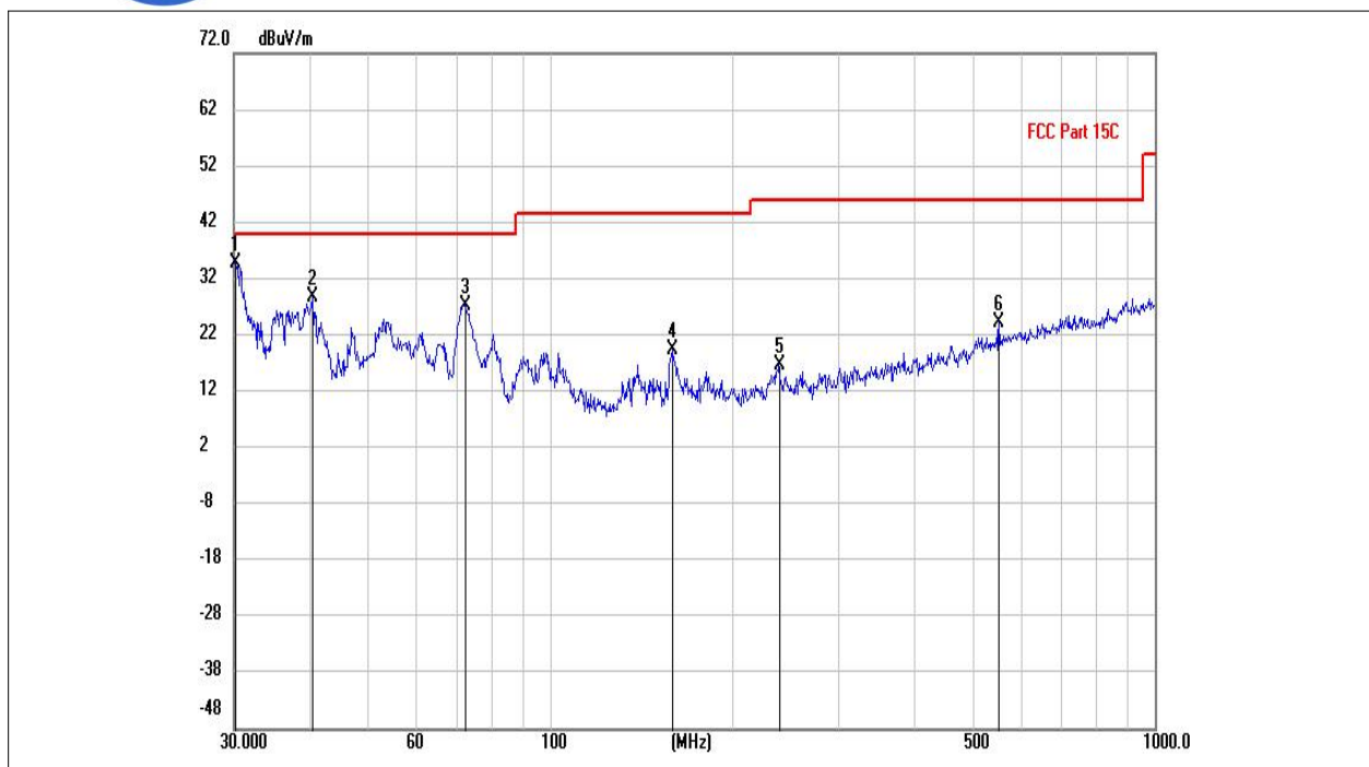
(802.11n_5190MHz, Antenna Vertical, 30MHz to 1GHz)
