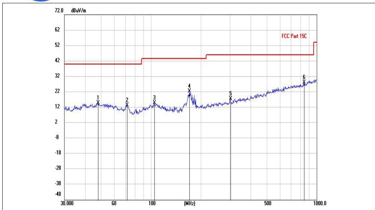
(802.11ac _5220MHz, Antenna Horizontal, 30MHz to 1GHz)
