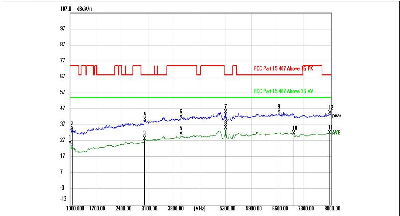
(802.11ac_5180MHz, Antenna Vertical, 1GHz to 8GHz)
