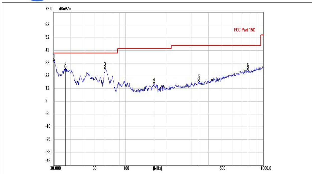
(802.11n _5260MHz, Antenna Vertical, 30MHz to 1GHz)
