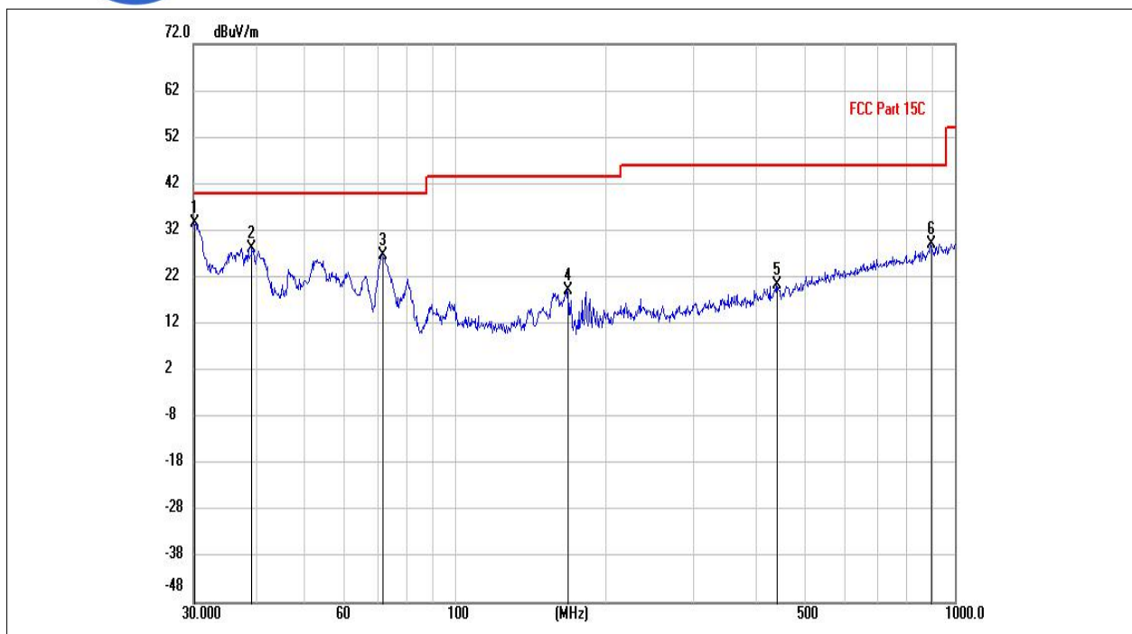
(802.11n_5310MHz, Antenna Vertical, 30MHz to 1GHz)
