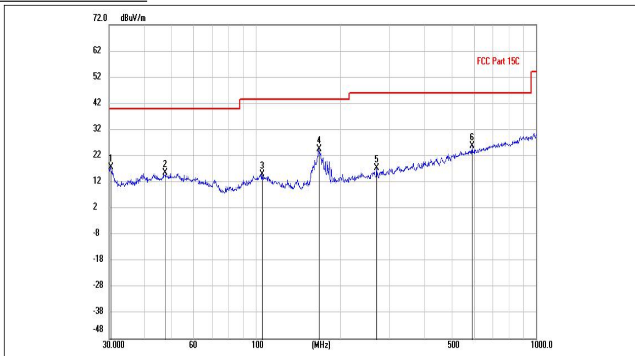
(802.11n _5190MHz, Antenna Horizontal, 30MHz to 1GHz)
