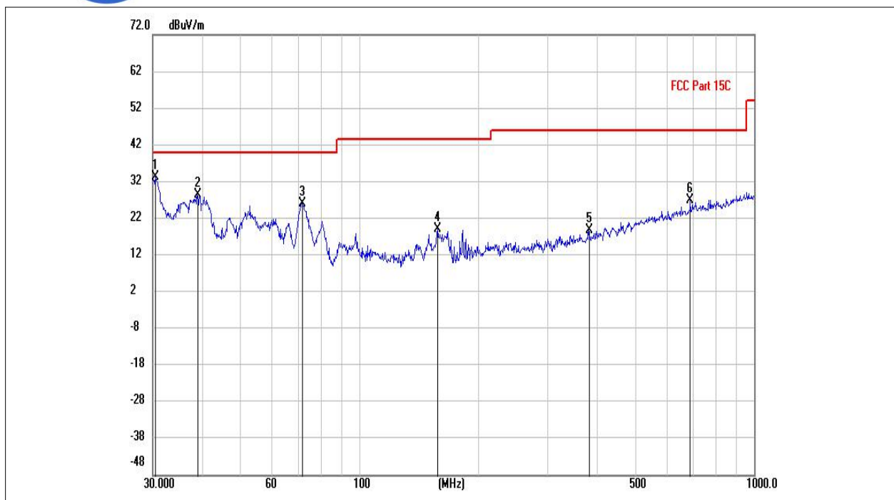
(802.11n_5755MHz, Antenna Vertical, 30MHz to 1GHz)
