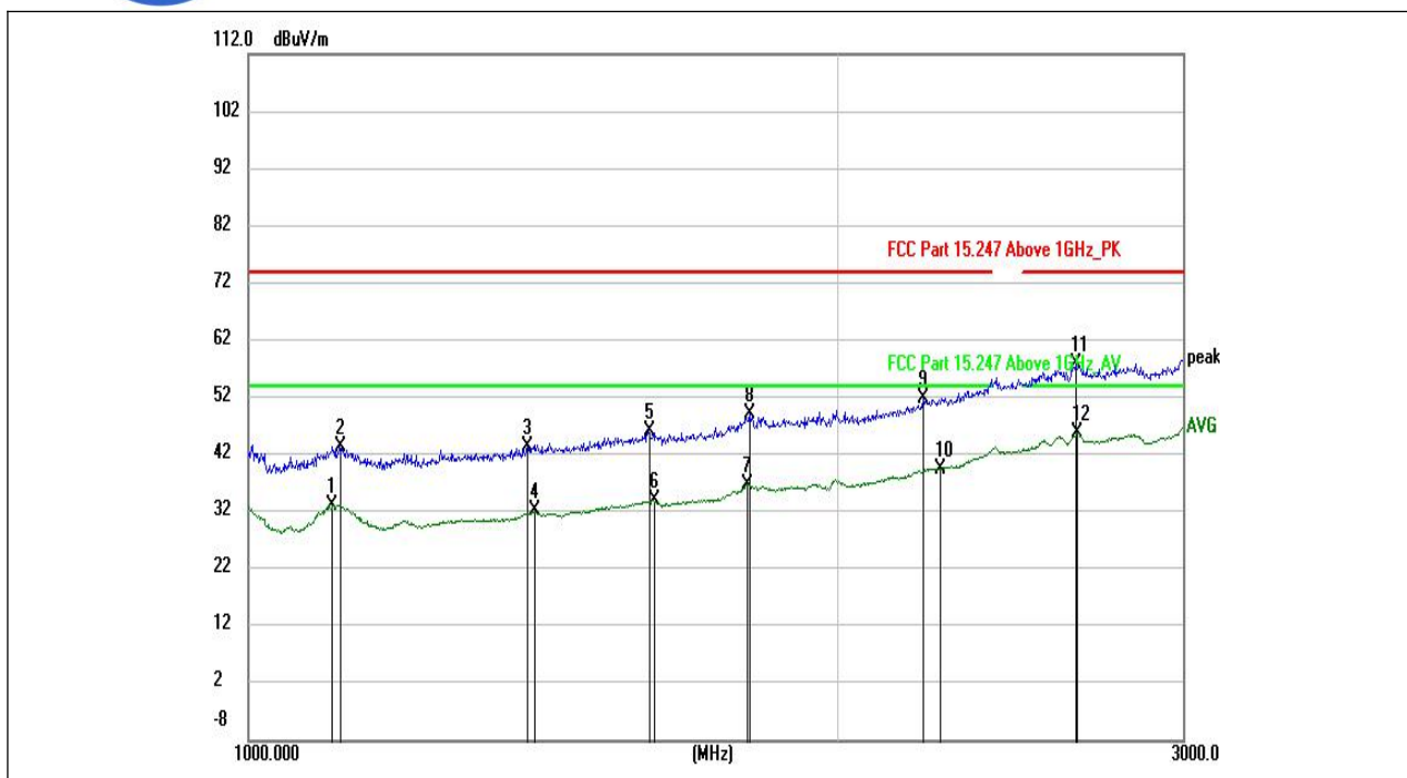
(802.11g _2467MHz, Antenna Horizontal, 1GHz to 3GHz)
