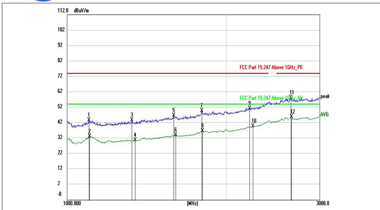
(802.11n_20M_2472MHz, Antenna Horizontal, 1GHz to 3GHz)
