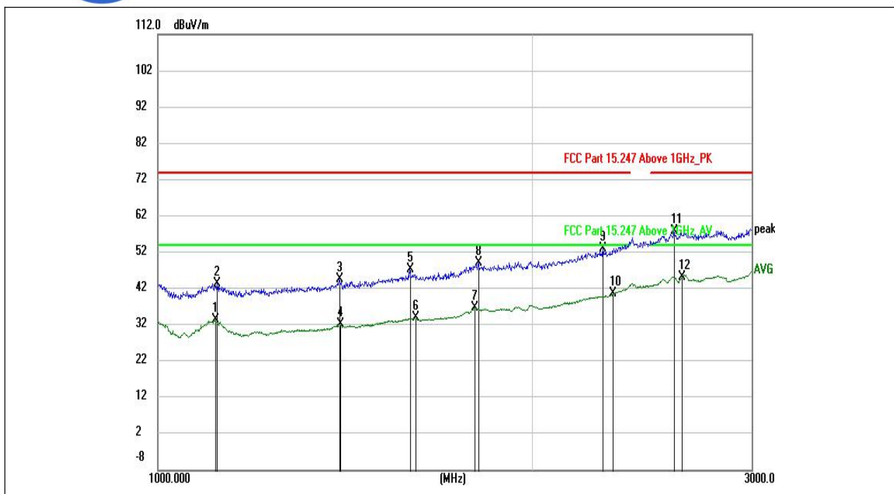
(802.11b _2472MHz, Antenna Horizontal, 1GHz to 3GHz)
