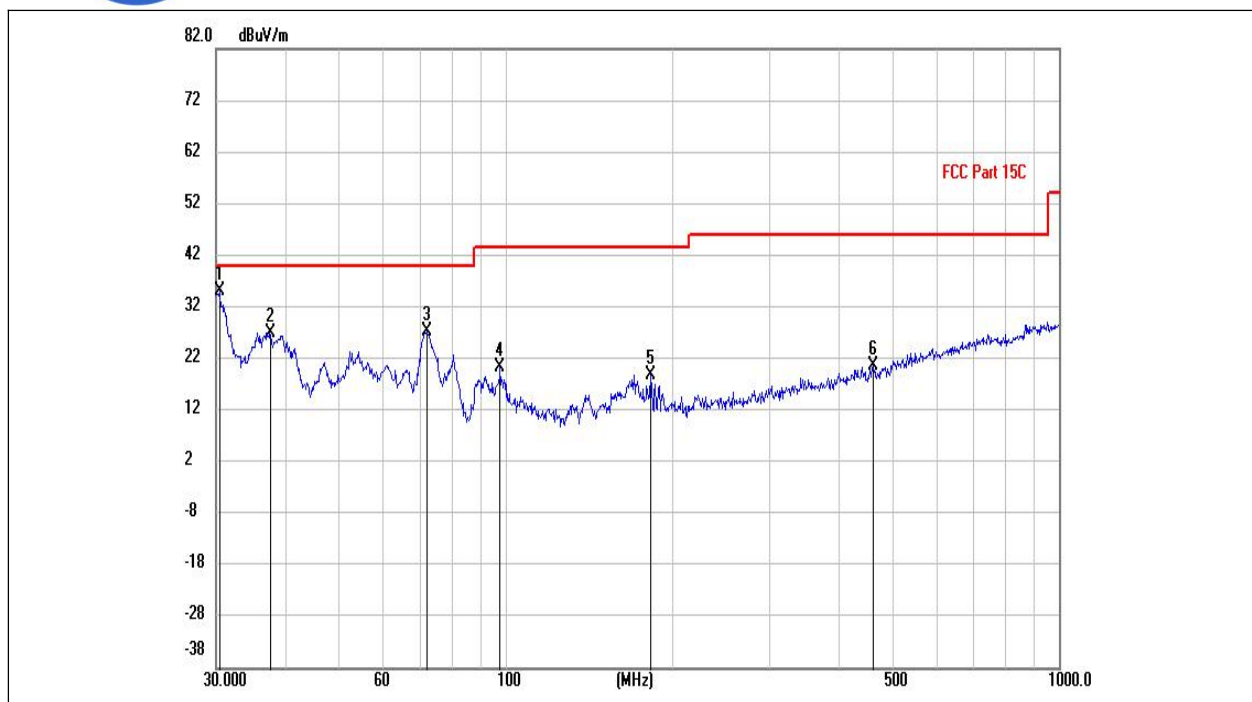
(802.11g _2472MHz, Antenna Vertical, 30MHz to 1GHz)
