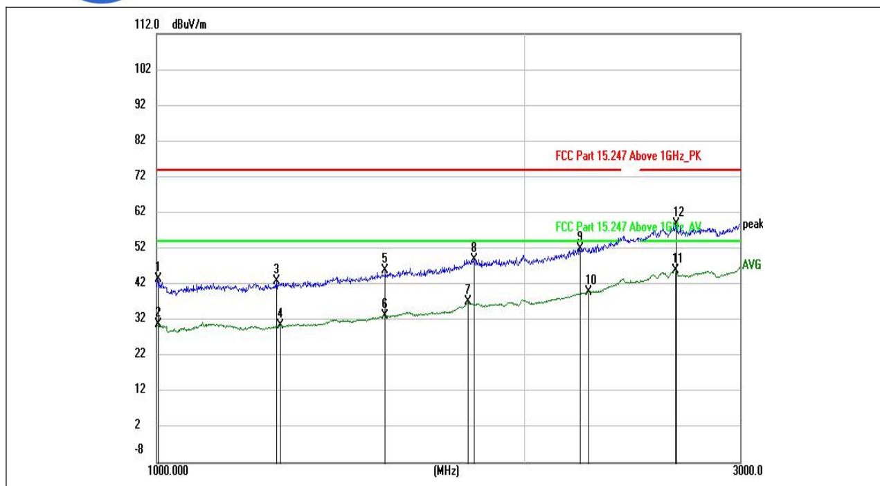
(802.11n_20M_2472MHz, Antenna Vertical , 1GHz to 3GHz)
