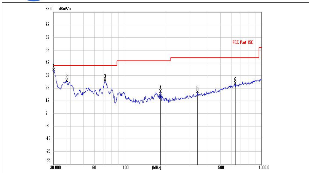
(802.11g _2437MHz, Antenna Vertical, 30MHz to 1GHz)
