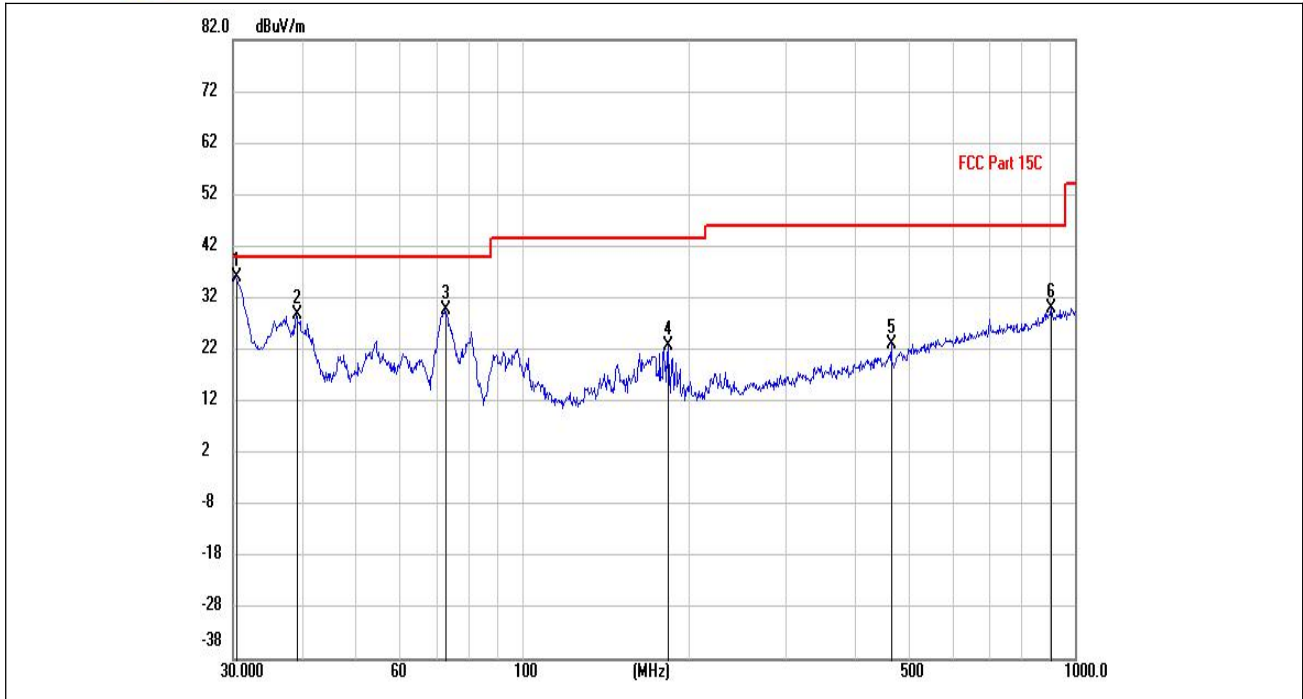
(802.11b_2472MHz, Antenna Vertical, 30MHz to 1GHz)
