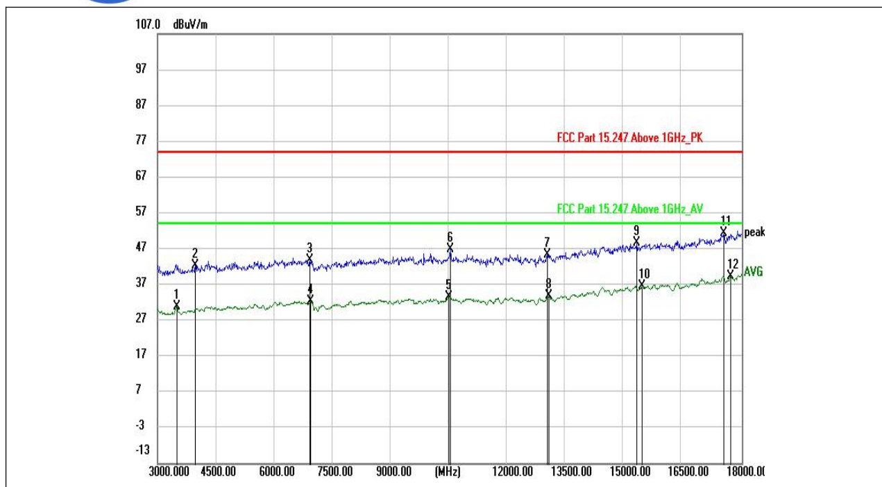
(802.11g _2467MHz, Antenna Horizontal, 3GHz to 18GHz)
