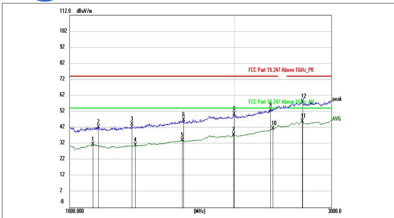
(802.11n_20M_2467MHz, Antenna Vertical , 1GHz to 3GHz)
