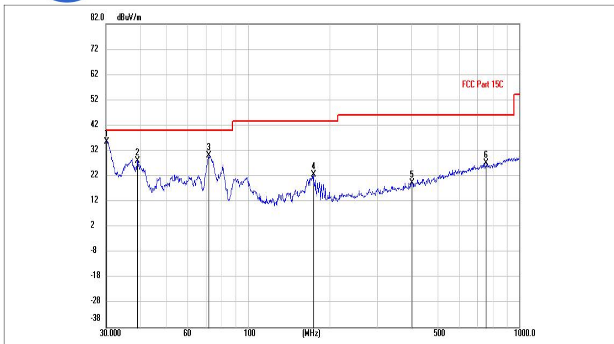
(802.11b_2467MHz, Antenna Vertical, 30MHz to 1GHz)
