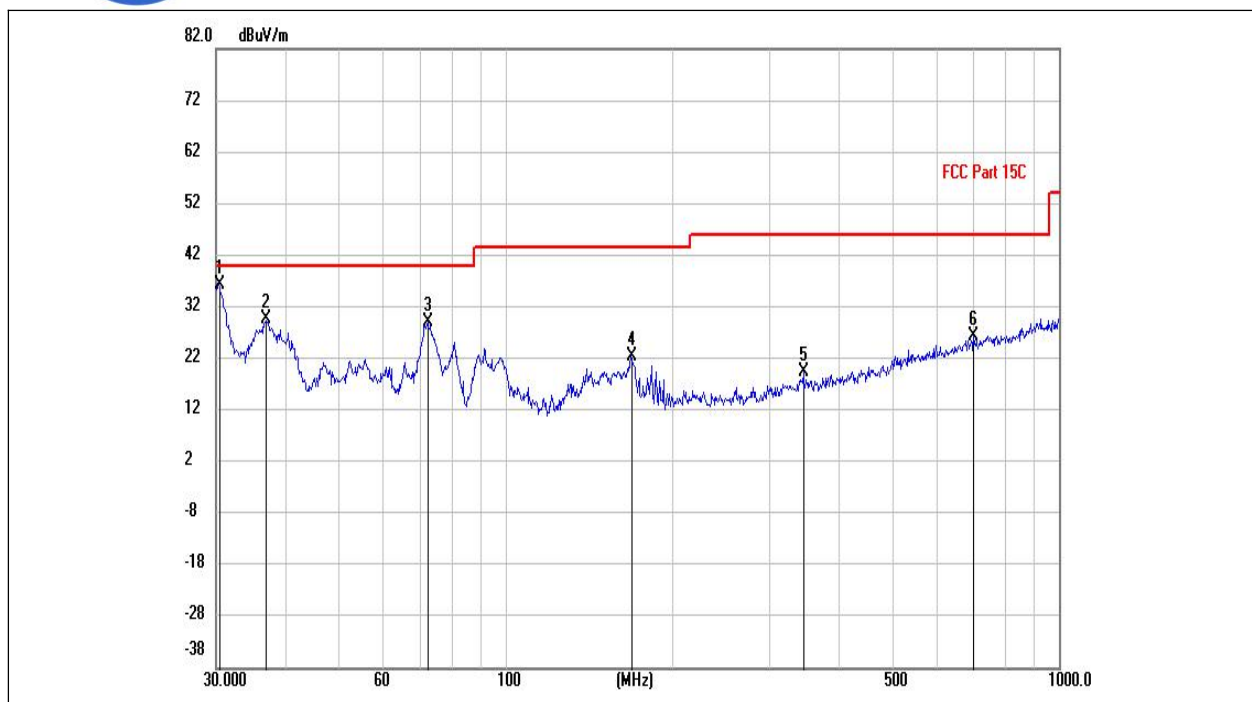
(802.11n_20M_2437MHz, Antenna Vertical, 30MHz to 1GHz)
