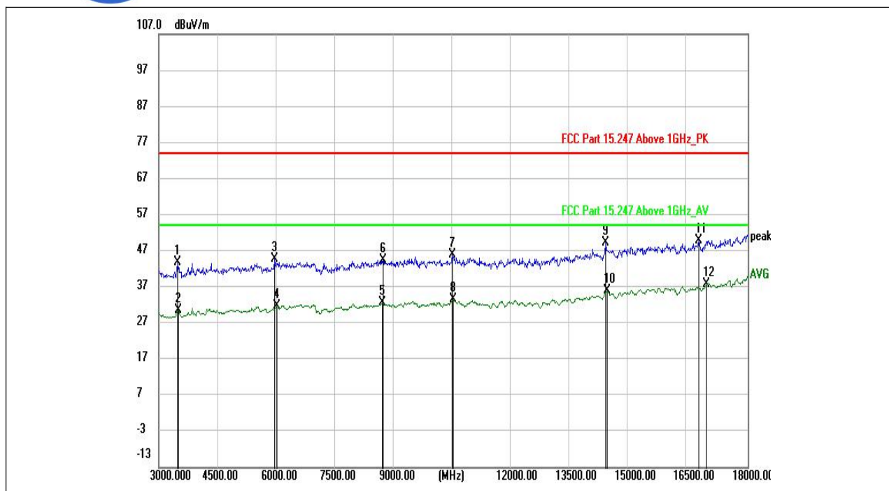
(802.11n_20M_2472MHz, Antenna Horizontal, 3GHz to 18GHz)
