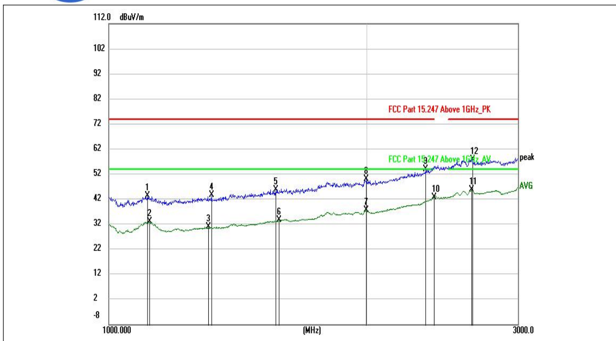
(802.11b _2467MHz, Antenna Horizontal, 1GHz to 3GHz)
