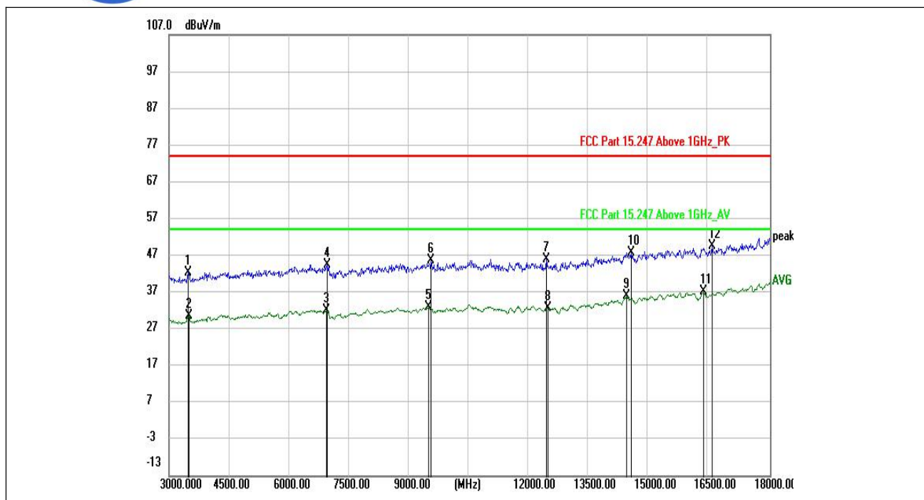
(802.11n_20M_2462MHz, Antenna Horizontal, 3GHz to 18GHz)
