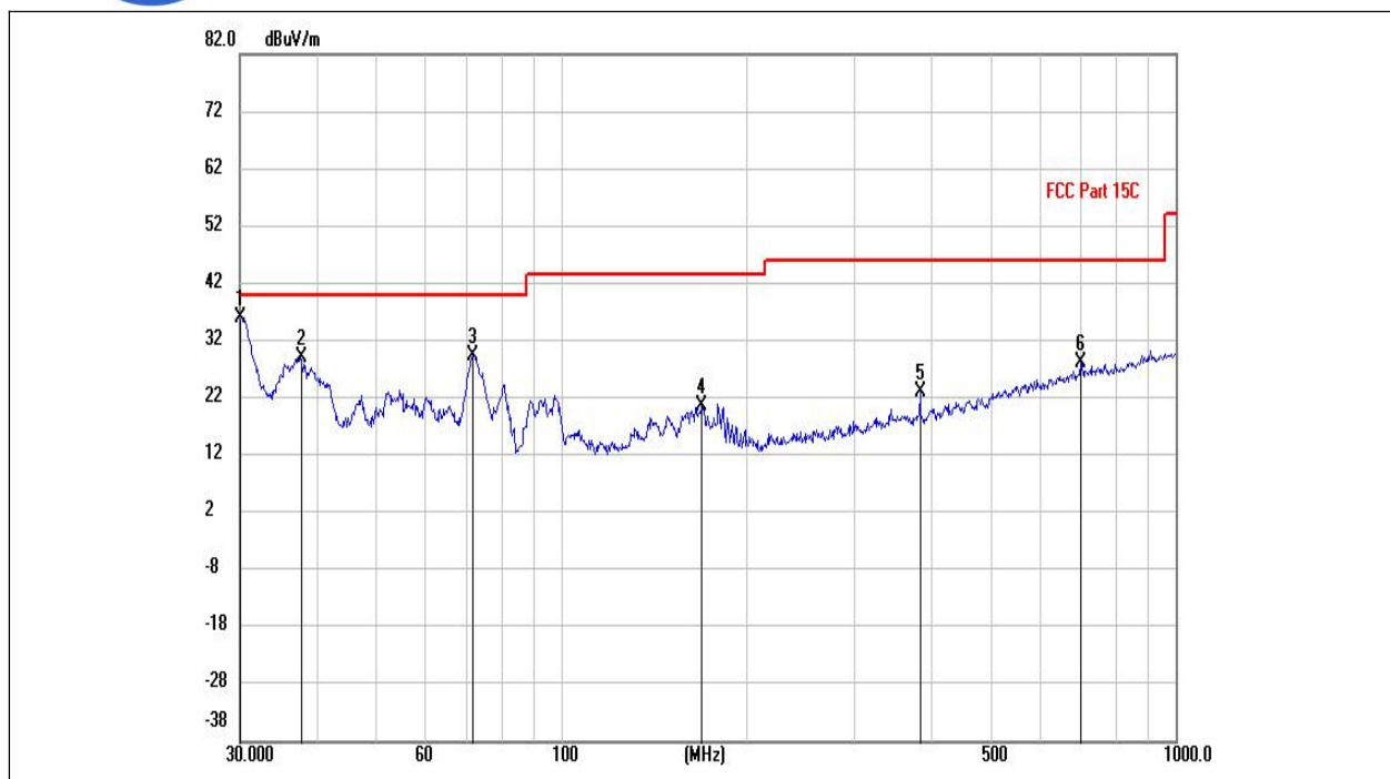
(802.11n_20M_2467MHz, Antenna Vertical, 30MHz to 1GHz)
