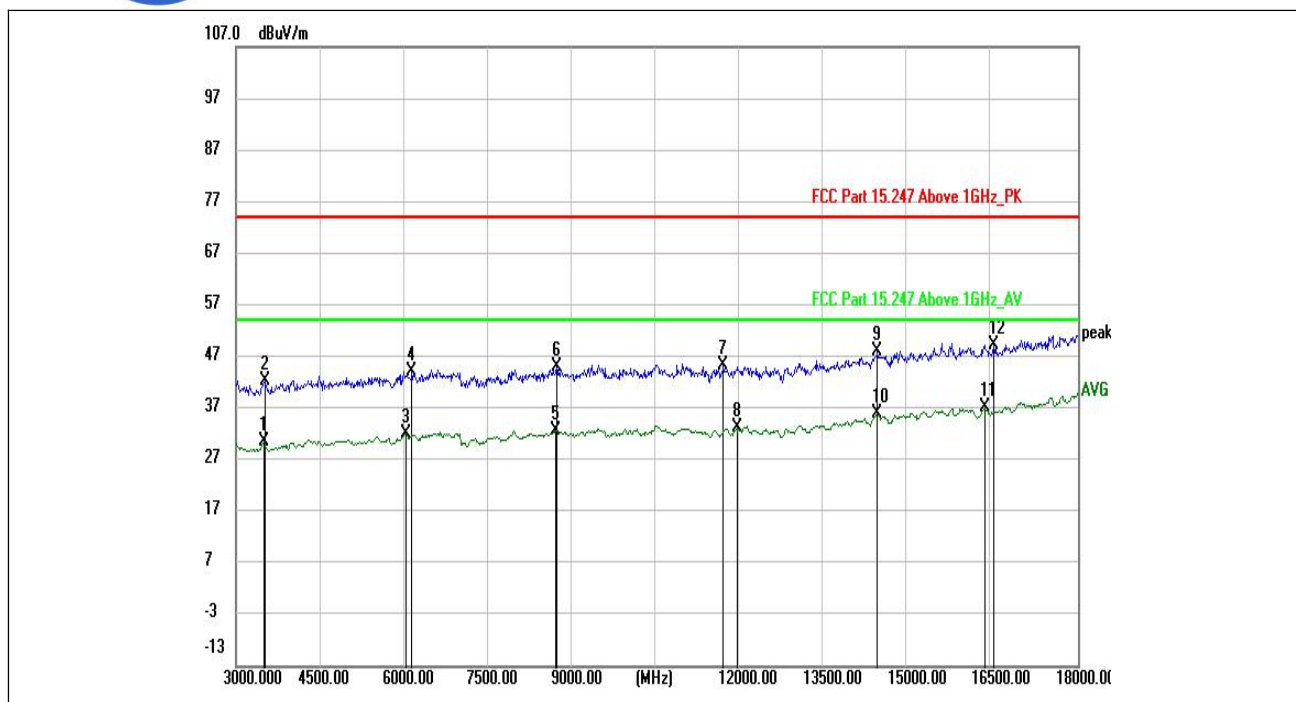
(802.11g _2472MHz, Antenna Vertical, 3GHz to 18GHz)
