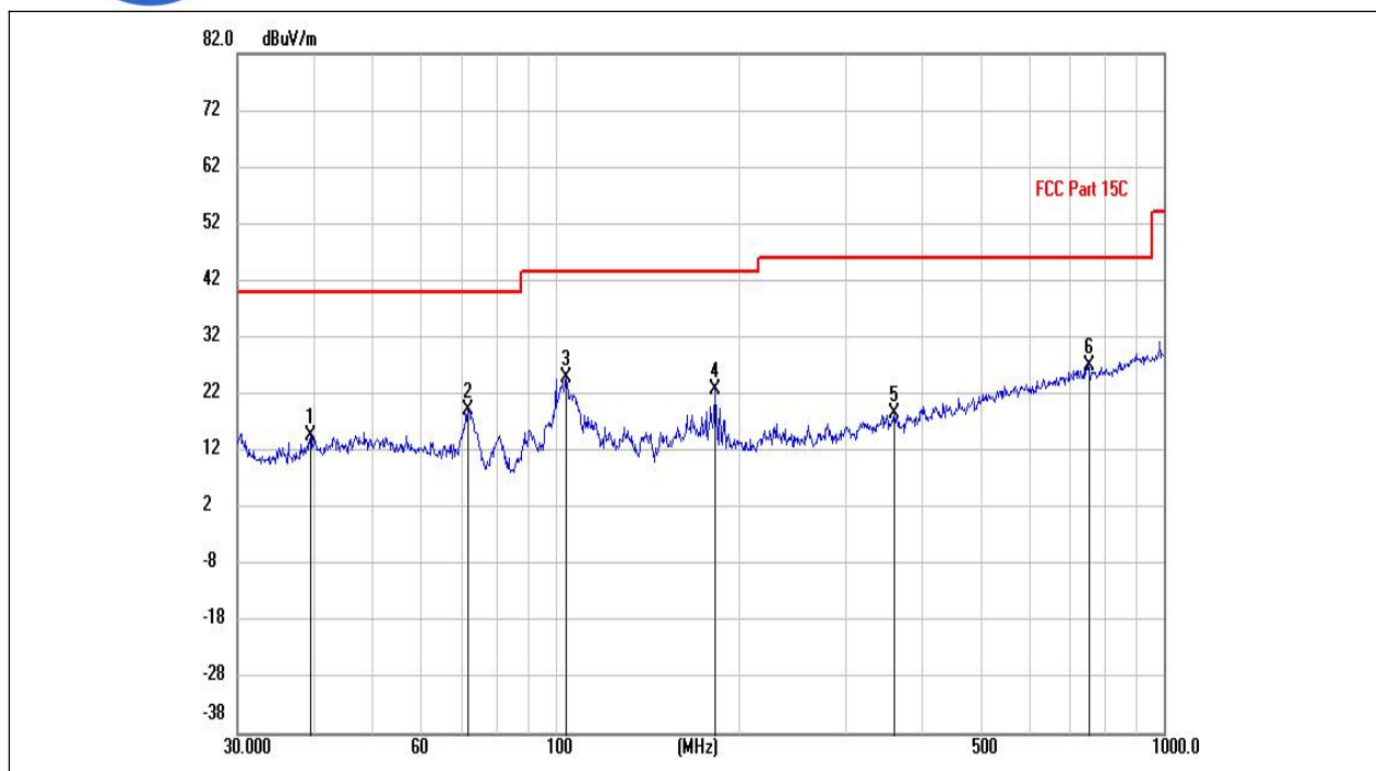
(802.11g _2472MHz, Antenna Horizontal, 30MHz to 1GHz)
