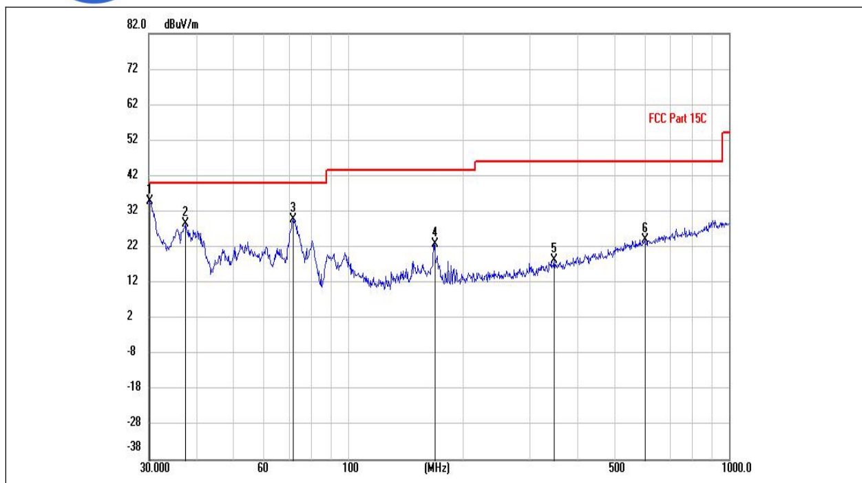
(802.11n_20M_2472MHz, Antenna Vertical, 30MHz to 1GHz)
