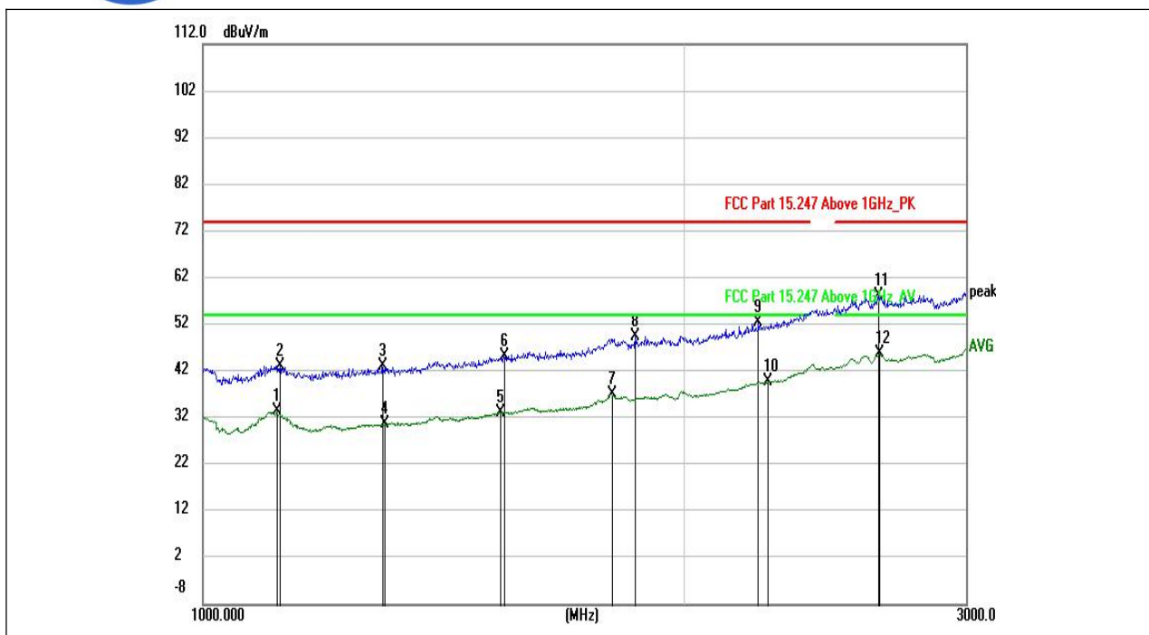
(802.11g _2472MHz, Antenna Horizontal, 1GHz to 3GHz)
