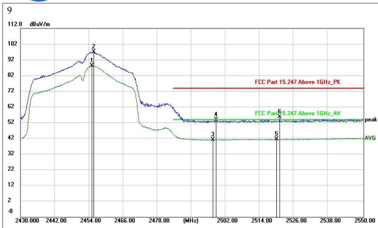
(802.11n_40M _2452MHz, Antenna Horizontal)
