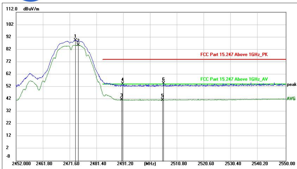
(802.11b_2472MHz, Antenna Vertical)
