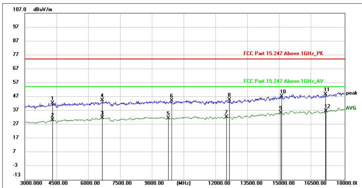
(GFSK_2480MHz, Antenna Horizontal, 3GHz to 18GHz)
