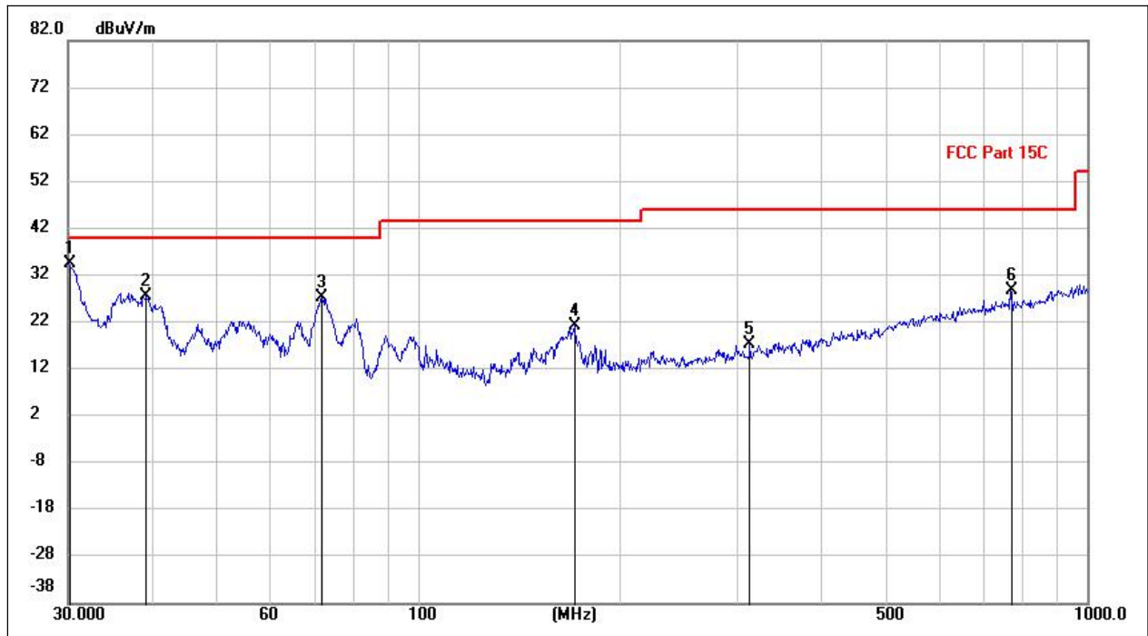
(π/4-DQPSK_2440MHz, Antenna Vertical, 30MHz to 1GHz)
