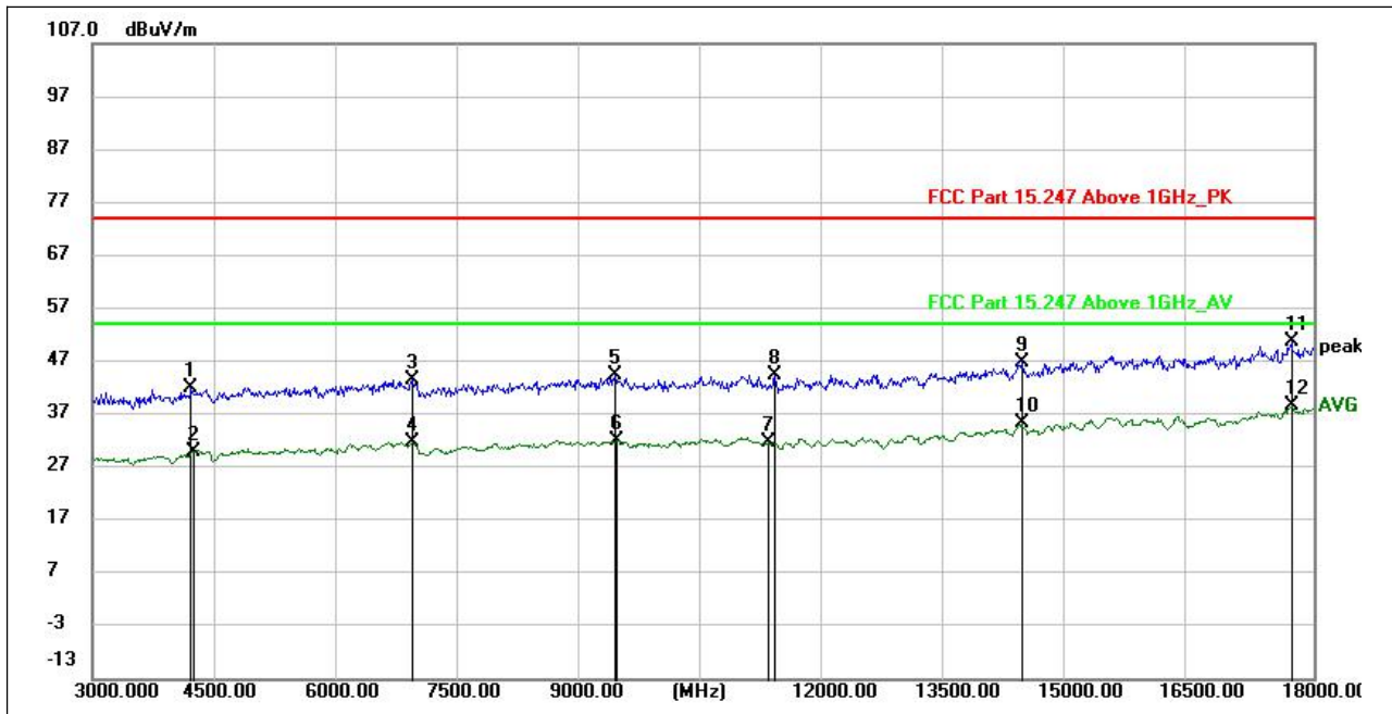
( \pi/4 -DQPSK _2402MHz, Antenna Vertical, 3GHz to 18GHz)
