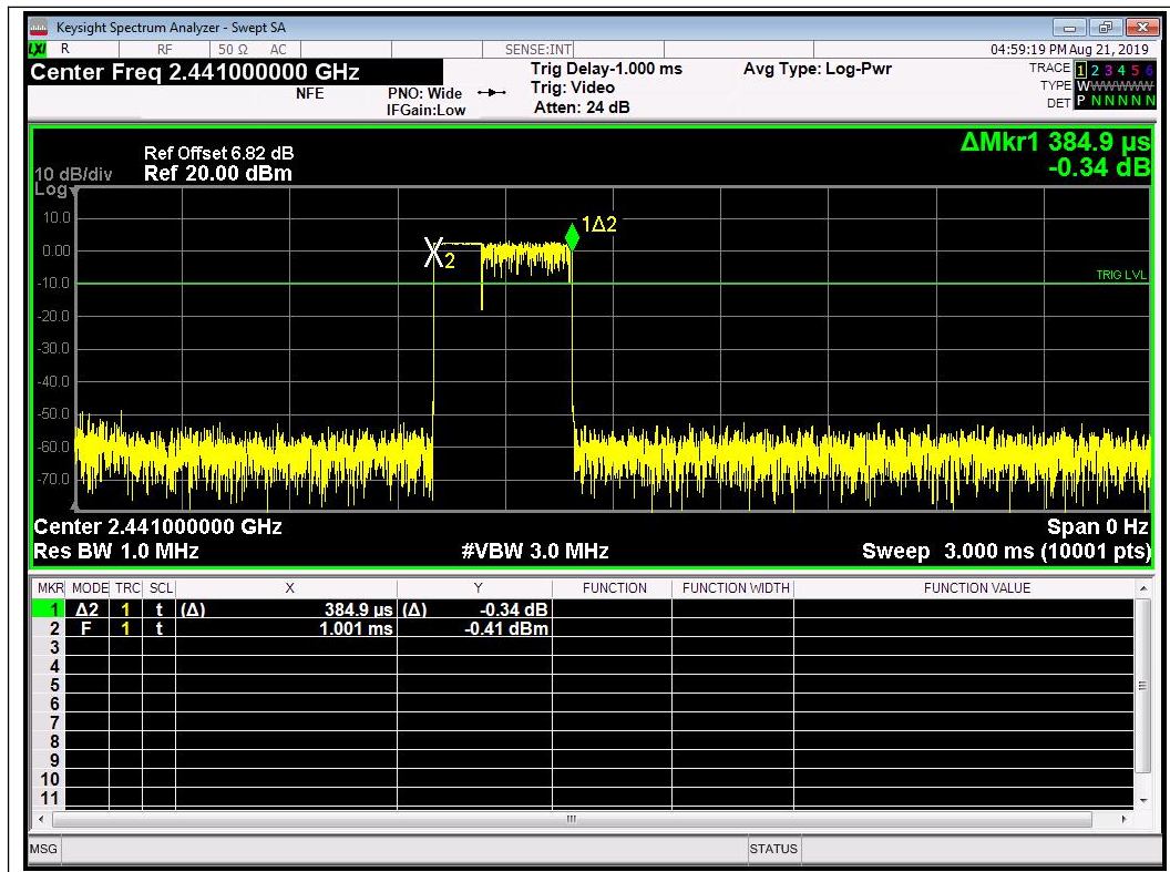
(3DH1_2441M, 8-DQPSK)
