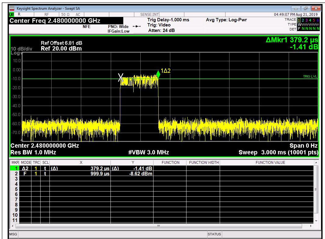
(2DH1_2480M, \pi/4 -DQPSK)
