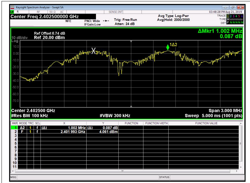
(GFSK, Channel 0 and 1, 2402MHz)
