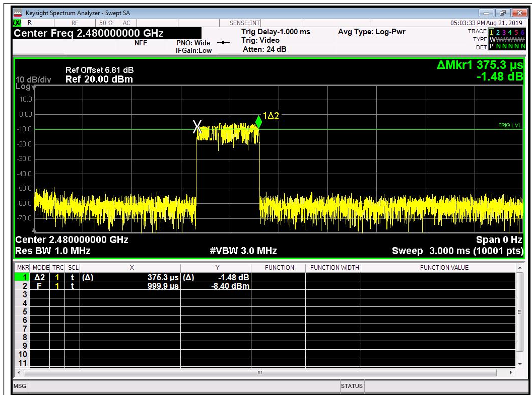
(3DH1_2480M, 8-DQPSK)
