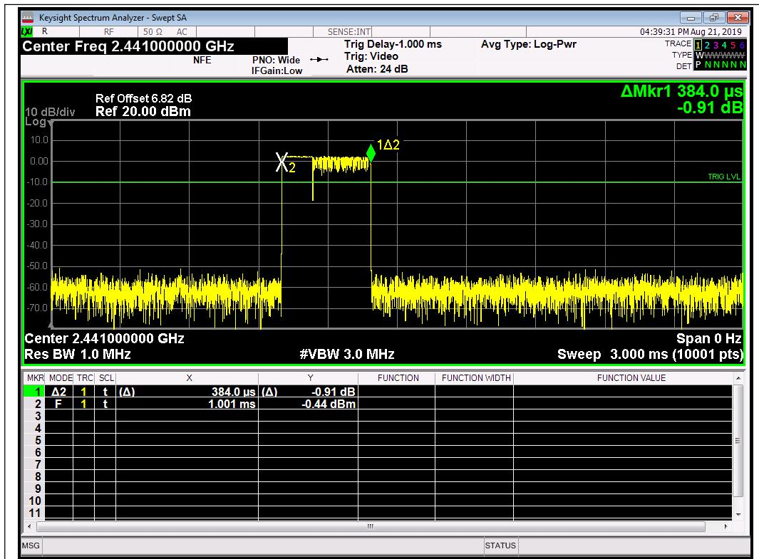
(2DH1_2441M, \pi/4 -DQPSK)
