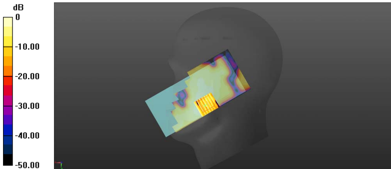
0 dB = 0.0472 W/kg
