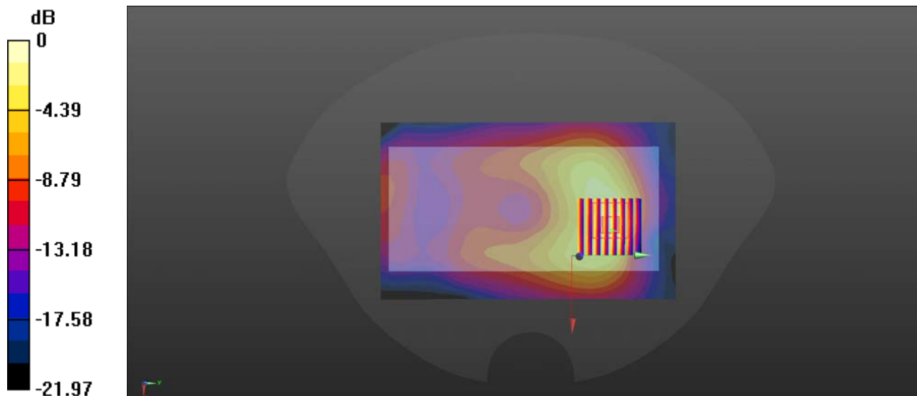
0 dB = 0.634 W/kg
