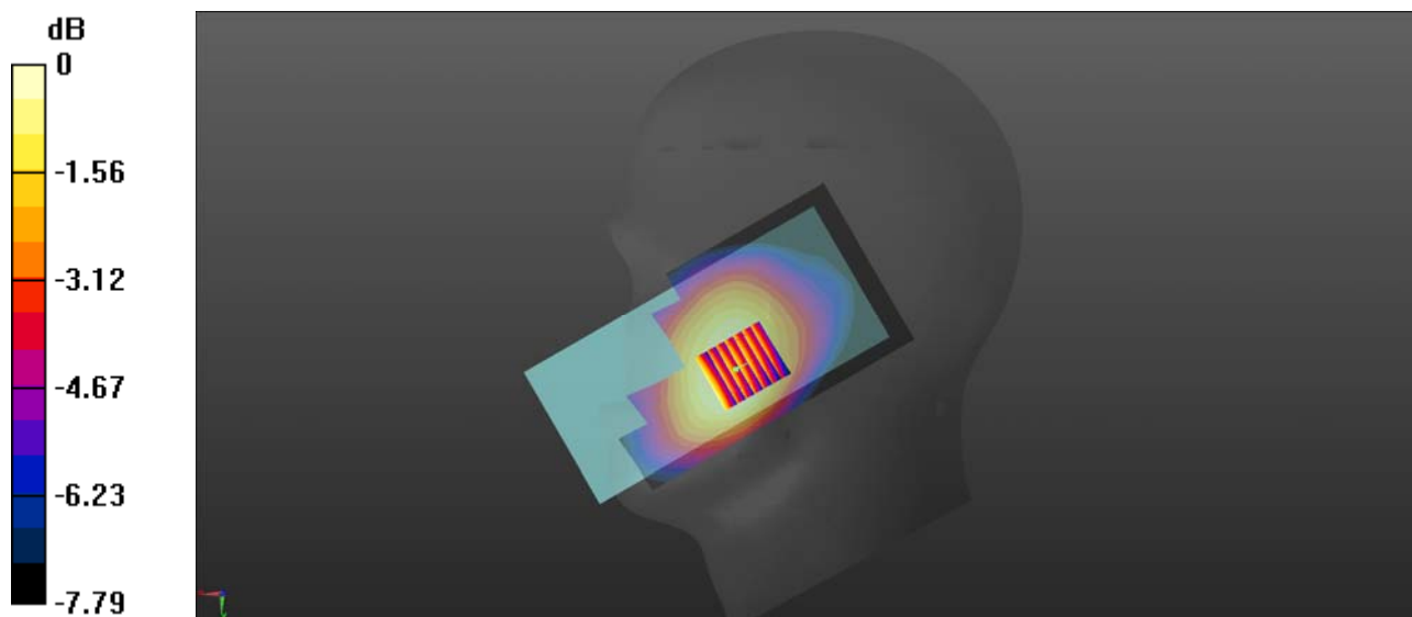
0 dB = 0.182 W/kg
