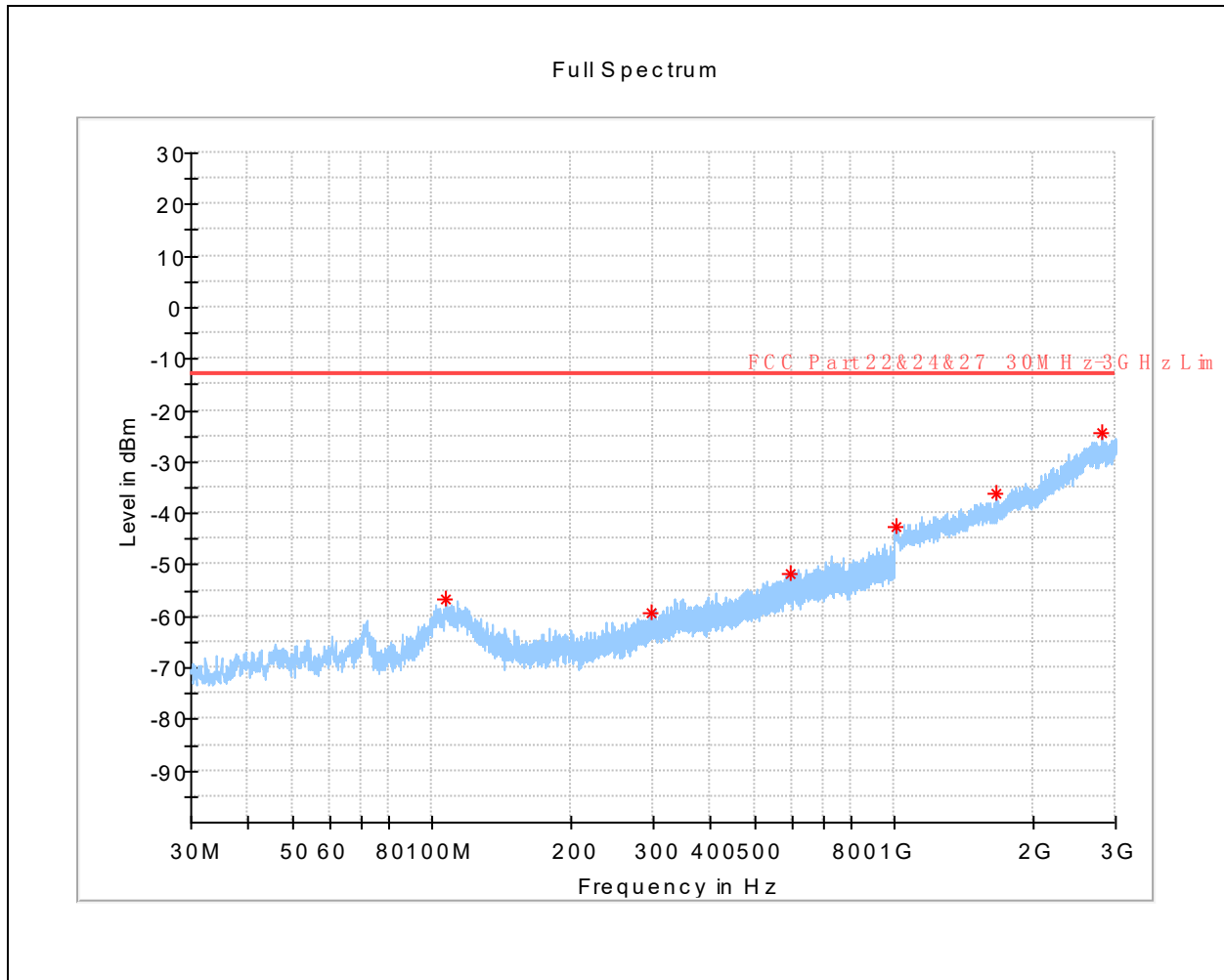
(LTE Band 41 _ QPSK_ High Channel _ 30MHz to 3GHz _ Vertical)
