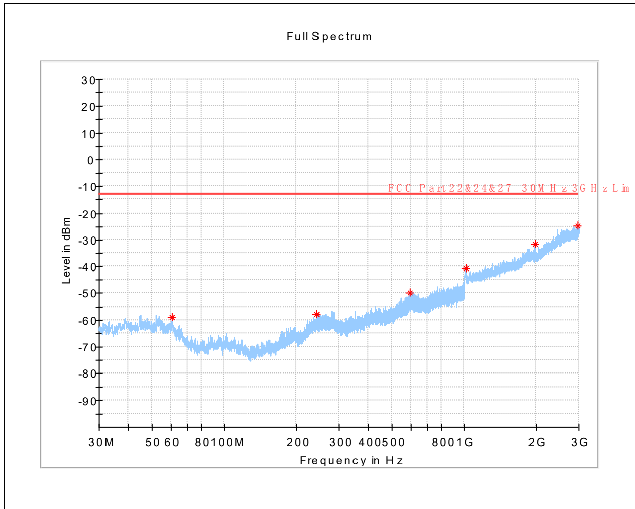
(LTE Band 25_QPSK_High Channel_30MHz to 3GHz_Horizontal)
