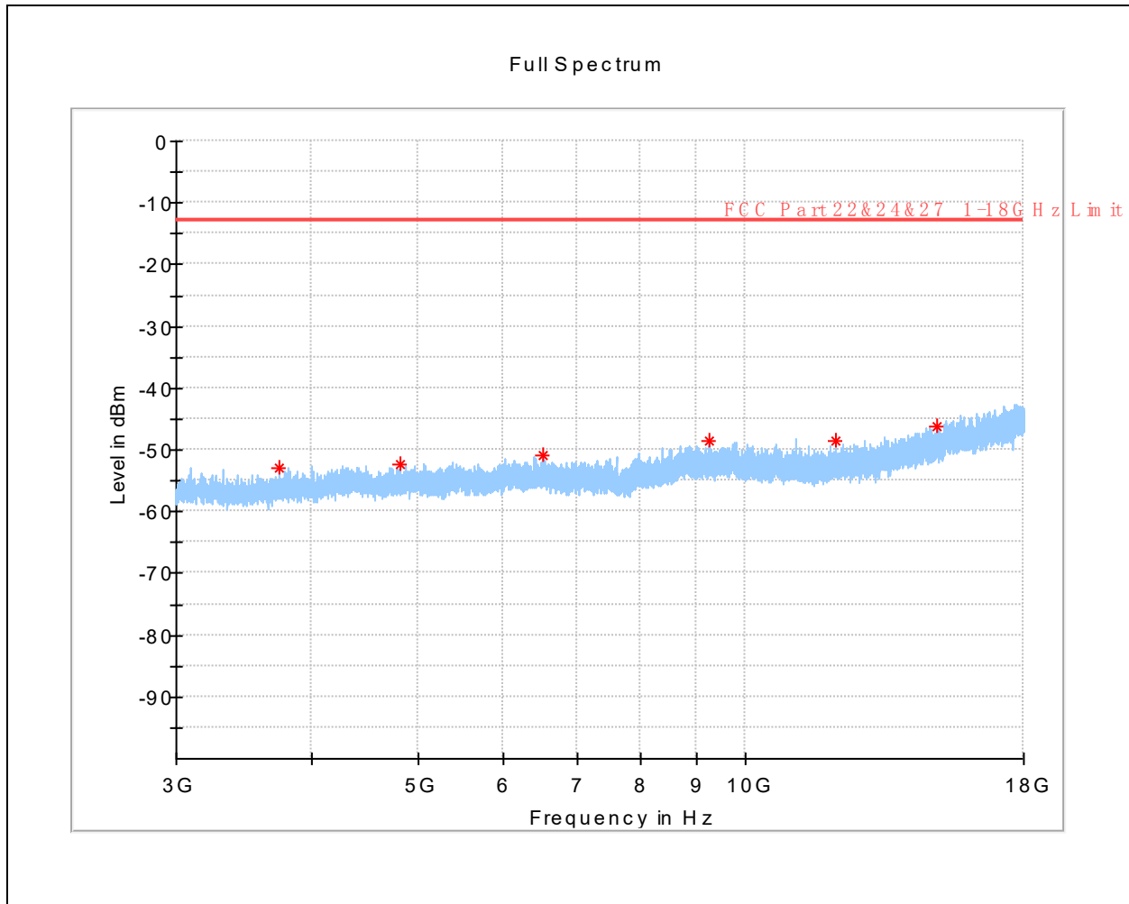
(LTE Band 25_QPSK_Middle Channel_3GHz to 18GHz_Horizontal)
