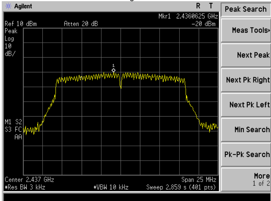
Mode :TX 11g middle channel
