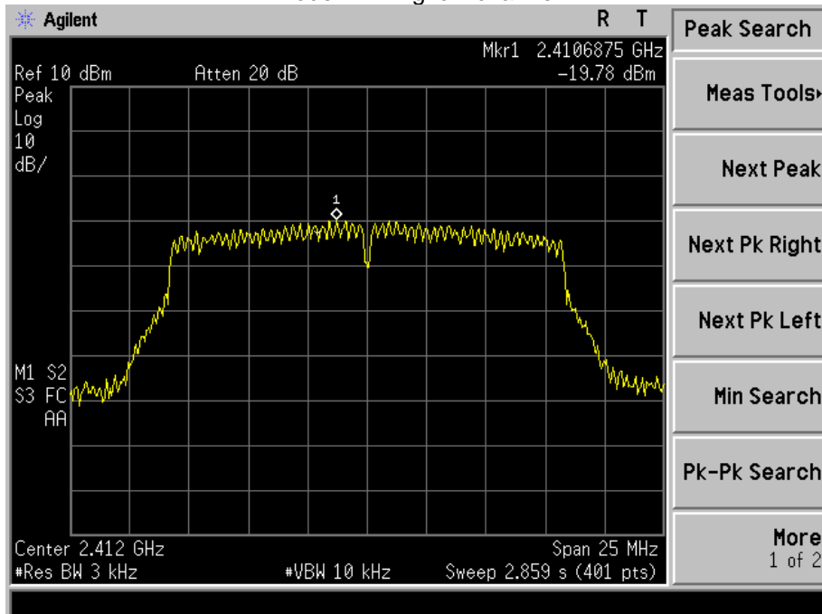
Mode :TX 11g low channel
