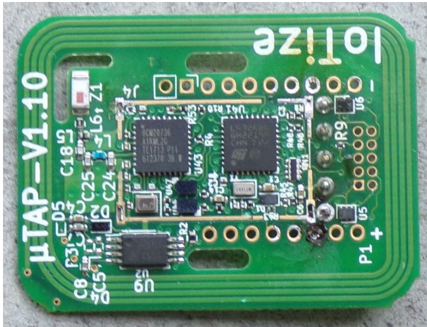
Shield removed
