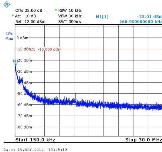
Figure 24 Frequency Operation 469.9875MHz, 0.15-30MHz band
