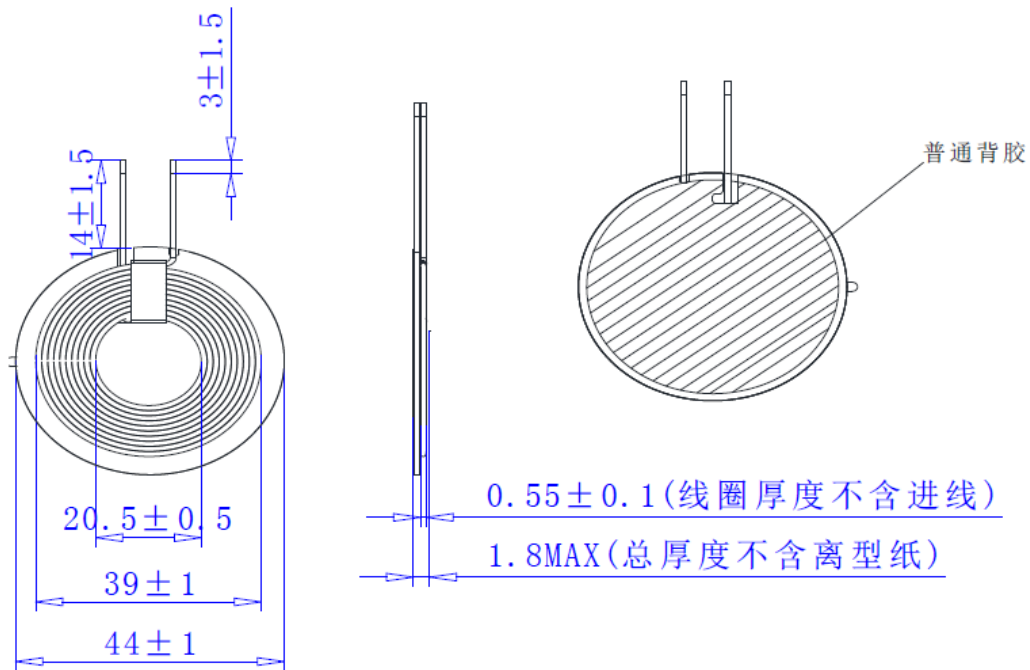
Phone Coil Antenna& Airpods Coil Antenna:
