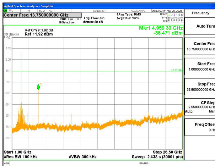
3DH1_Ant1_2402_0~Reference
