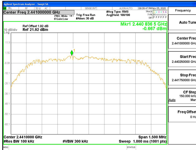
2DH1_Ant1_2441_30~100
