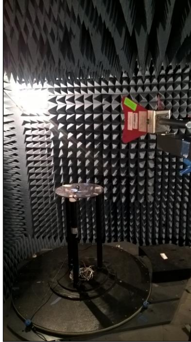
Photograph 1. Radiated Spurious Emissions, Test Setup 1: Above 1 GHz
