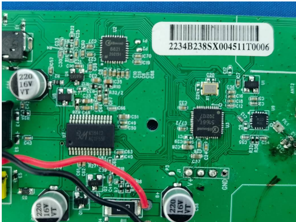
DHP380R/ ADH300 OPEN VIEW OF EUT (FIGURE 1)
