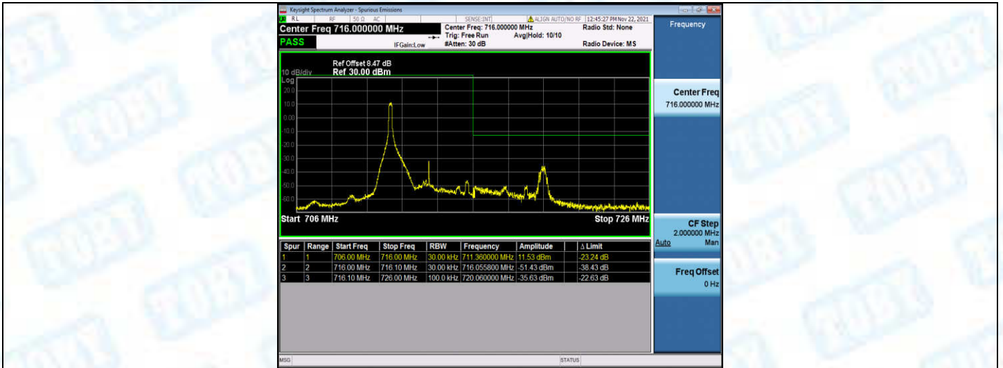
Band12-5MHz-16QAM-23155-1RB#24
