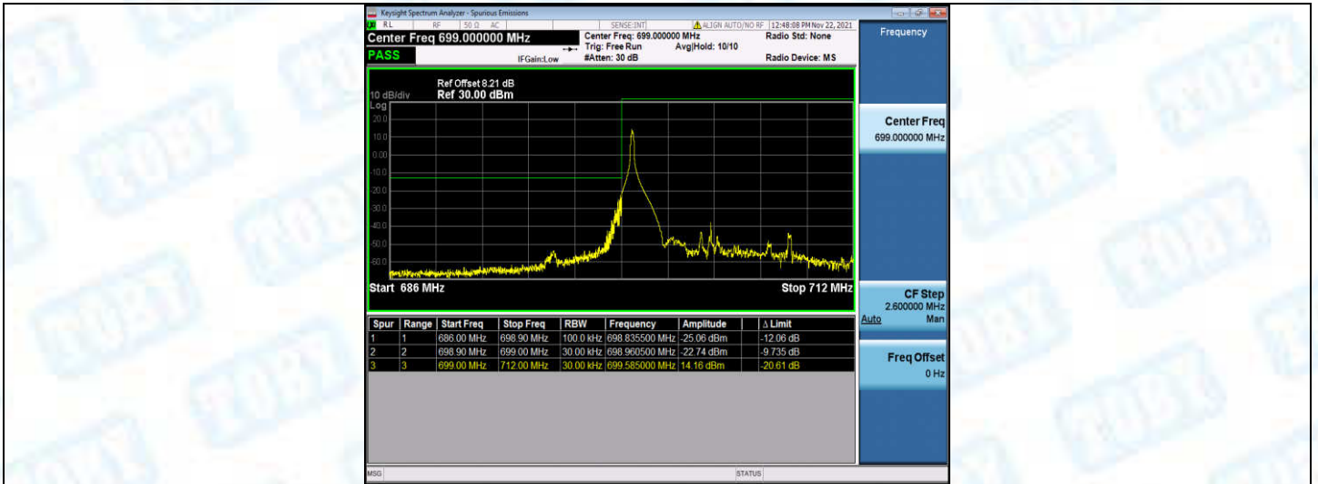
Band12-10MHz-16QAM-23060-1RB#49
