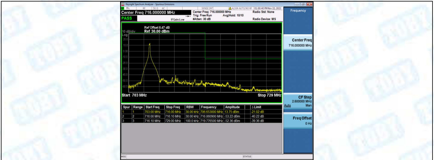
Band17-10MHz-16QAM-23800-1RB#49
