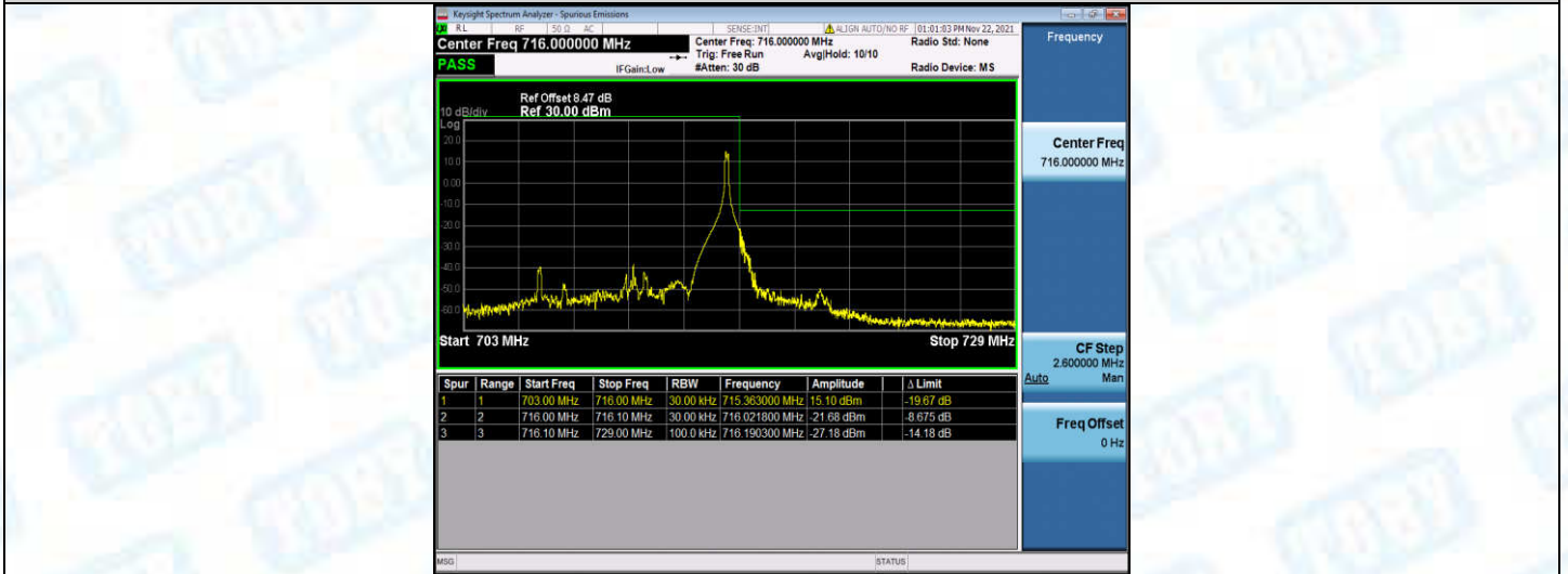
Band17-10MHz-QPSK-23800-50RB#0
