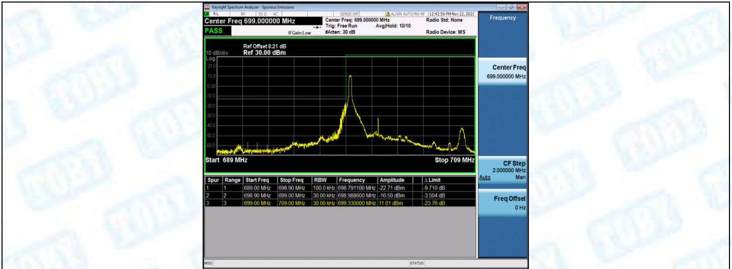
Band12-5MHz-16QAM-23035-1RB#24
