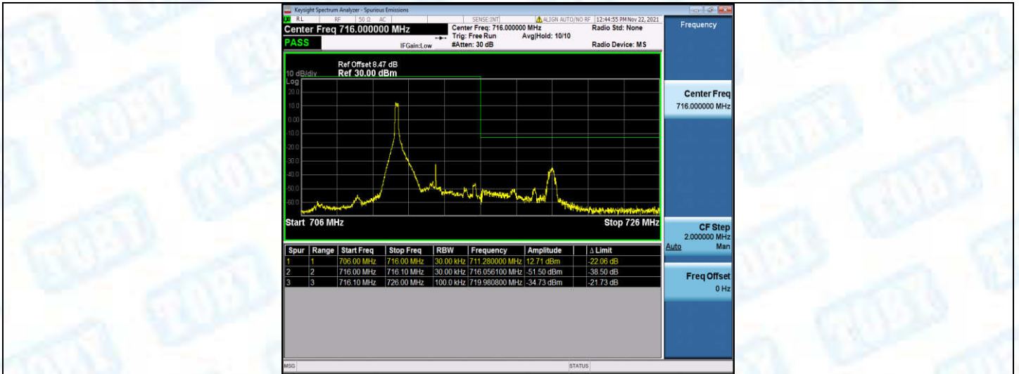
Band12-5MHz-QPSK-23155-1RB#24
