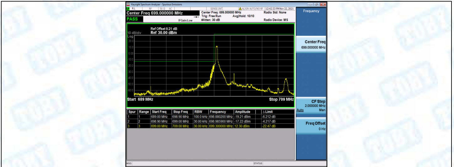
Band12-5MHz-QPSK-23035-1RB#24
