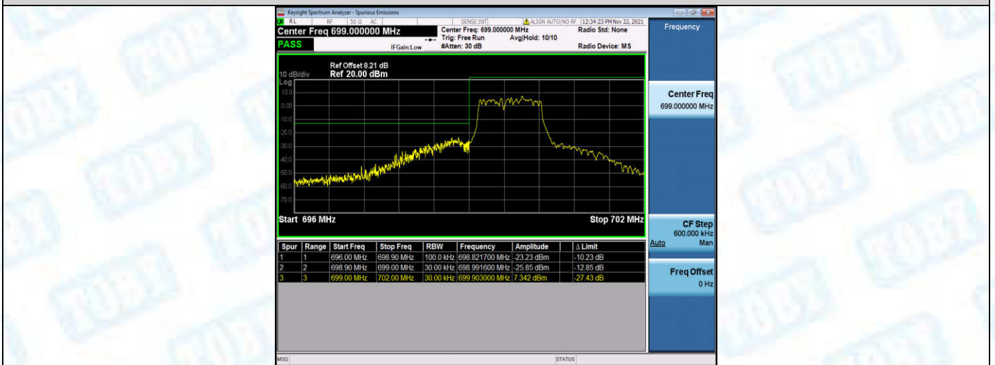
Band12-1.4MHz-16QAM-23173-1RB#0
