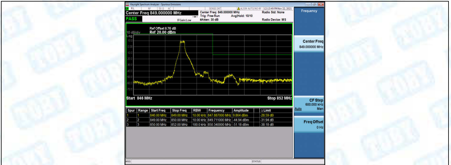
Band5-1.4MHz-16QAM-20643-1RB#5
