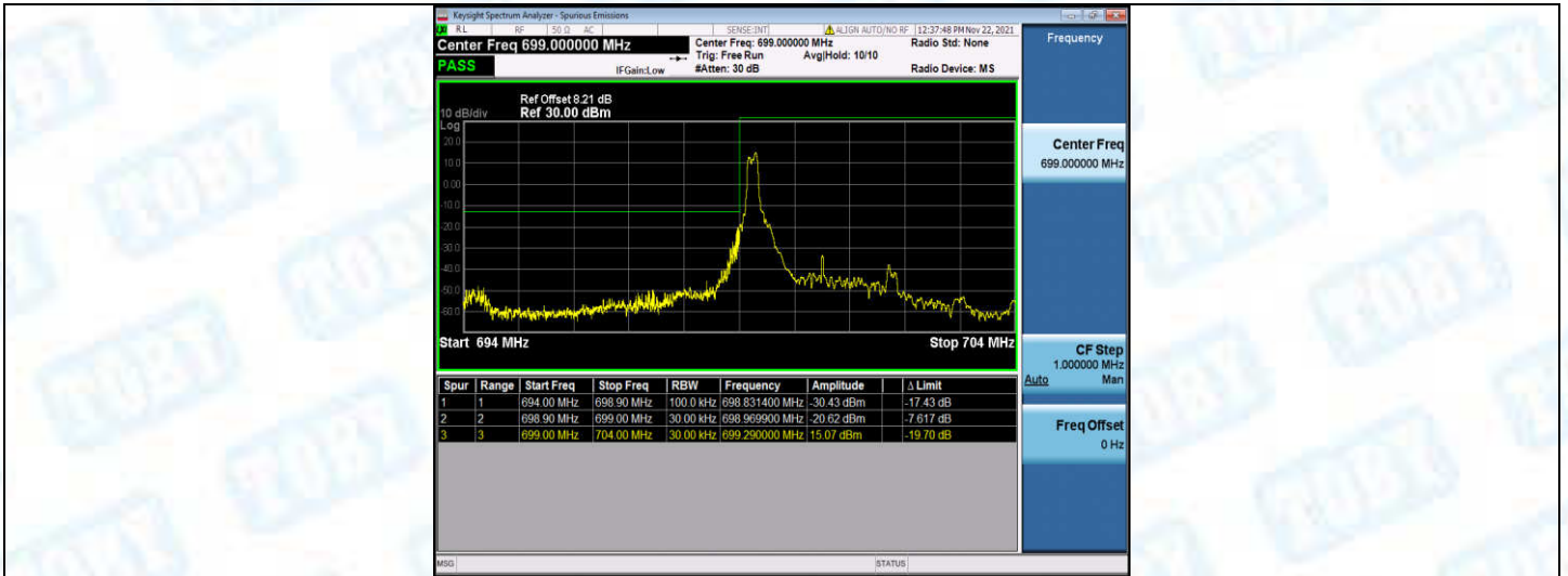
Band12-3MHz-16QAM-23025-1RB#14
