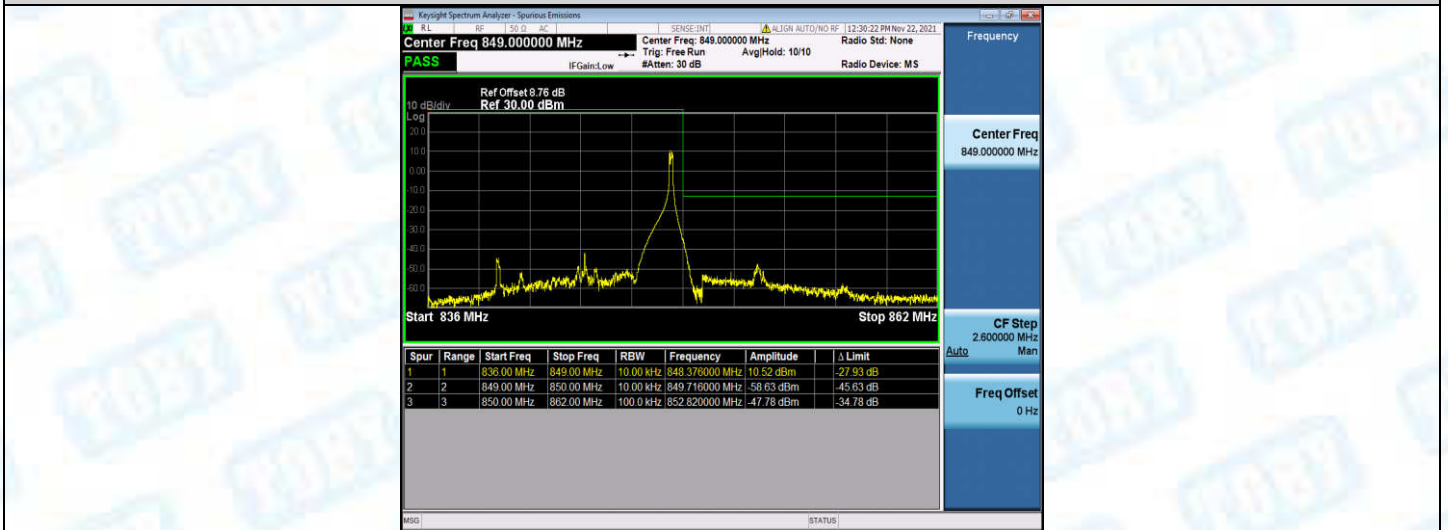
Band5-10MHz-QPSK-20600-50RB#0
