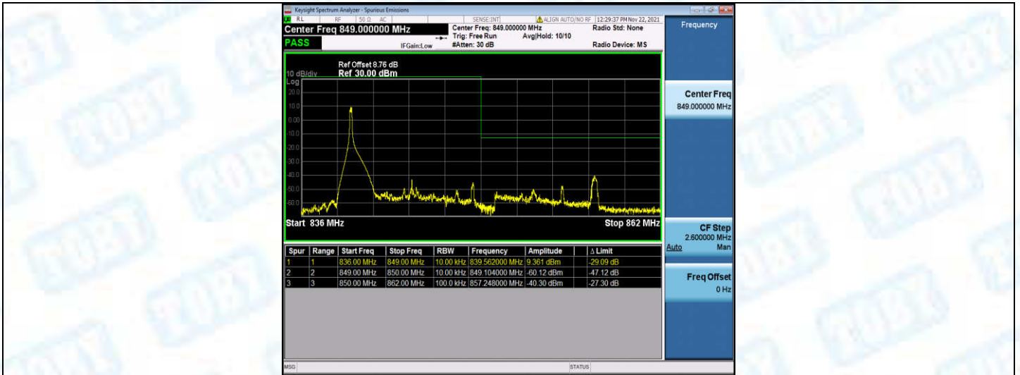
Band5-10MHz-QPSK-20600-1RB#49
