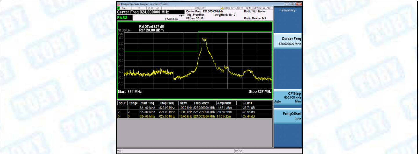
Band5-1.4MHz-16QAM-20407-1RB#5
