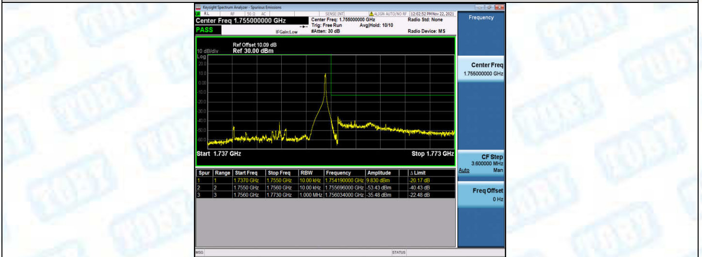
Band4-15MHz-16QAM-20325-75RB#0
