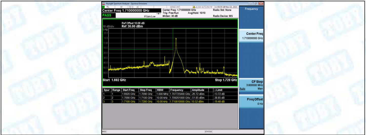
Band4-15MHz-16QAM-20025-1RB#74
