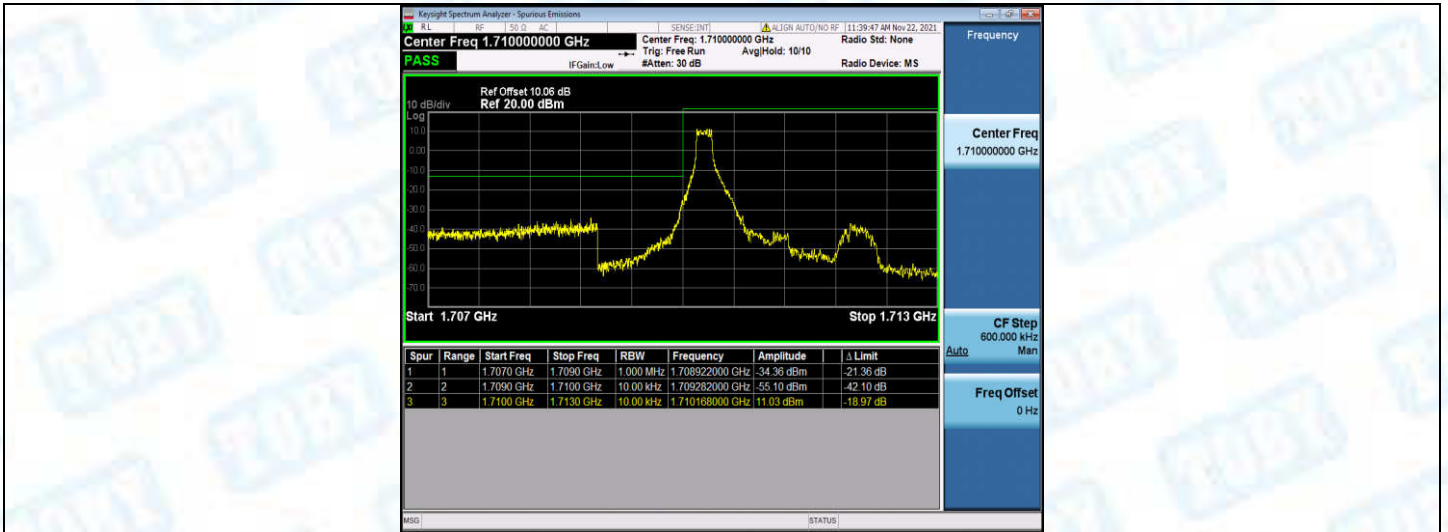
Band4-1.4MHz-16QAM-19957-1RB#5
