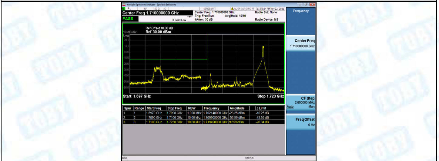
Band4-10MHz-16QAM-20000-50RB#0
