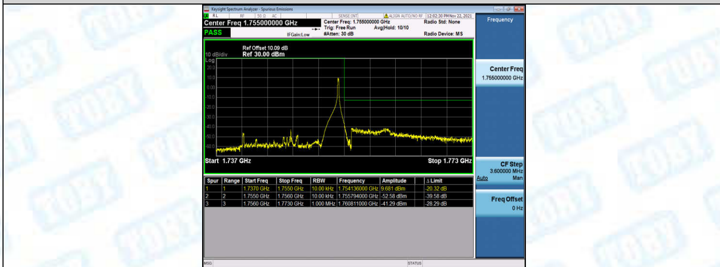
Band4-15MHz-QPSK-20325-75RB#0
