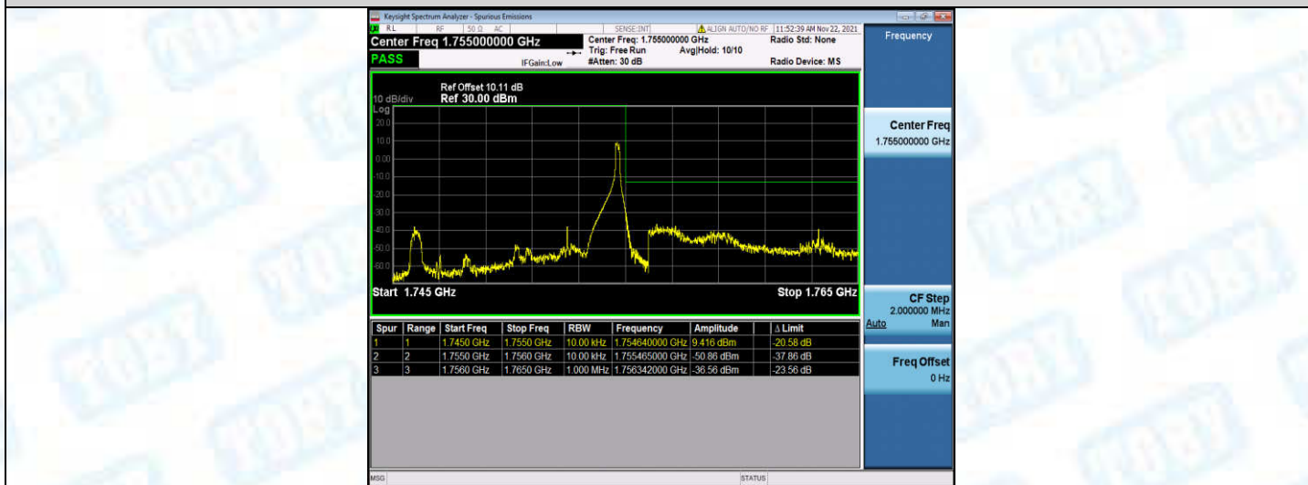
Band4-5MHz-16QAM-20375-25RB#0
