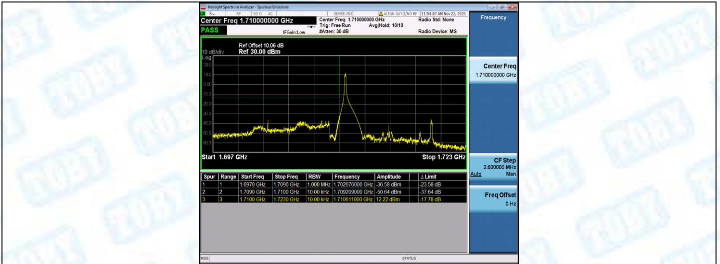
Band4-10MHz-QPSK-20000-1RB#49
