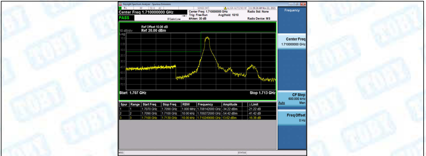
Band4-1.4MHz-QPSK-19957-1RB#5
