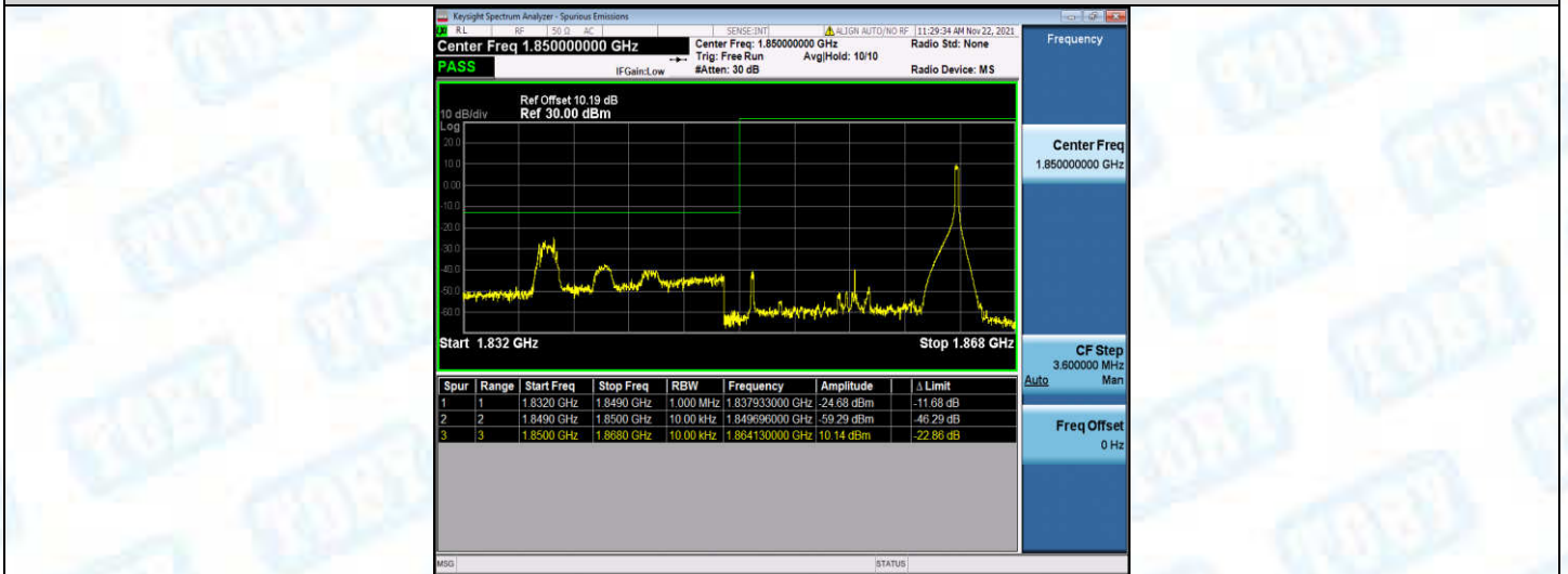
Band2-15MHz-16QAM-18675-75RB#0
