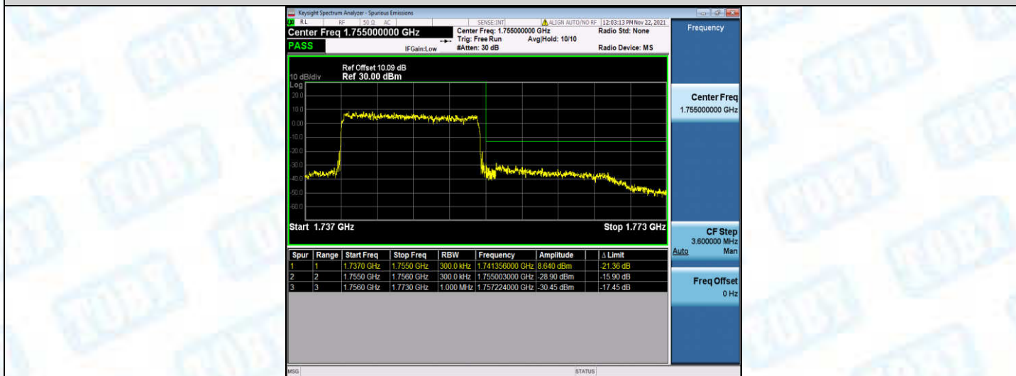
Band4-15MHz-16QAM-20025-1RB#0
