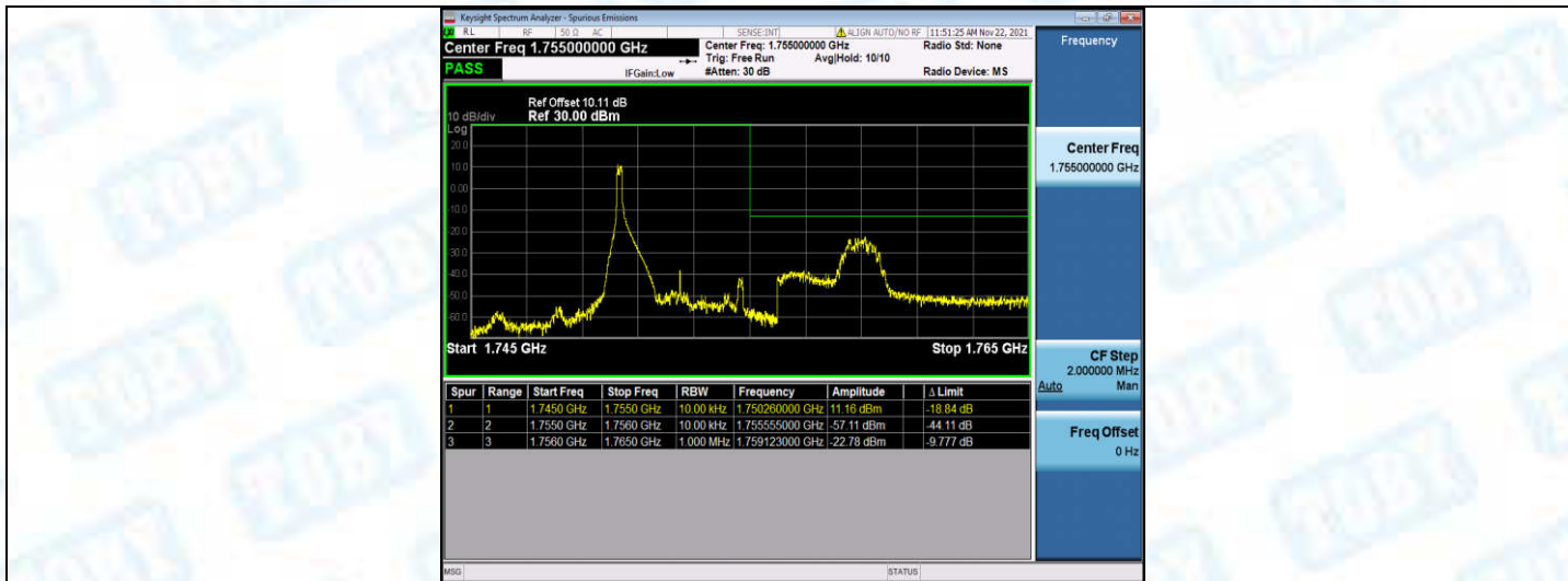
Band4-5MHz-QPSK-20375-1RB#24
