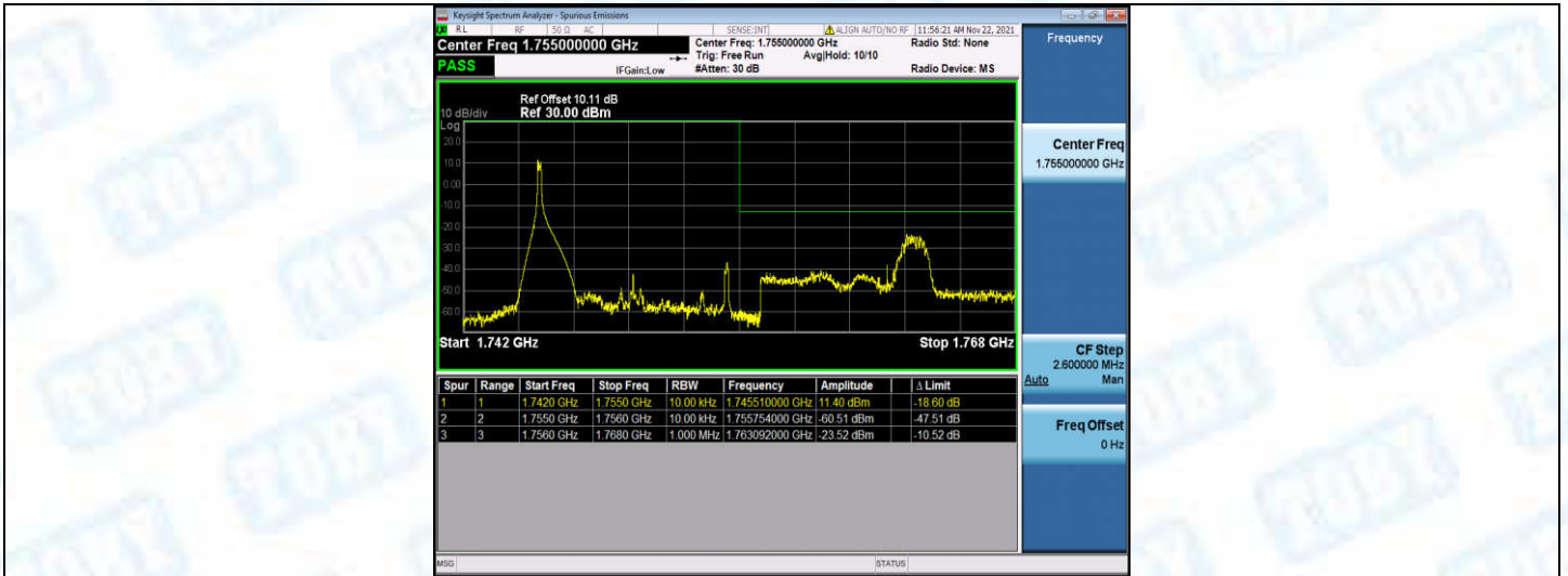
Band4-10MHz-QPSK-20350-1RB#49
