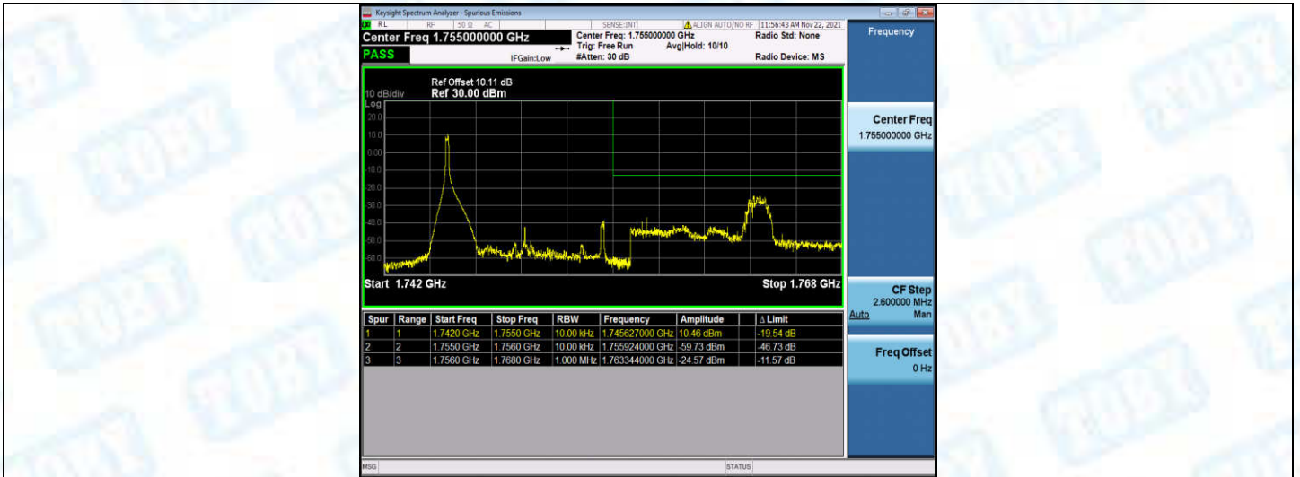
Band4-10MHz-16QAM-20350-1RB#49
